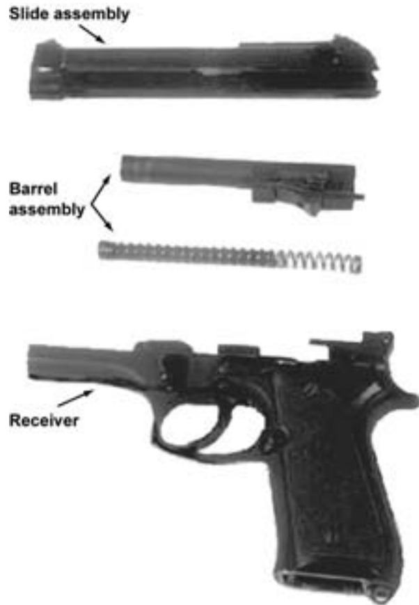
Figure 1-4. Major Components.
