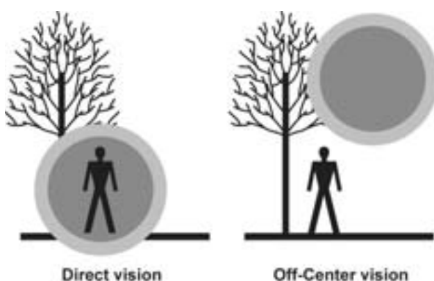
Figure 10-1. Off-Center Vision.
