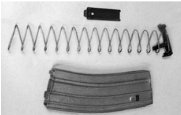
Figure 2-19. Magazine Disassembled.
