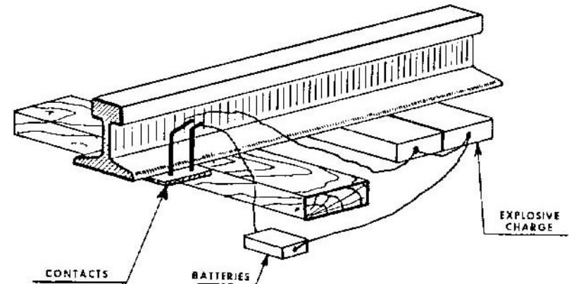
Figure 32 (UNCLASSIFIED). FN wheel-flange firing device (U).
