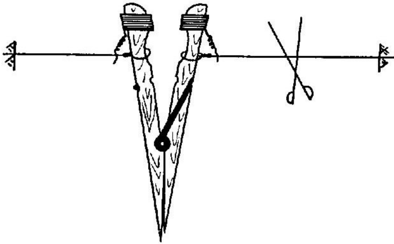
Figure 30 (UNCLASSIFIED). FN clothspine firing device (tension-release-operated) (U).
