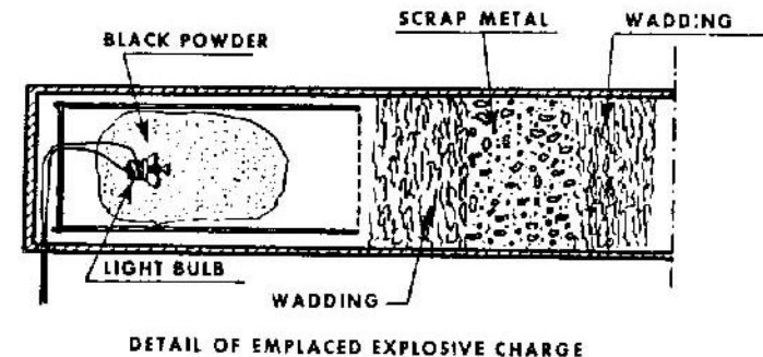
DETAIL OF EMPLACED EXPLOSIVE CHARGE
