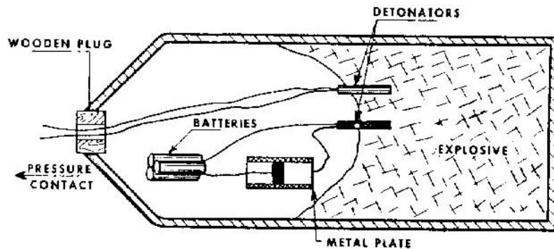
Figure 24 (UNCLASSIFIED). FLN ontillift mine (U).
