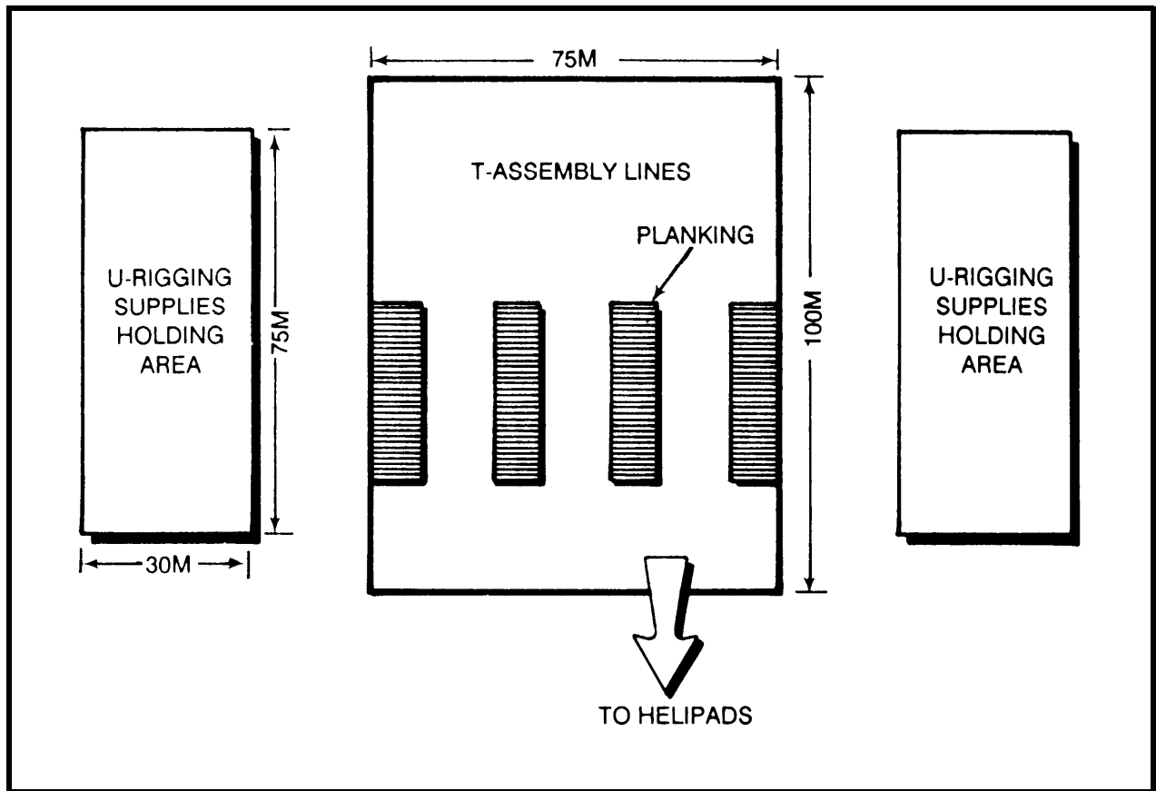
Figure 6-4. Holding areas
