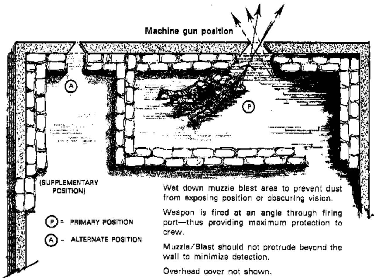
Figure C-5a Machine Gun Position
