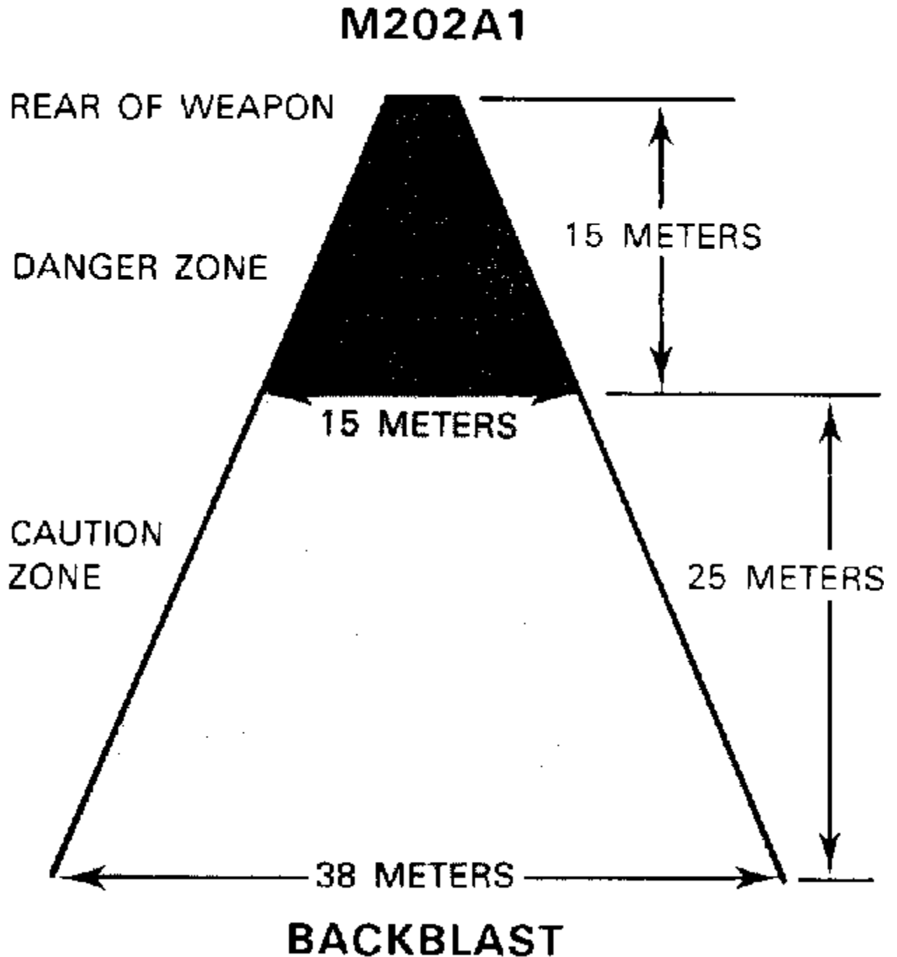
Figure 4-5. M202A1
