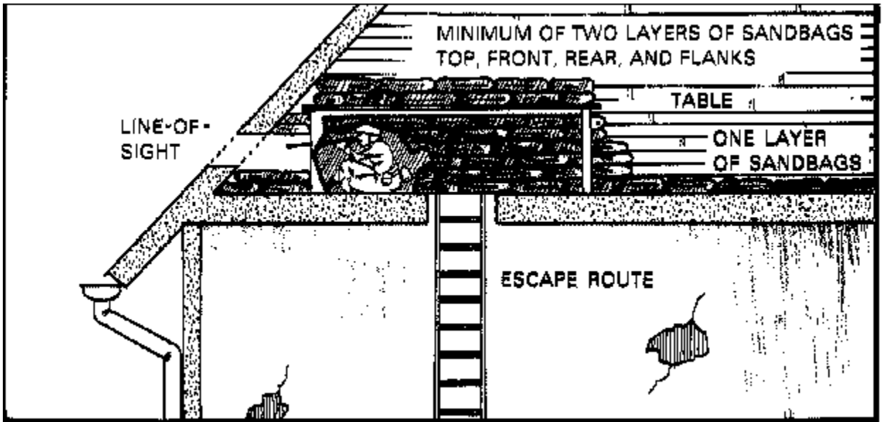
Figure C-6a Attic Position
