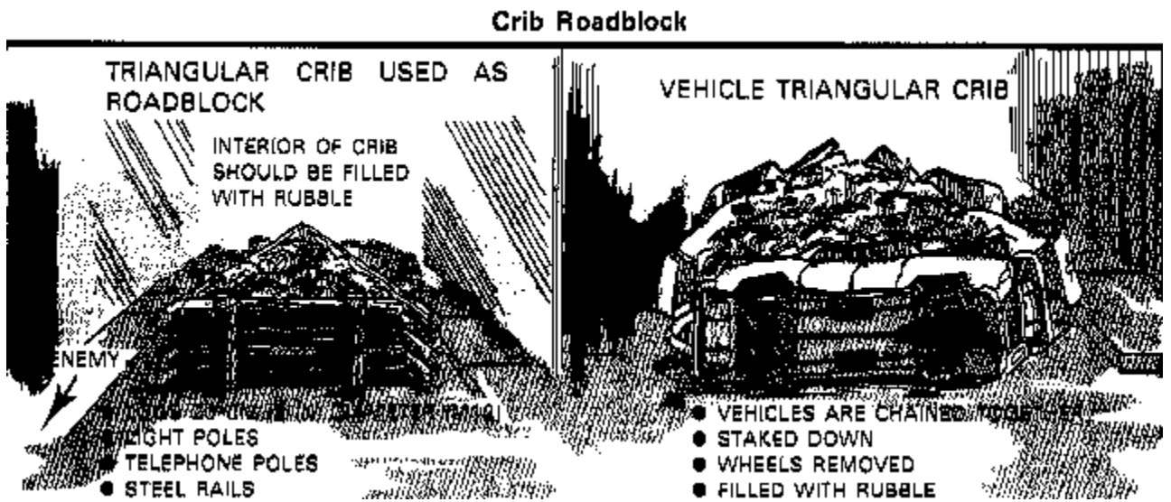
Figure D-6a Crib Roadblock
