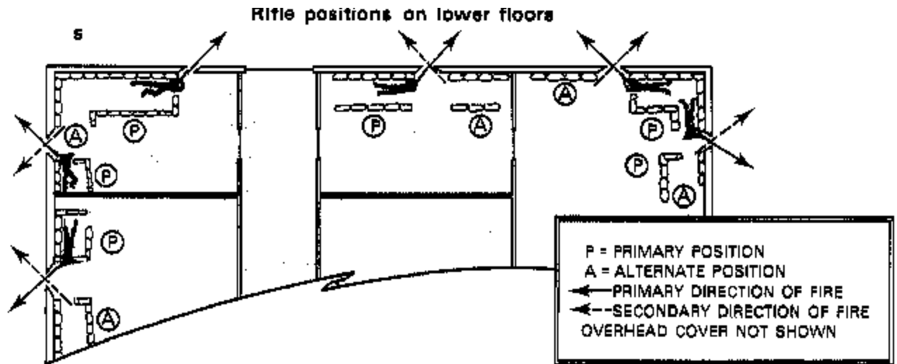
Figure C-4c Rifle Positions on Lower Floor
