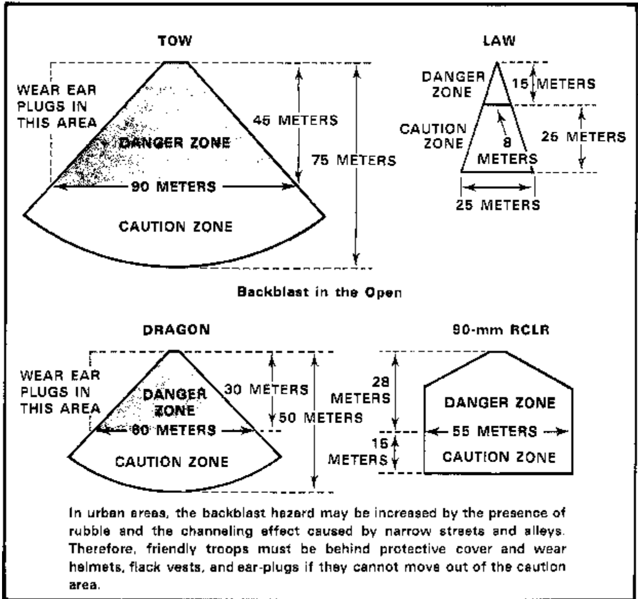
Figure B-8. Back blast Hazard
