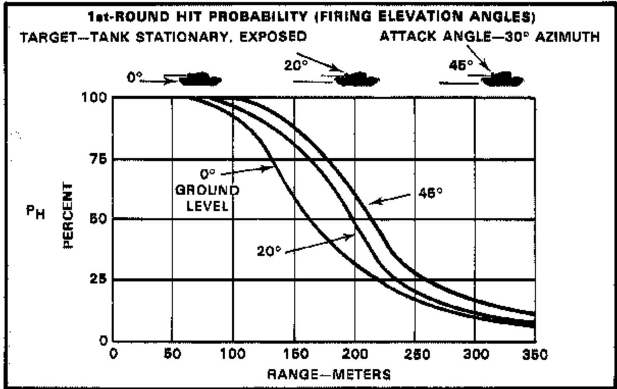
Figure B-7b 1st-Round Hit Probability.
