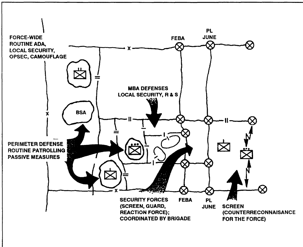
Figure 4-3. Counterreconnaissance considerations.
