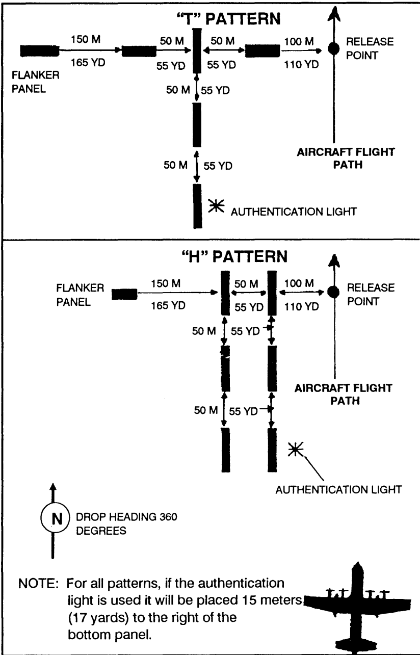
Figure 6-4. Panel emplacement.
