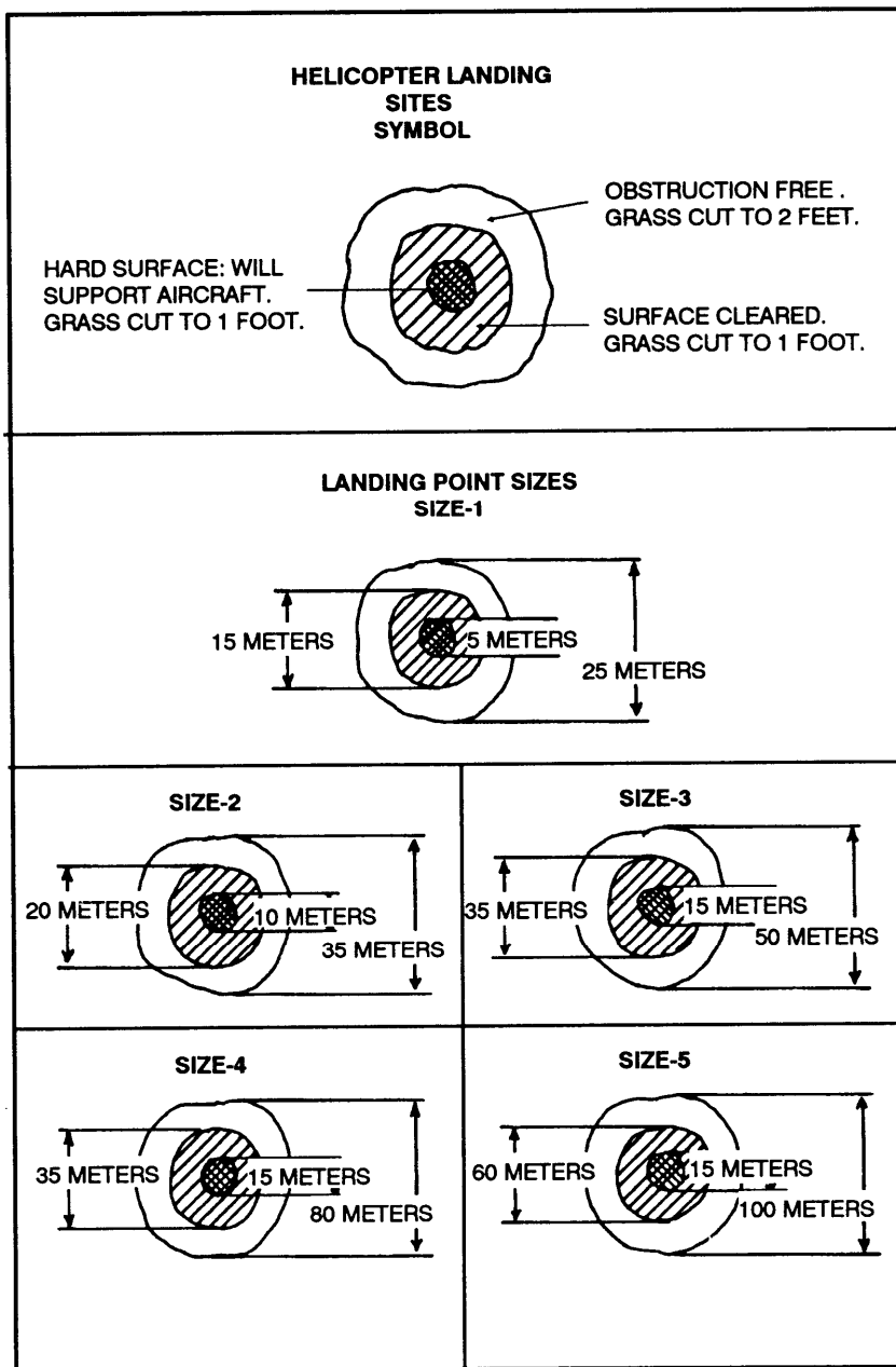
Figure 4-3. Landing points.
