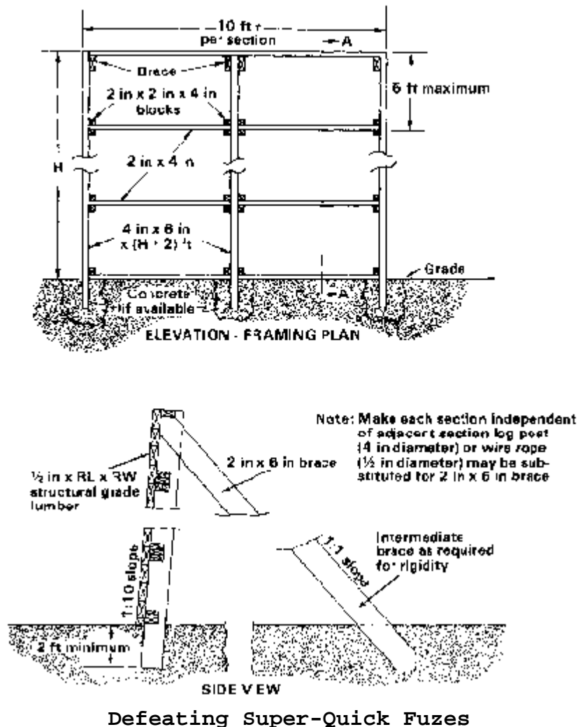
Typical standoff framing with dimensioned wood triggering screen
