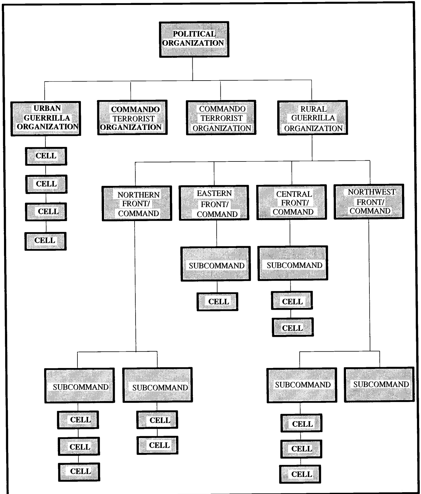
Figure 11-1. Insurgent organization.
