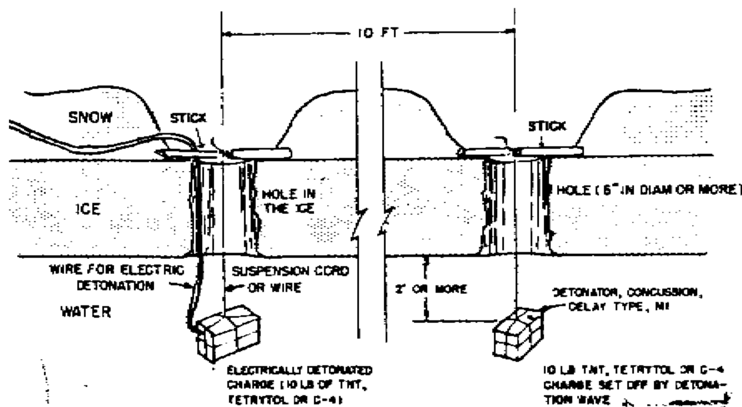
Figure 6-34. Method of placing charges in ice.
