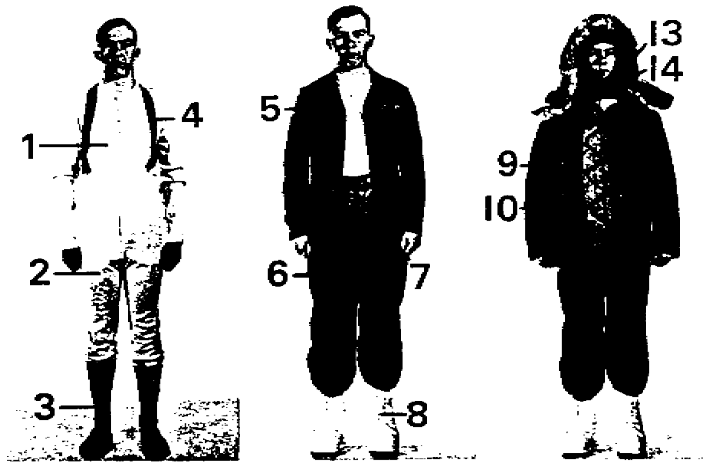
Figure 2-2. Basic components of cold-dry uniform.
