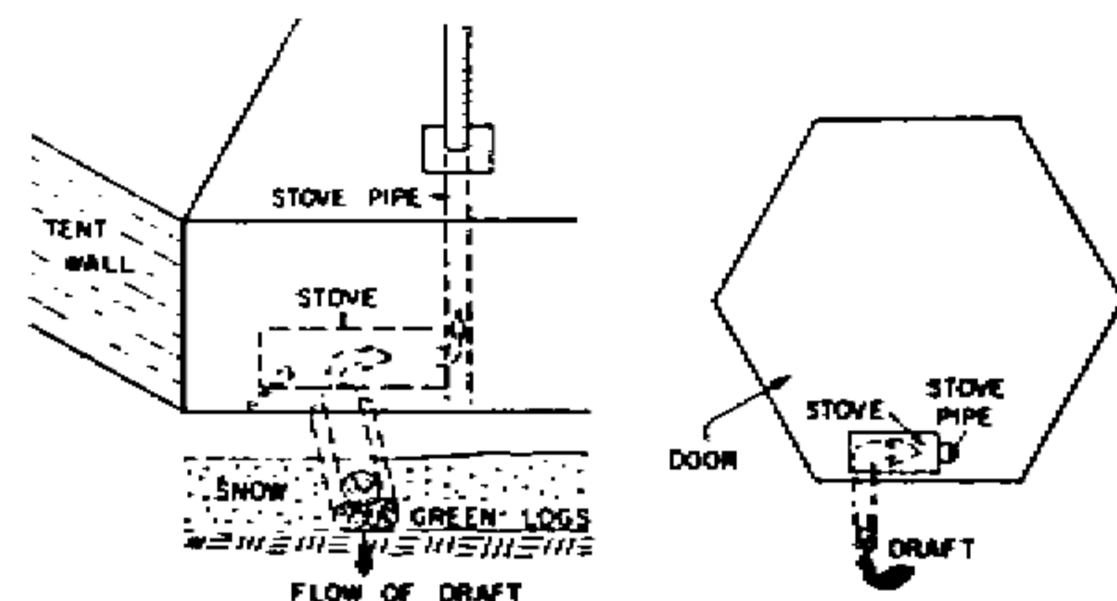
Figure 3-7. Draft channel for stove.
