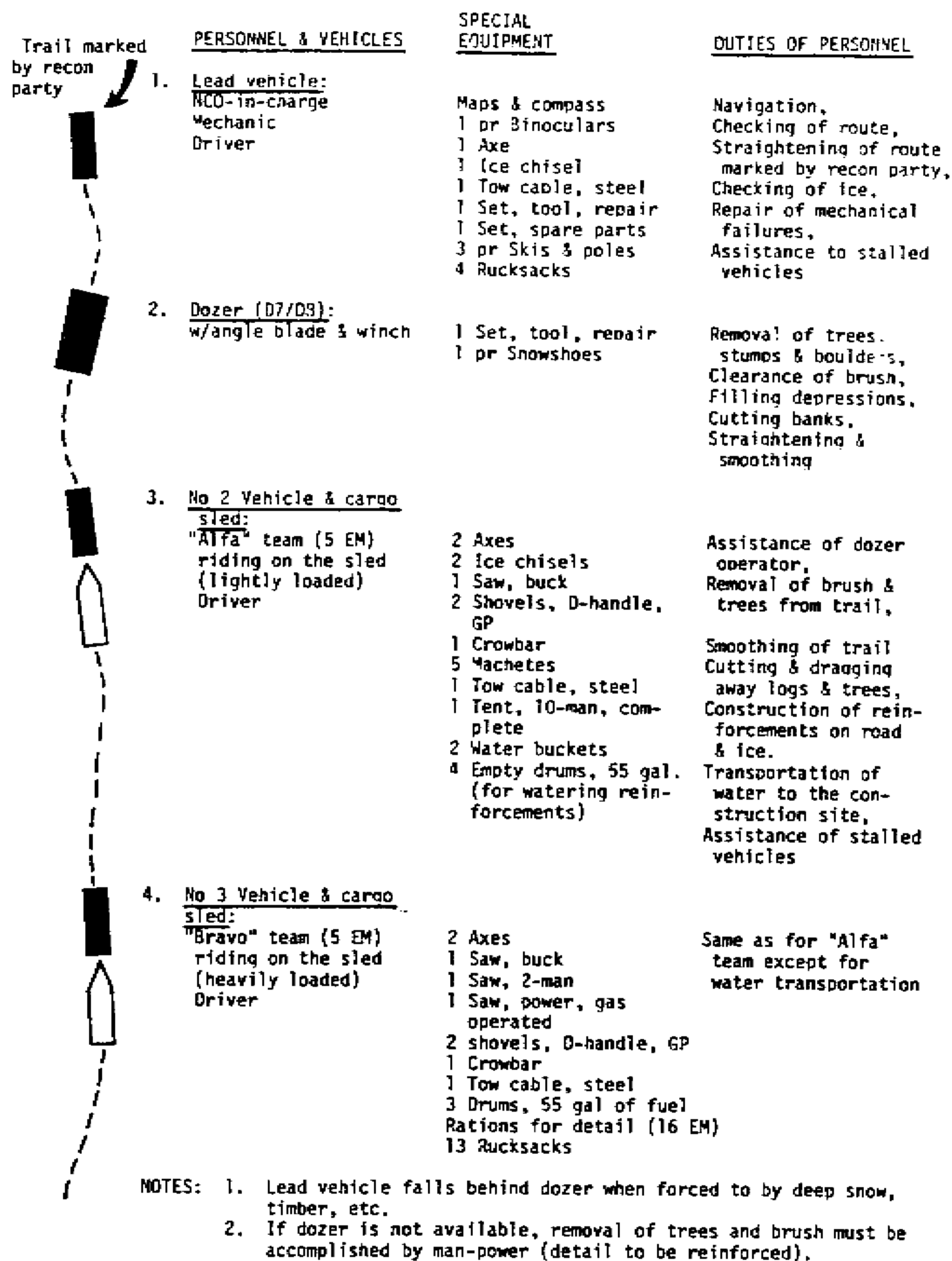
Figure 5-6. Construction detail for winter roads.
