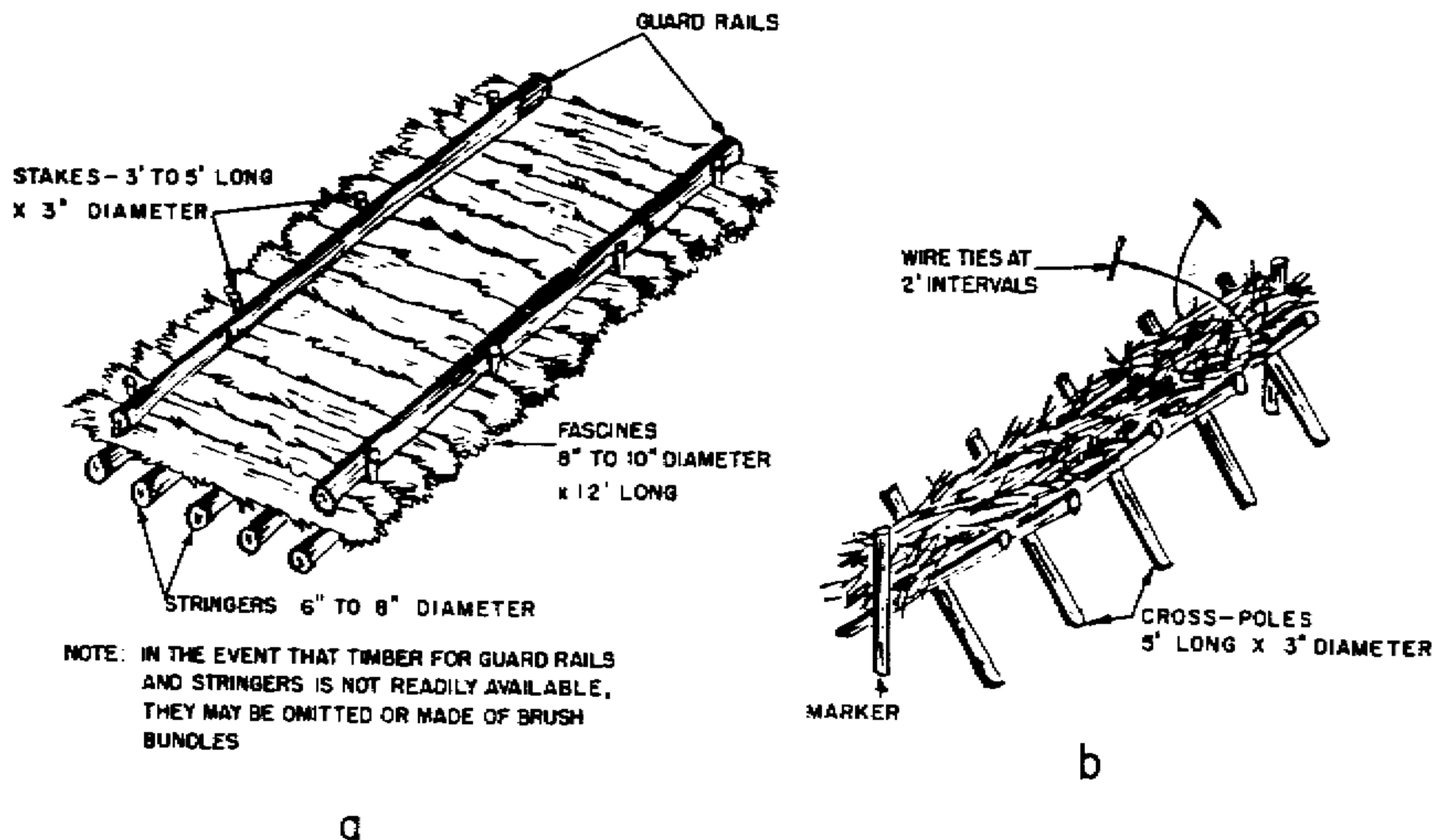
Figure 5-11. Types of corduroy roads.
