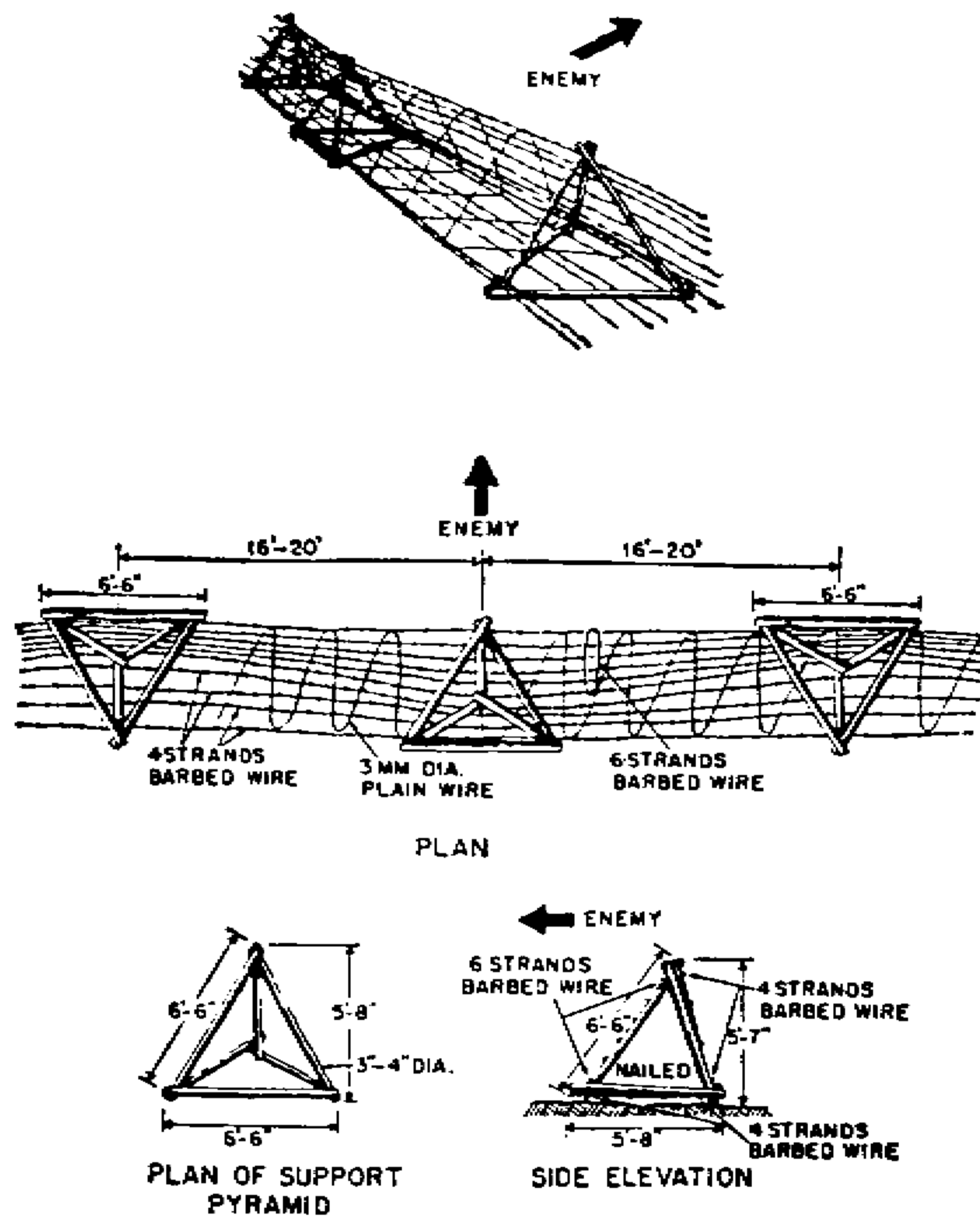
Figure 6-37. Lapland barbed wire.
