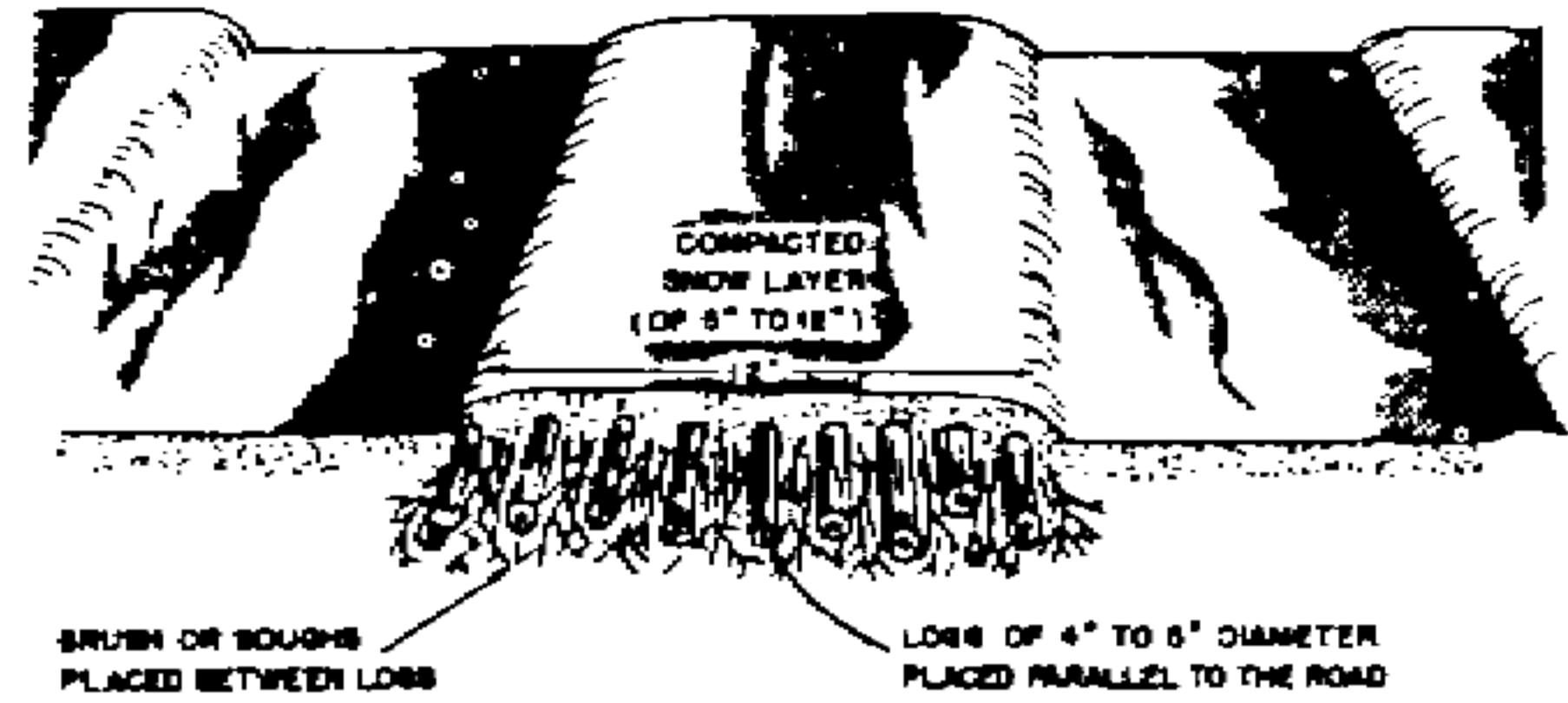
Figure 5-9. Road reinforced with brush, logs, and snow.
