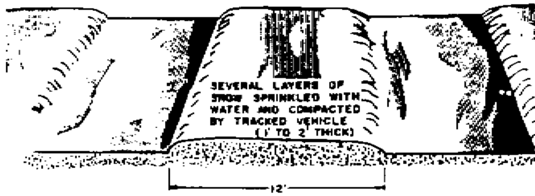
Figure 5-7. Road reinforced with snow.
