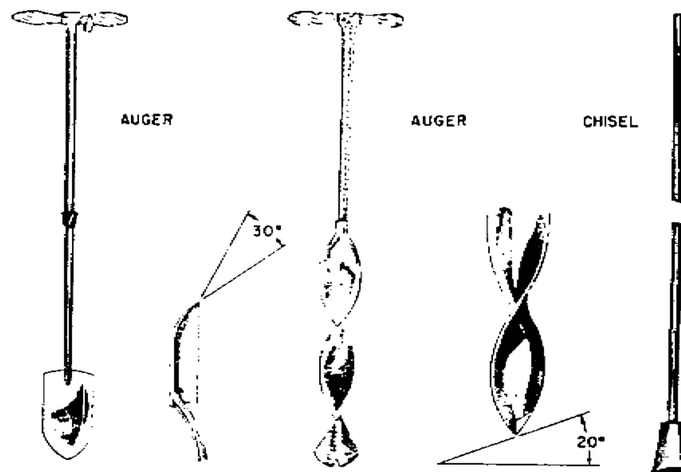
Figure 6-35. Types of ice augers and ice chisel.
