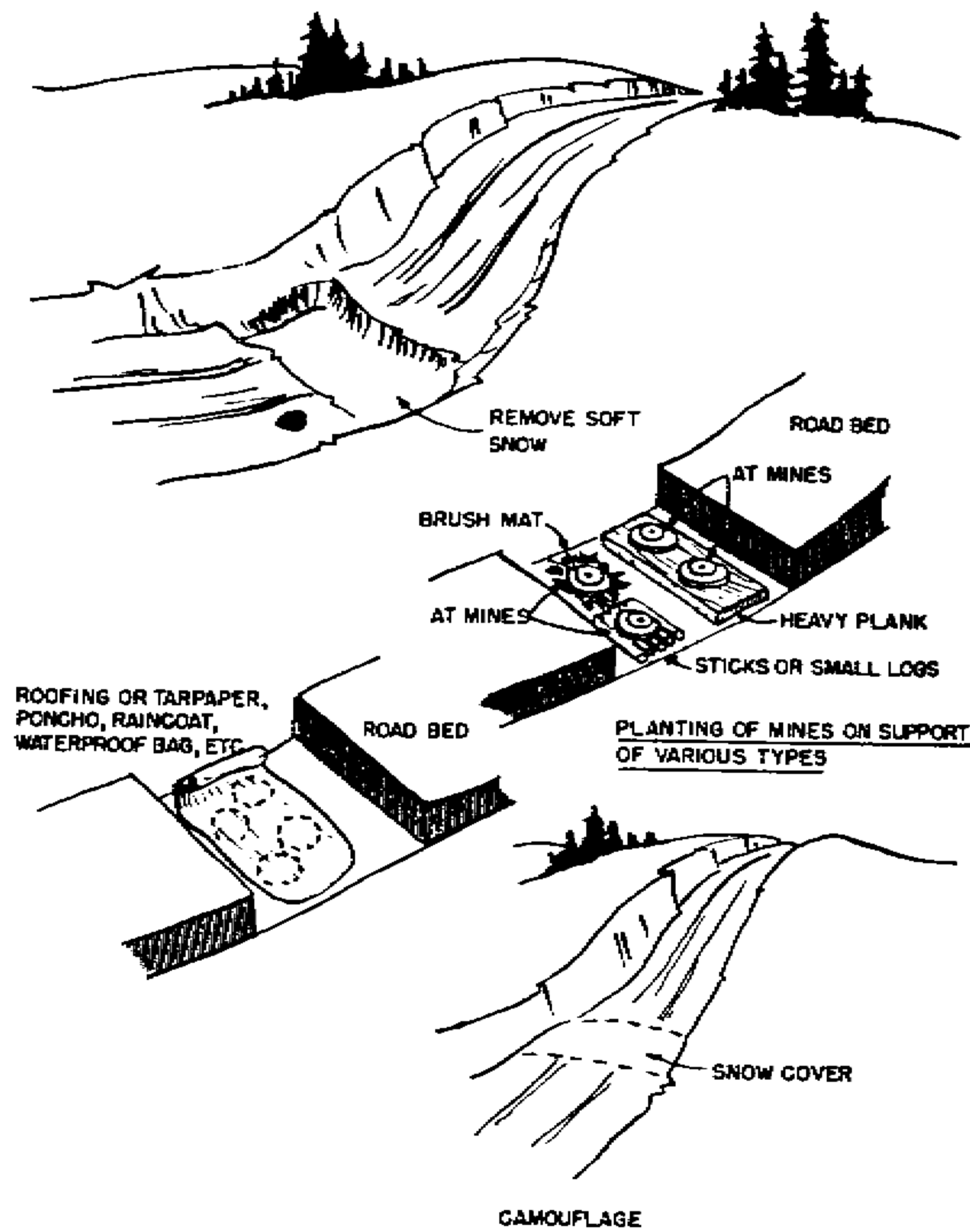
Figure 6-32. Laying mines in deep snow.
