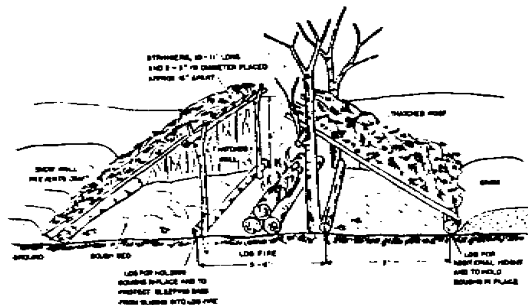
Figure 3-11. Double lean-to.
