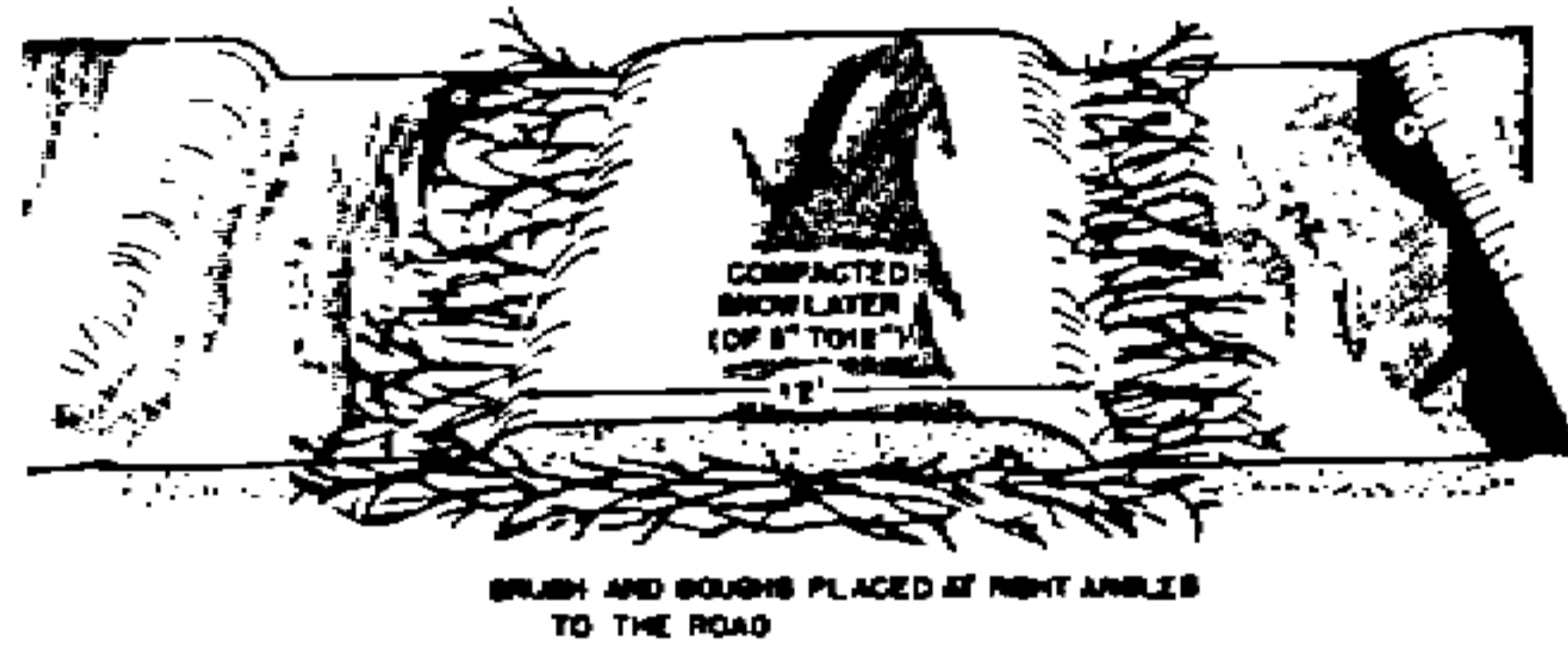
Figure 5-8. Road reinforced with brush and snow.
