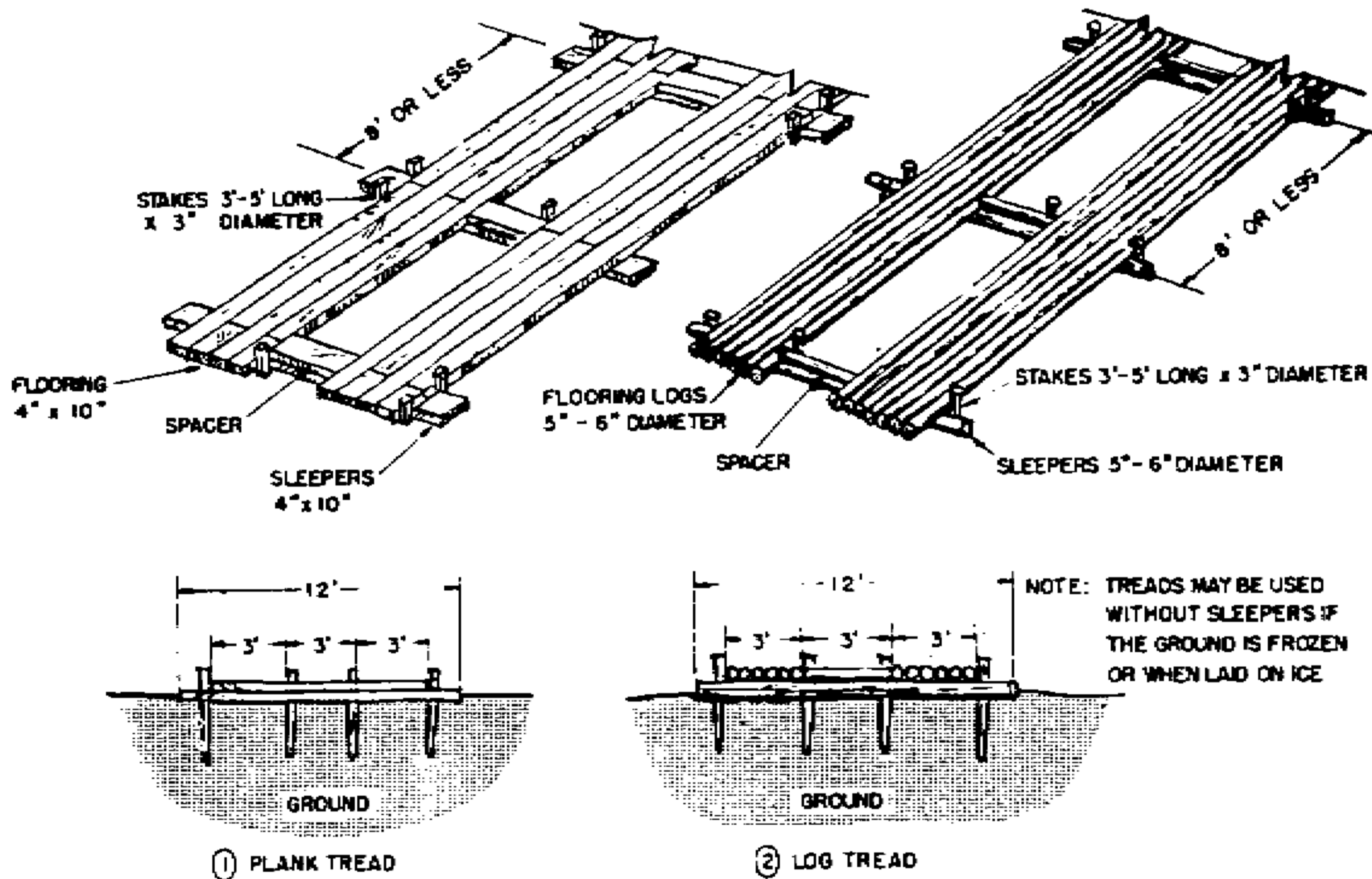
Figure 5-10. Road reinforced with tread.
