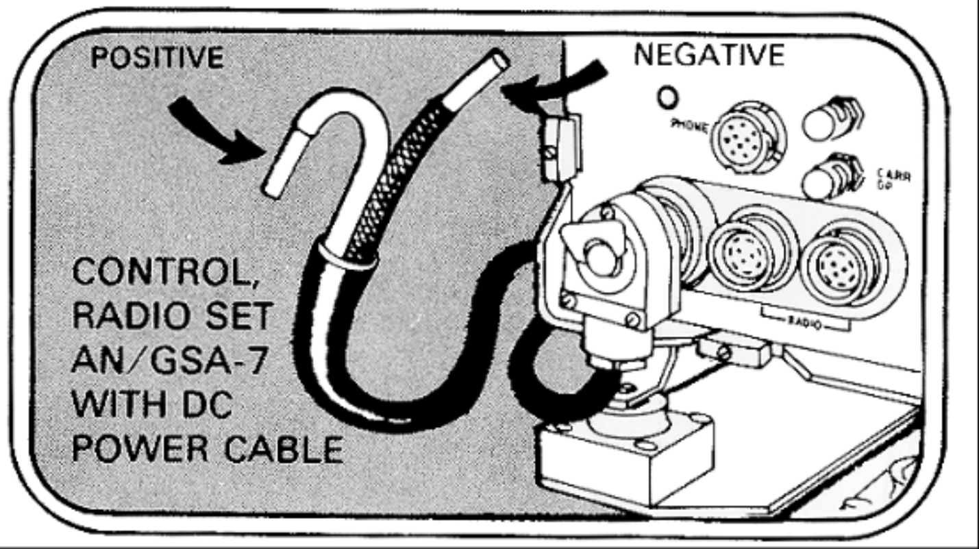
Figure F-10. Check polarity.
