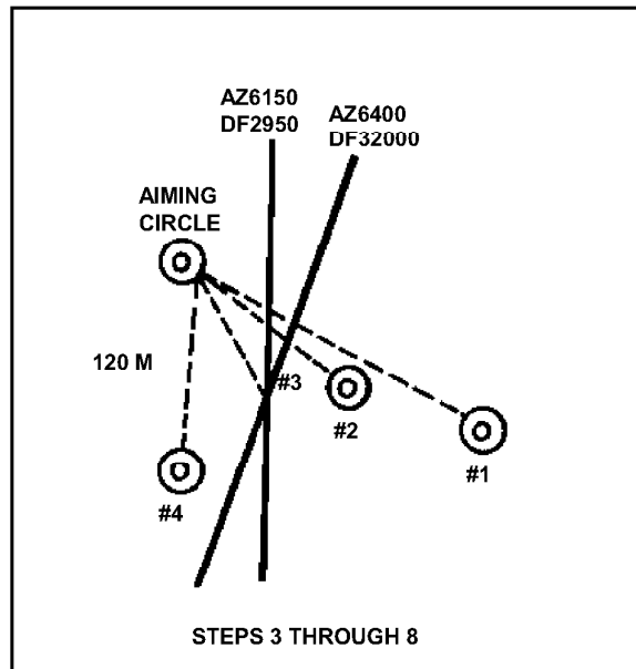
Figure E-4c. Determination of piece displacement (continued).
