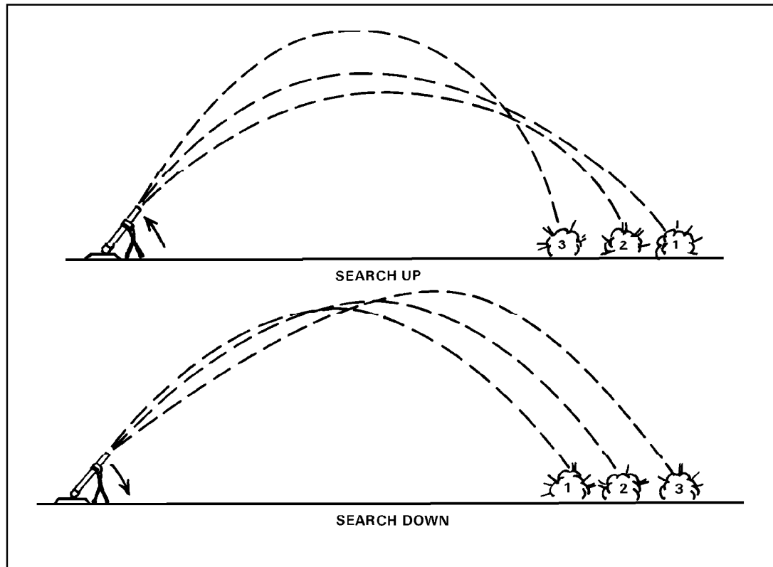
Figure 13-7. Fall of rounds during search mission.
