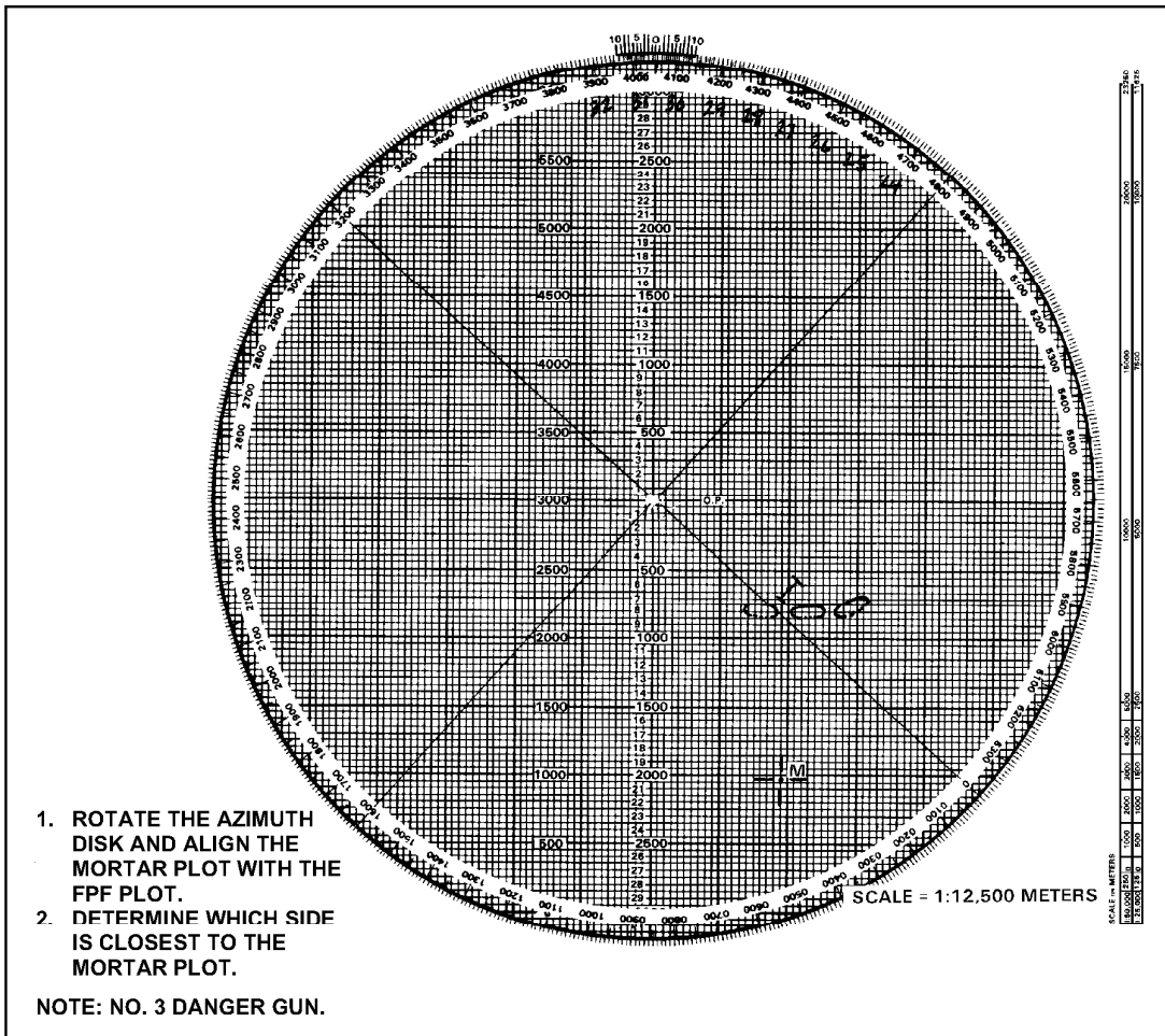
Figure 14-16. Determination of danger mortar.
