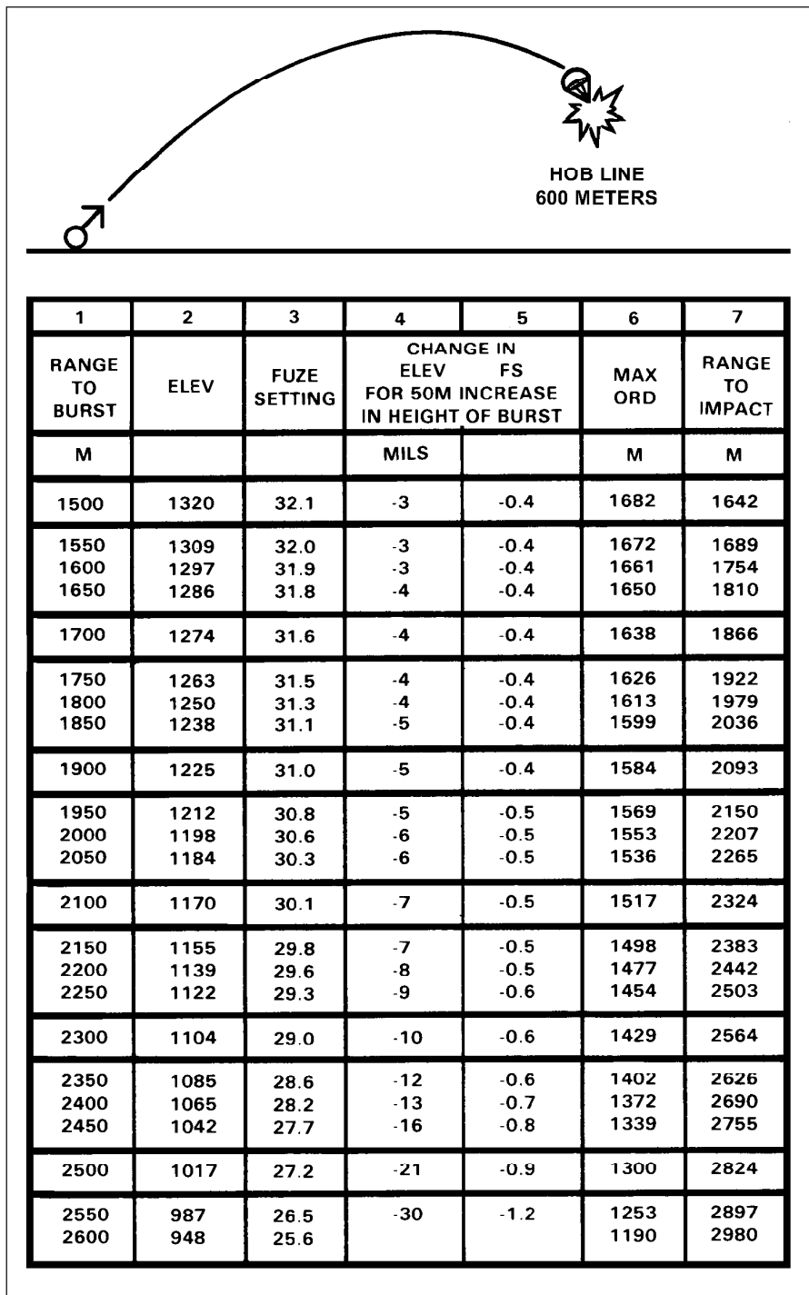
Figure 13-11. Height of burst line 81-mm.
