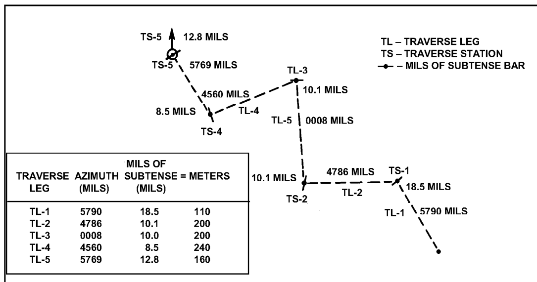
Figure C-9. Construction of a diagram.
