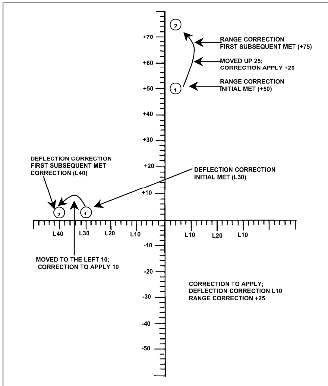
Figure 4-27. Deflection and range corrections.
