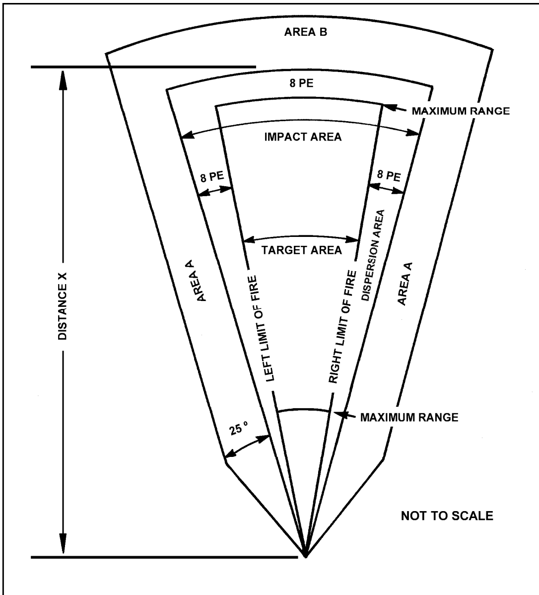
Figure B-1. Mortar surface danger zone.
