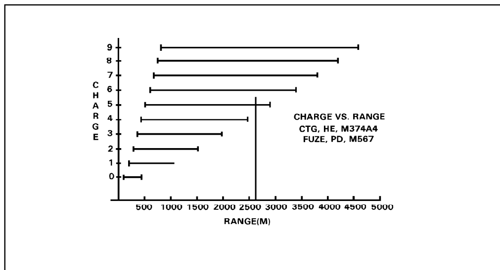
Figure 12-6. Charge zone and range.
