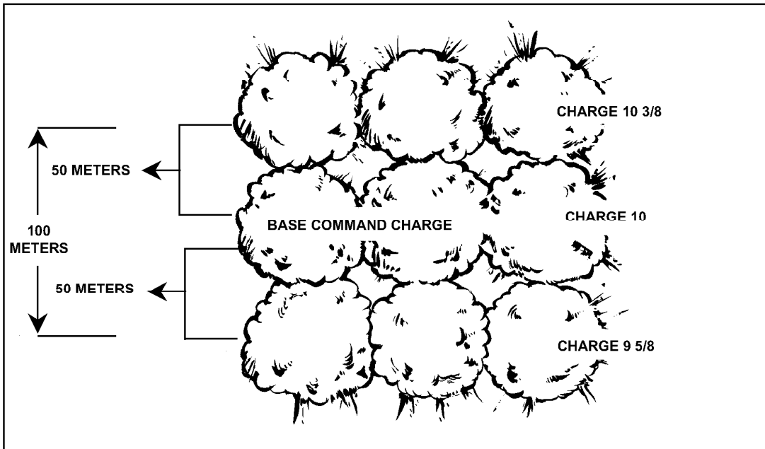
Figure 13-8. Firing without extension, 100-meter zone.
