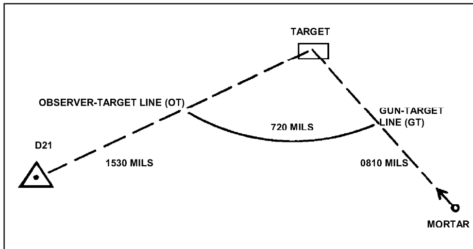
Figure 4-9. Angle T exceeding 500 mils.
