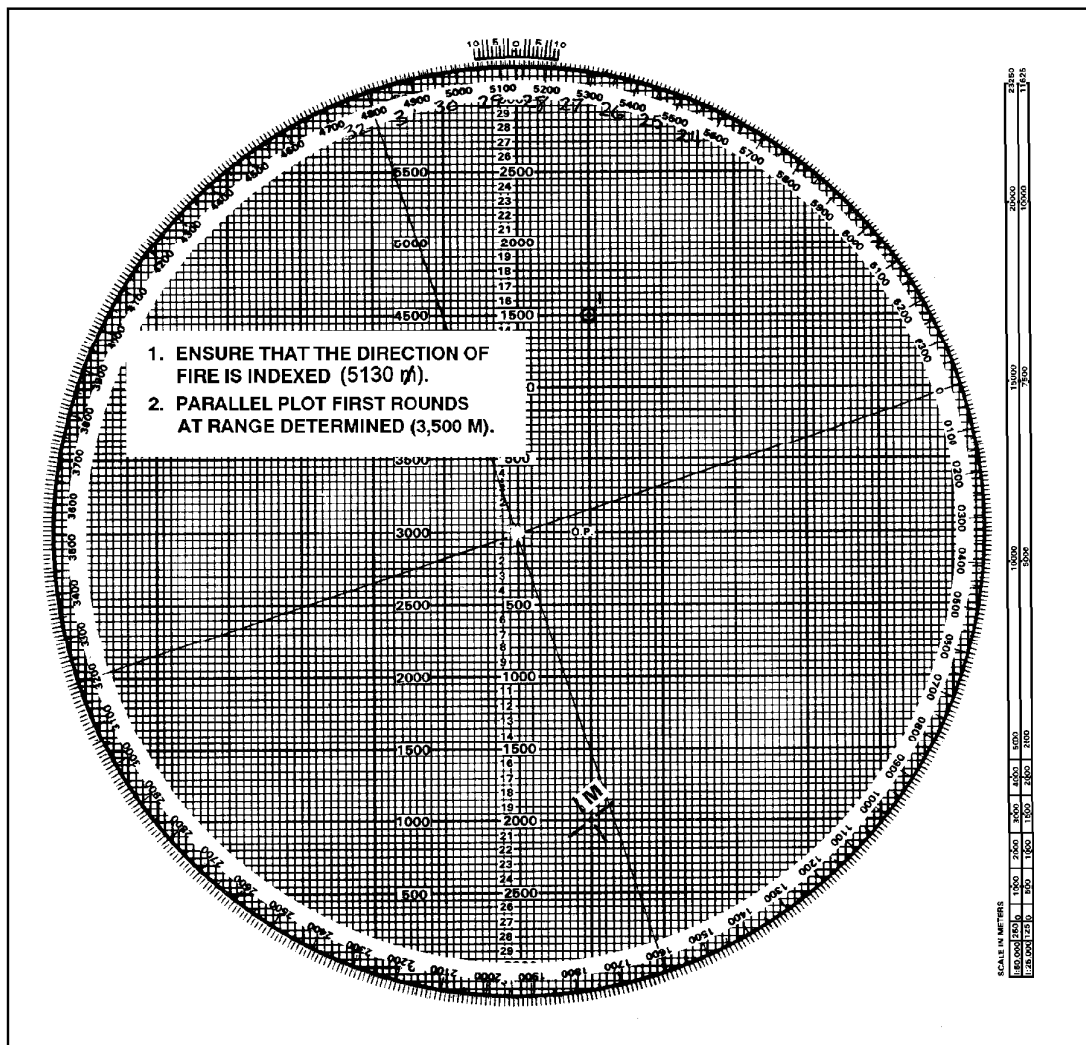
Figure 12-12. Plotting of first round.
