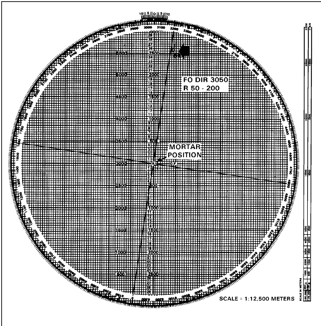
Figure 12-7. Plotting of observer's correction.
