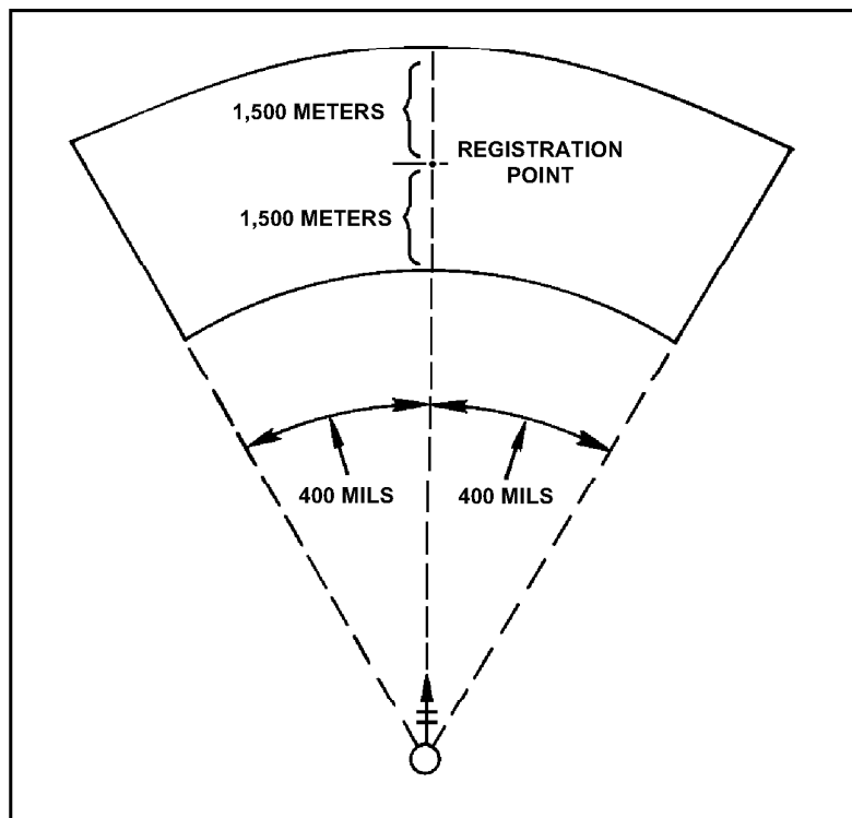
Figure 14-4. Transfer limits for one registration point.
