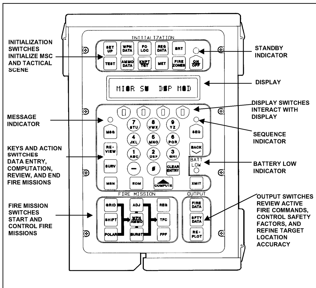
Figure 7-1. Mortar ballistic computer switch panel.
