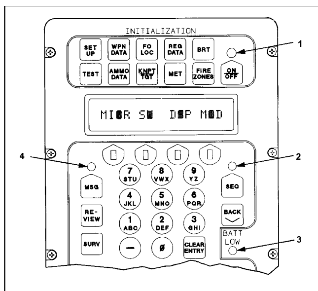
Figure 6-8. LED Indicators.
