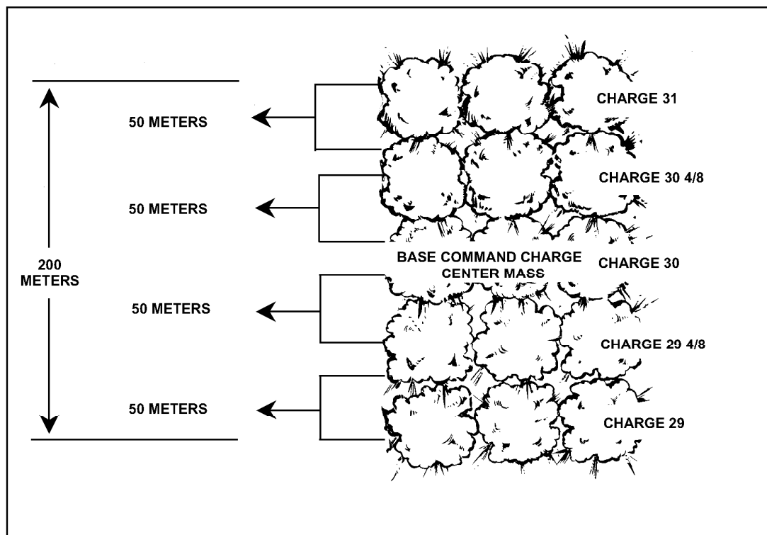
Figure 13-9. Firing without extension, 200-meter zone.
