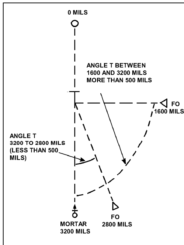
Figure 4-8. Angle T between 400 and 1600 mils.
