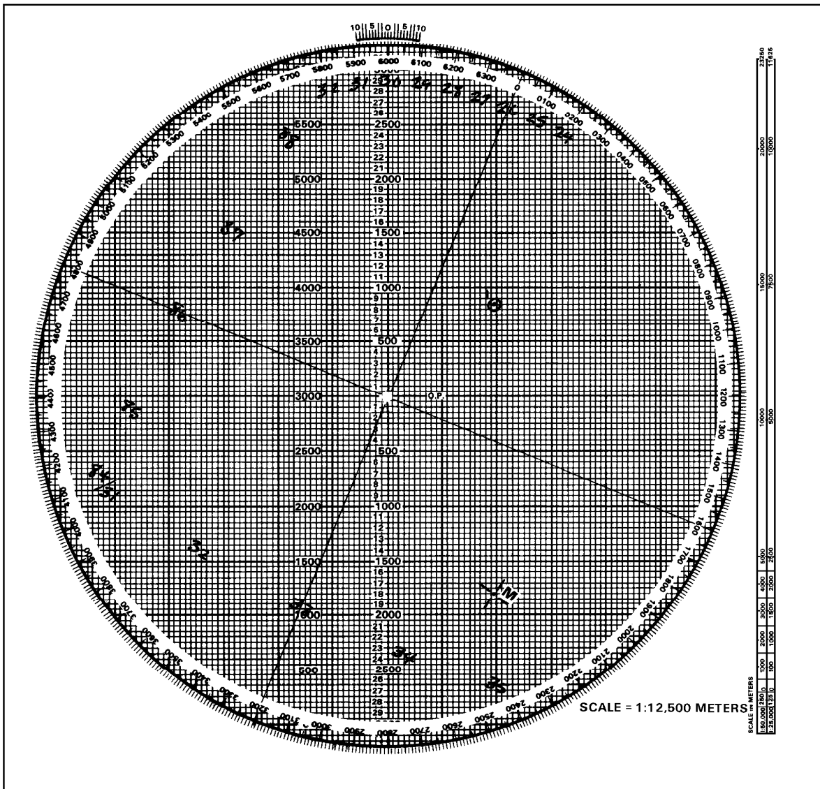
Figure 12-13. Parallel-line plotting.
