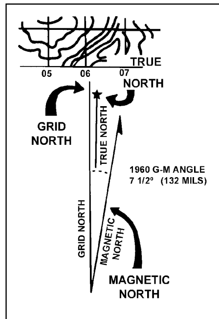
Figure 7-2. Declination diagram.
