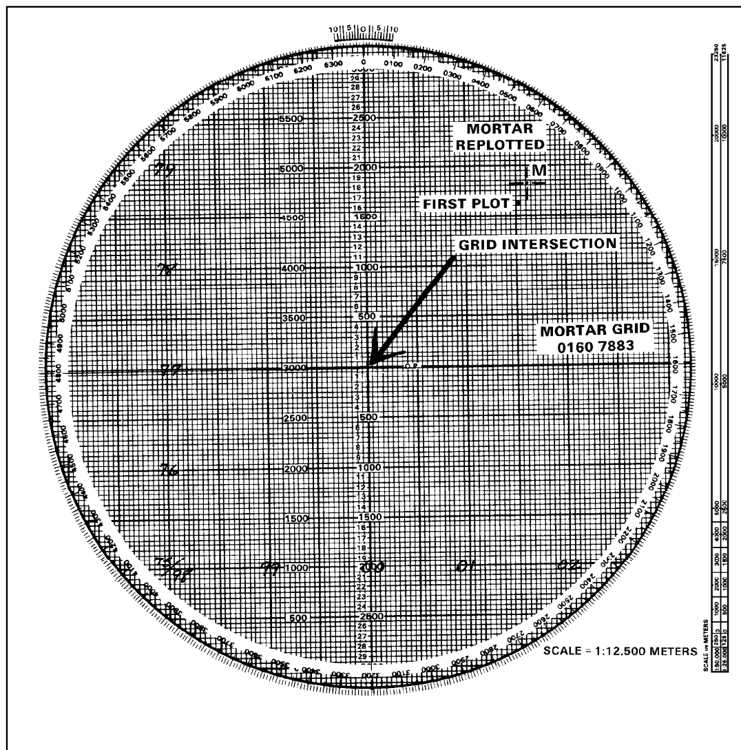
Figure 12-19. Replotting of mortar location.
