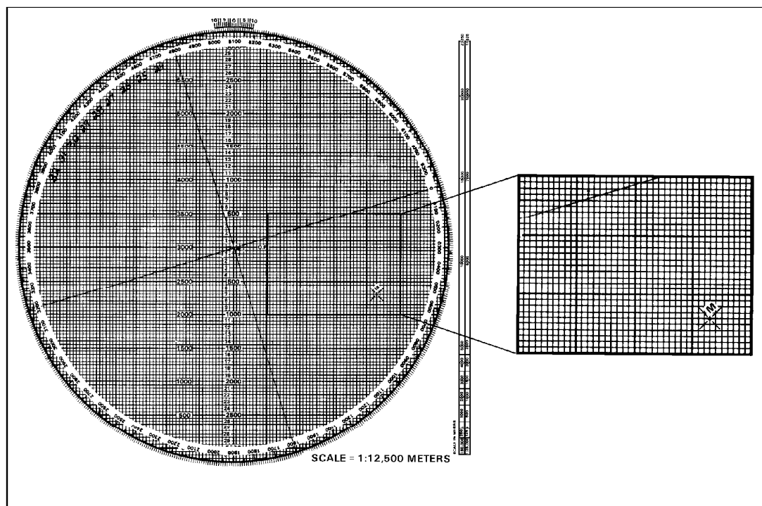
Figure 14-15. Drawing FPF symbol with attitude indexed.
