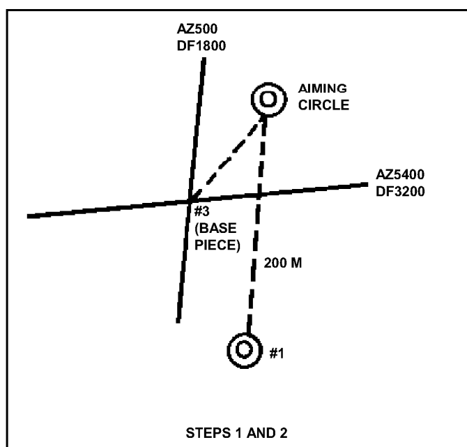
Figure E-4b. Determination of piece displacement (continued).
