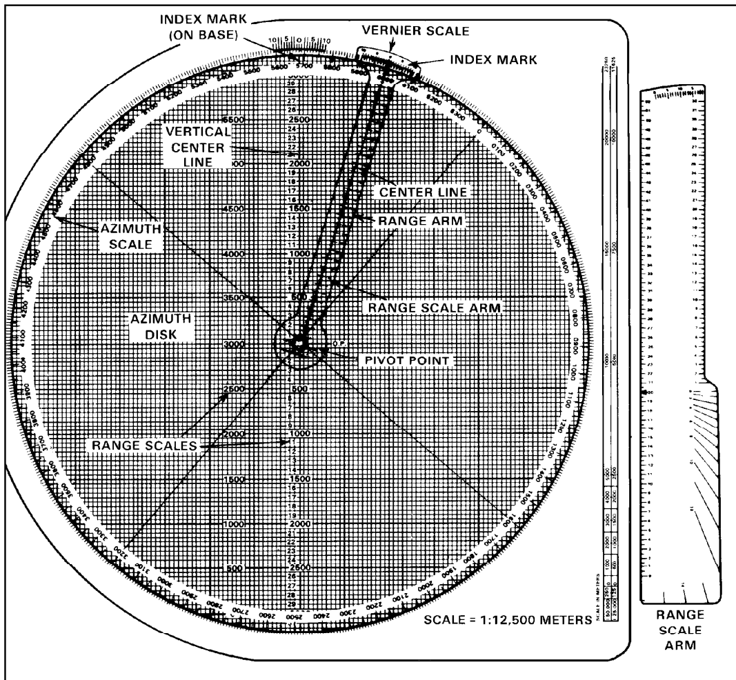
Figure 11-1. M16 plotting board.
