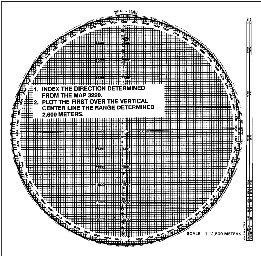
Figure 12-1. Preparation of the plotting board.
