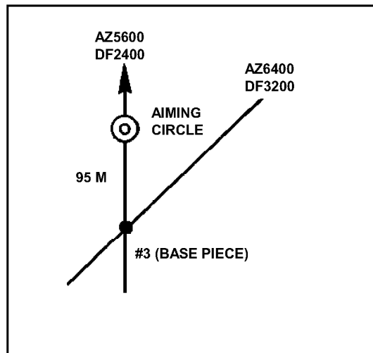
Figure E-4a. Determination of piece displacement.
