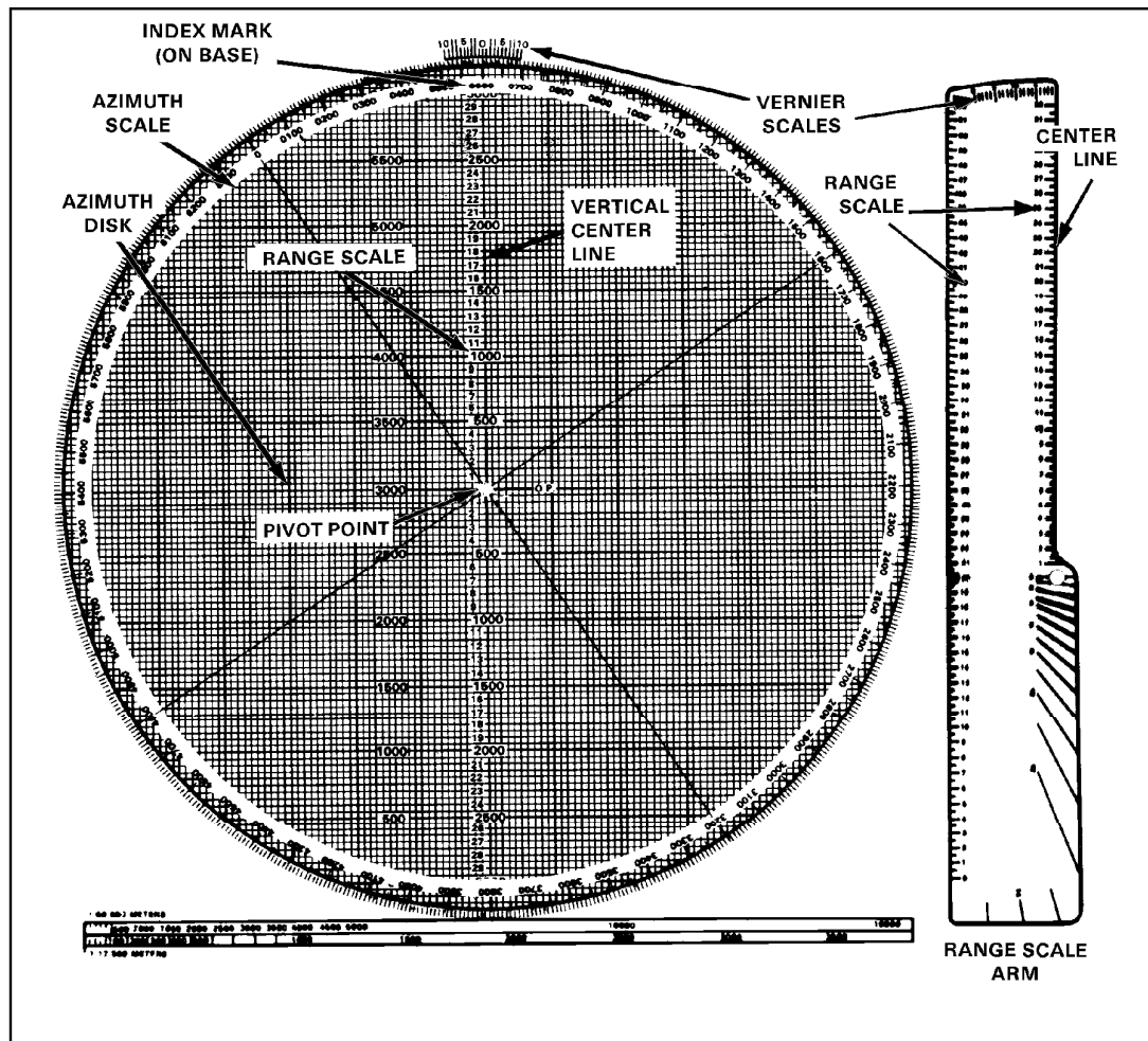
Figure 11-2. M19 plotting board.
