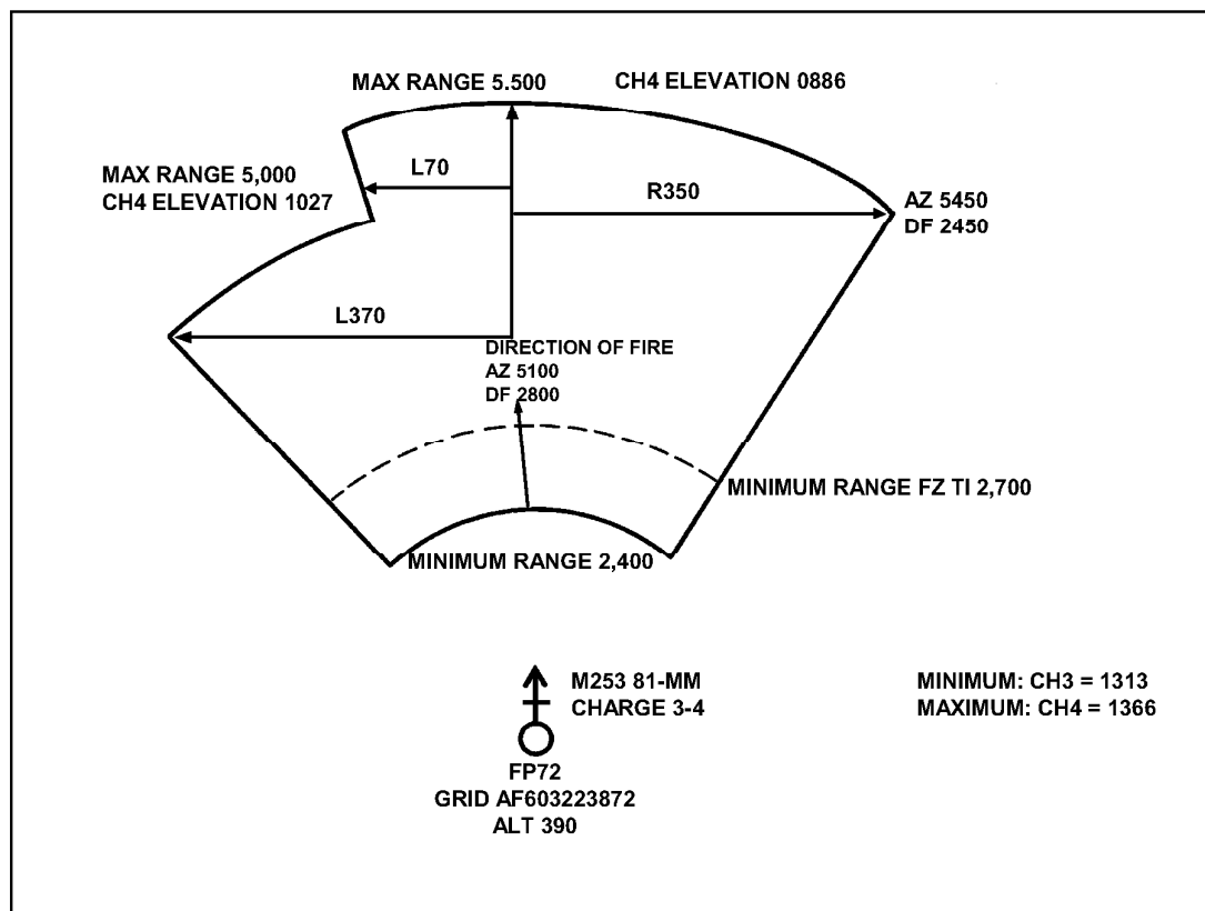
Figure B-3. Basic safety diagram.
