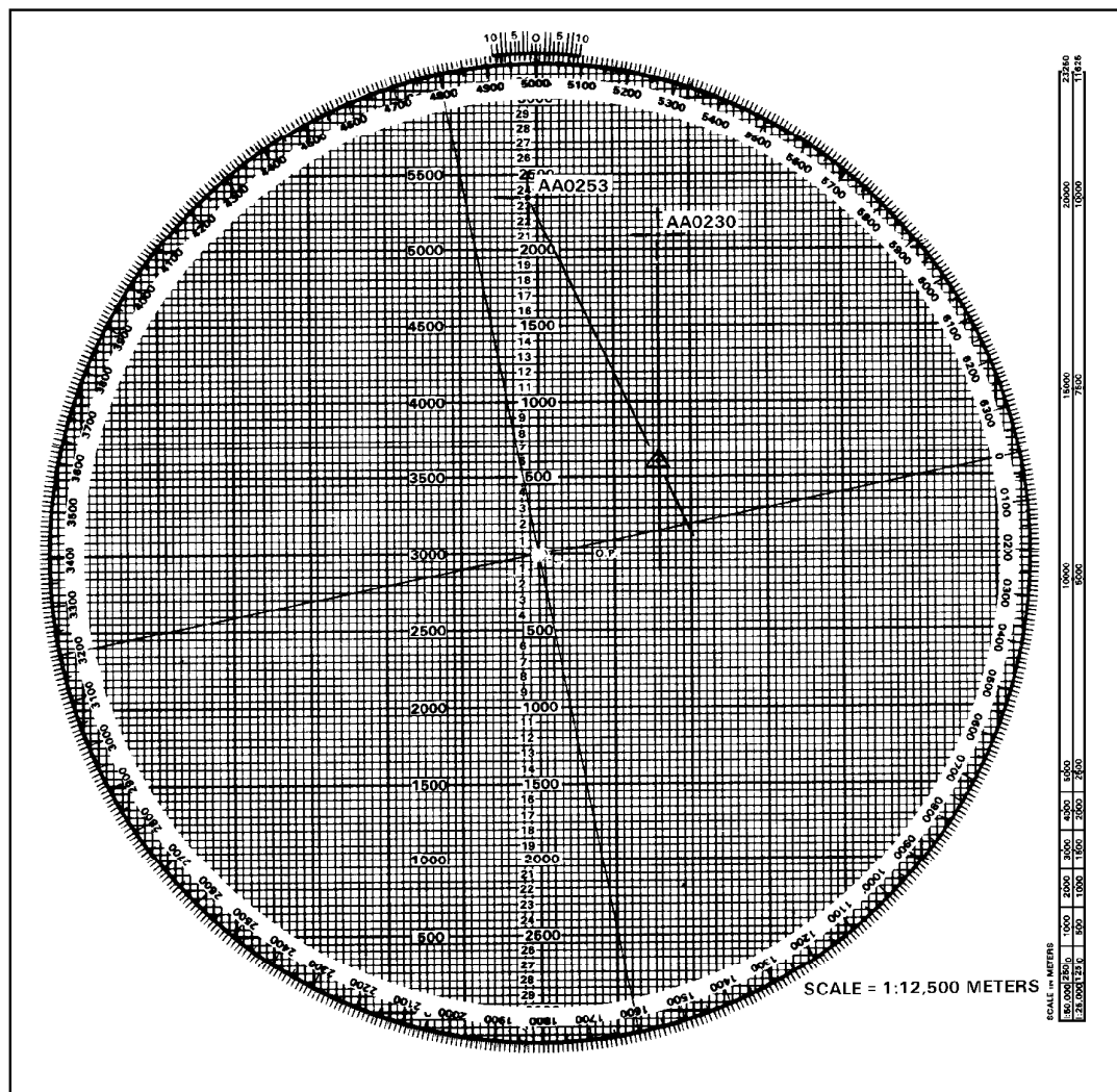
Figure 12-23. Resection.
