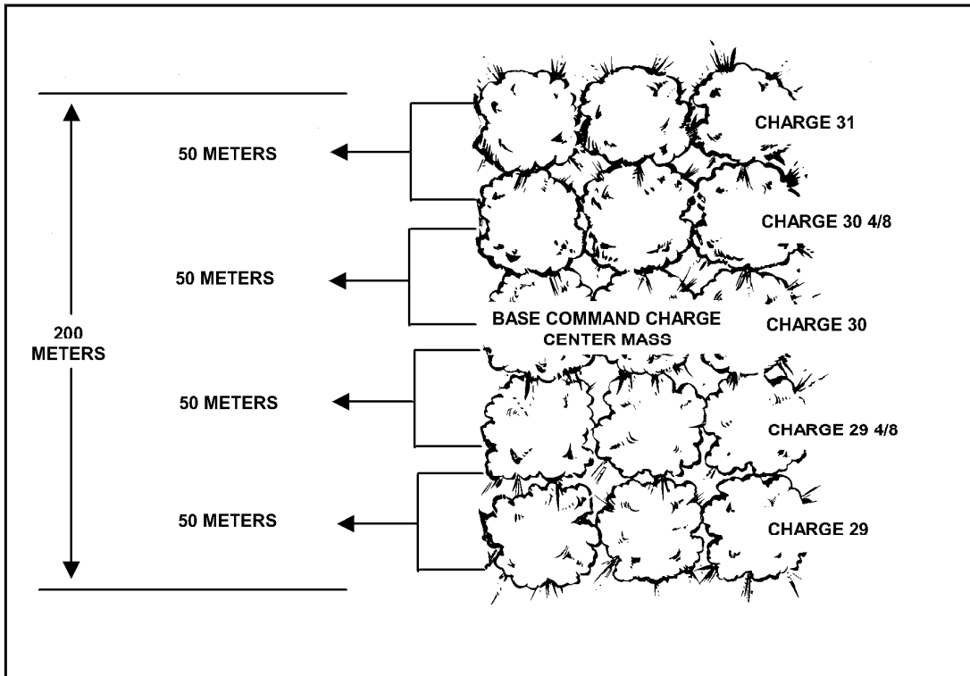
Figure 8-8. Firing 200-meter zone.
