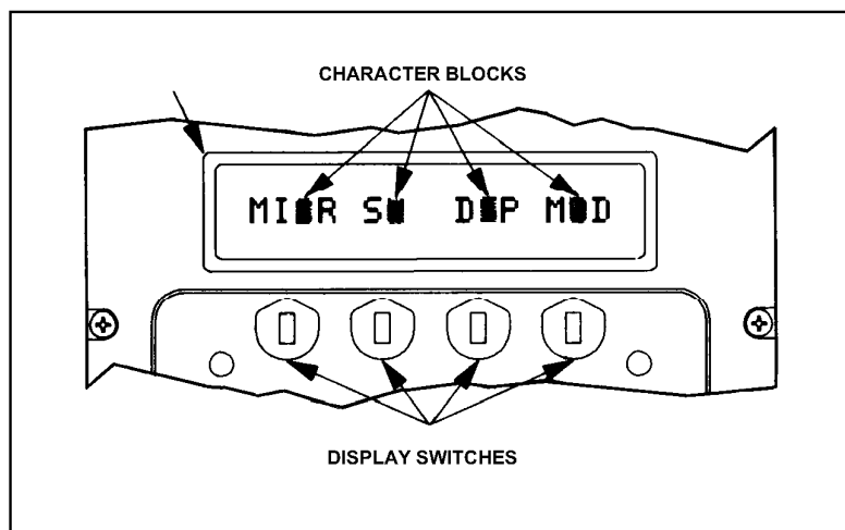
Figure 6-7. Display switches.
