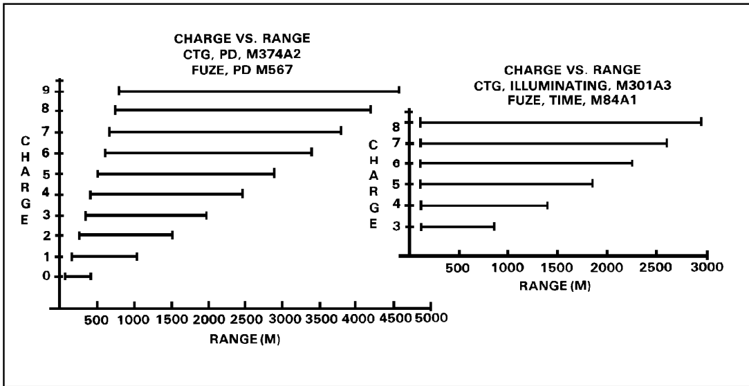
Figure 12-4. Charge-vs-range chart.
