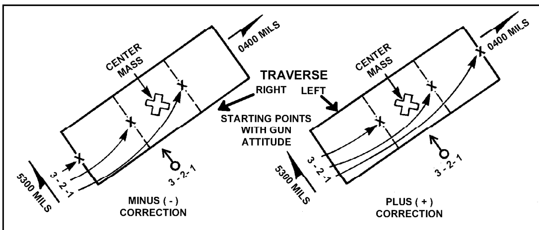
Figure 8-5. Situation charts numbers 4 and 5.
