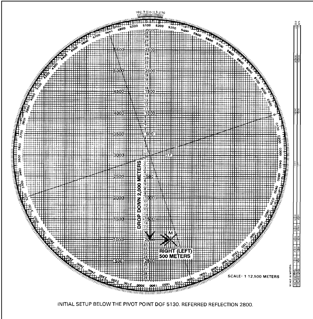
Figure 12-11. Plotting of mortar position.
