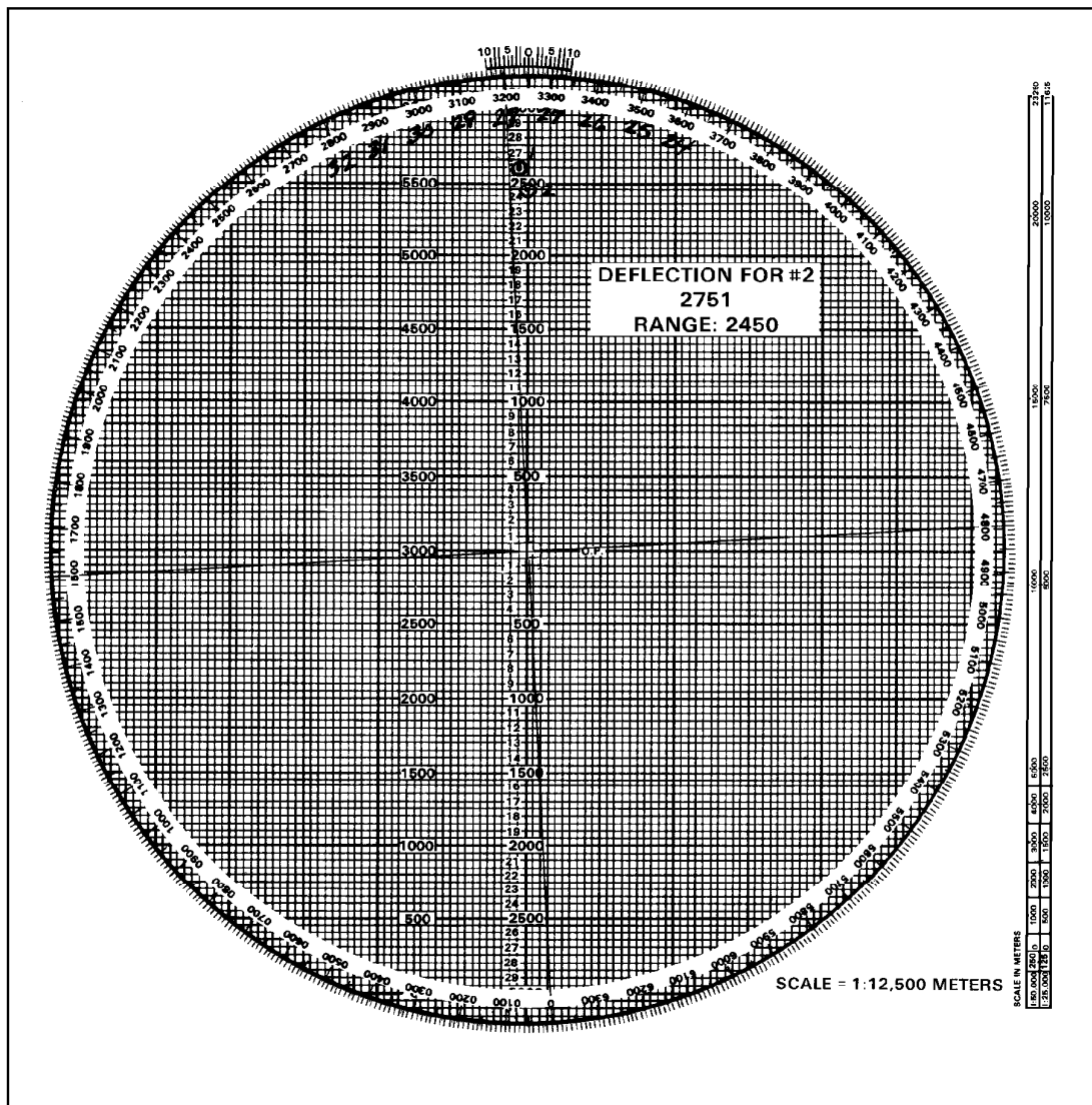
Figure 12-8. Determination of deflection and range.
