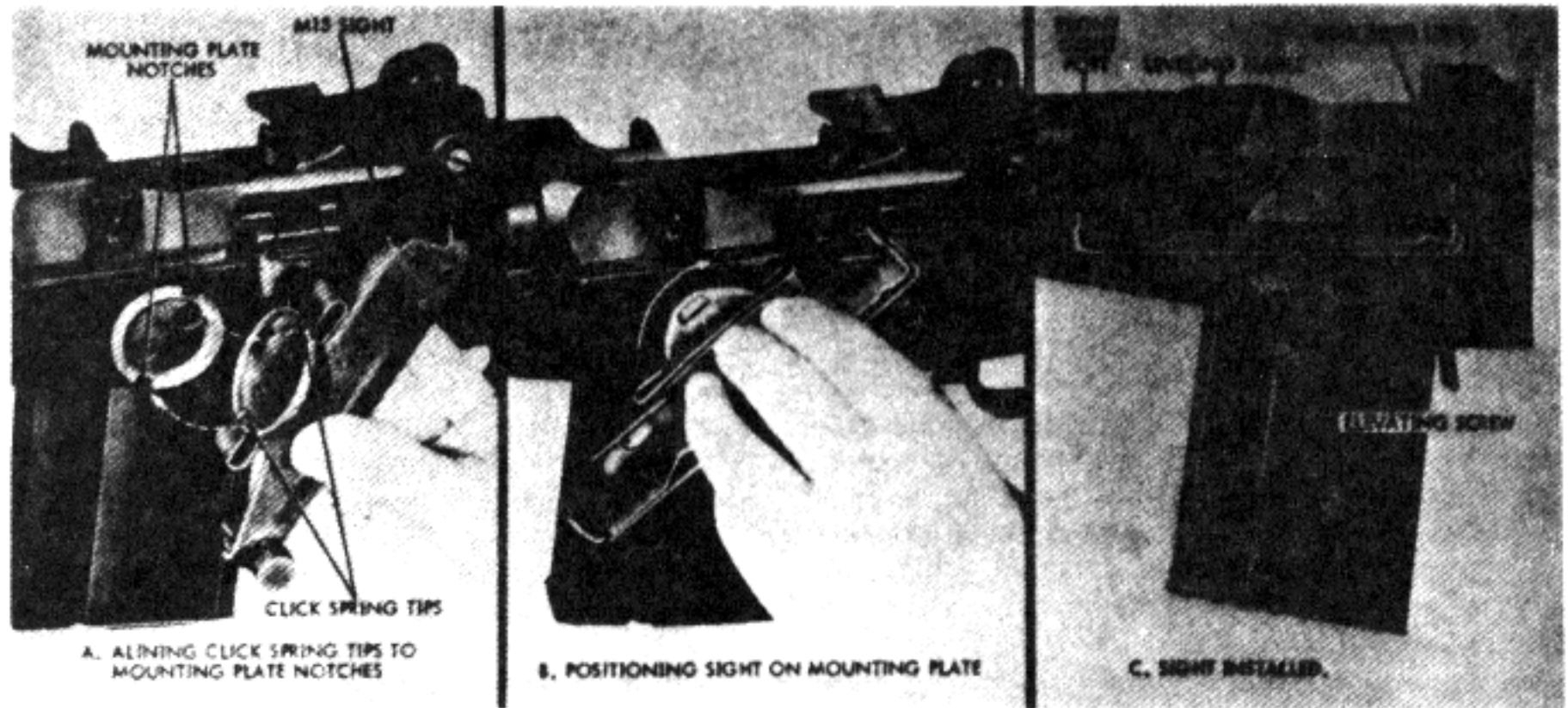
Figure 56. Installation of M15 grenade launcher sight.
