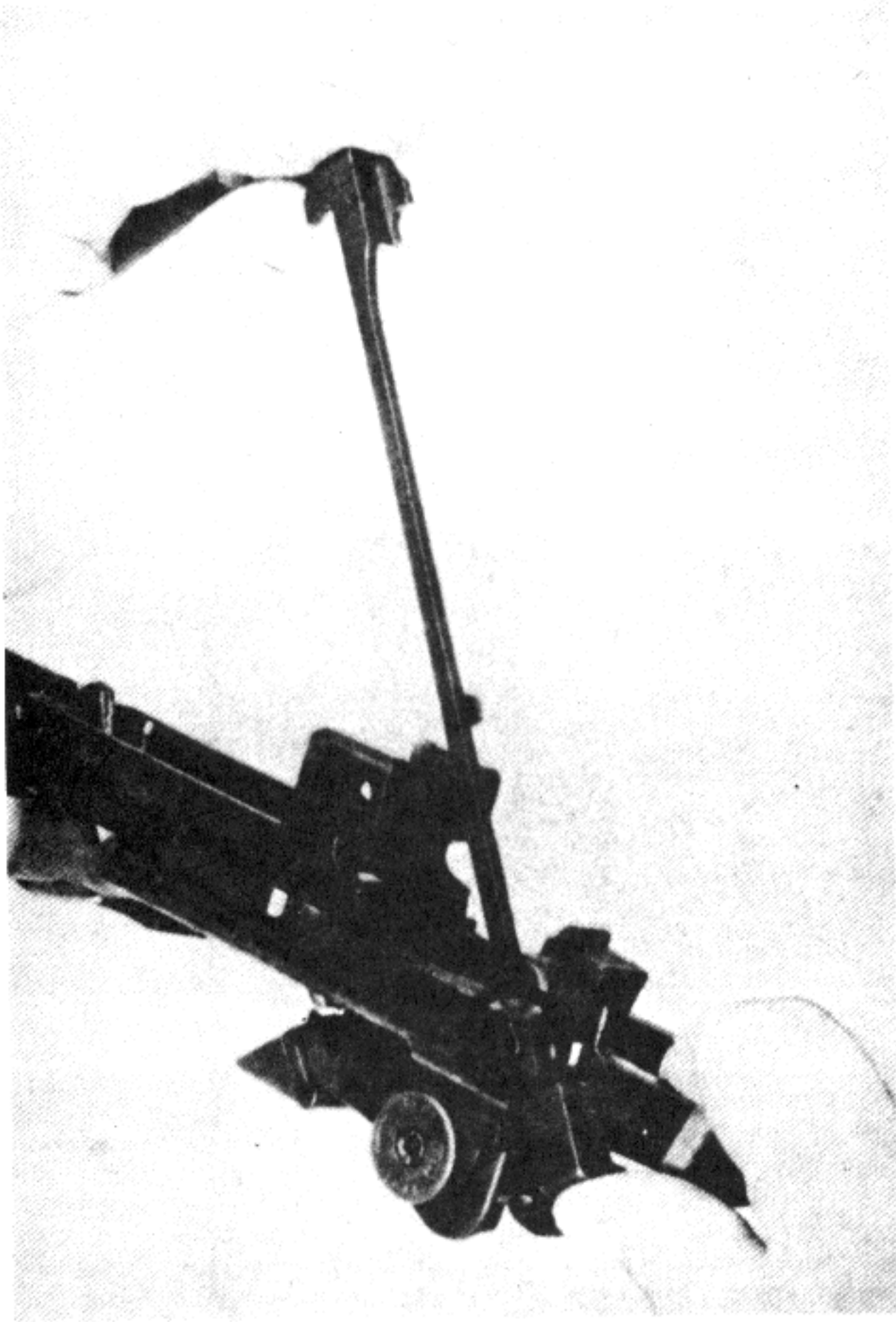
Figure 16. Replacing the connector assembly.
