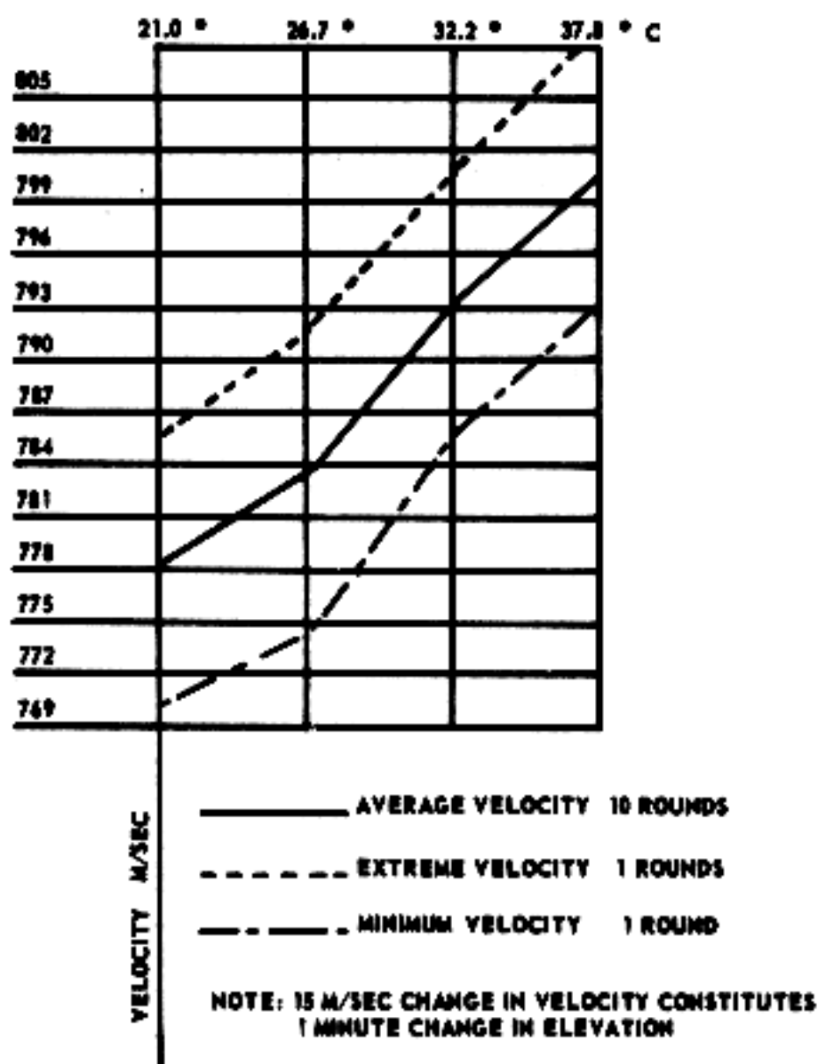
Figure 150. Temperature effects.
