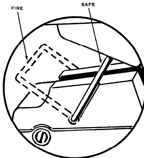
Figure 6. The M57 firing device safety bail.
