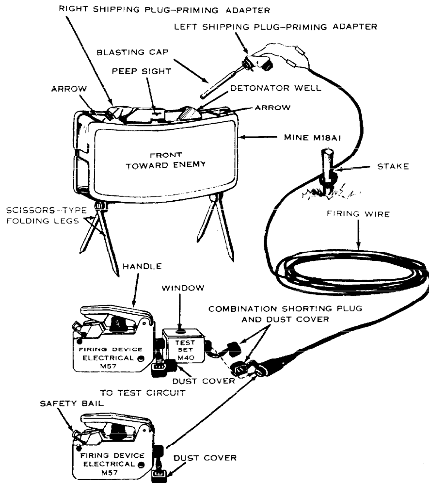
Figure 12. Arming and testing the M18A1 mine.
