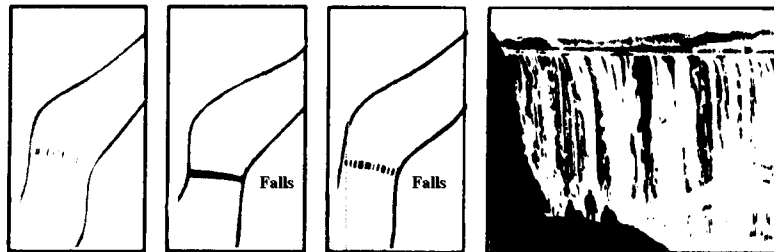
Figure 15. Large Falls.
