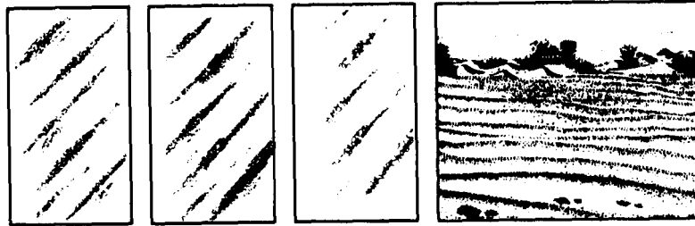
Figure 57. Lateral Dunes.
