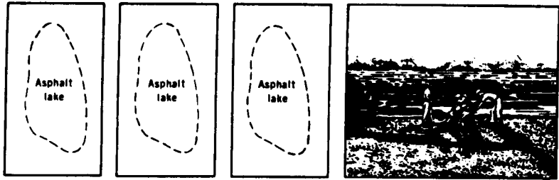
Figure 72. Asphalt Lake.
