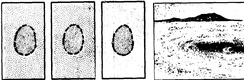
Figure 58. Wet Sand.
