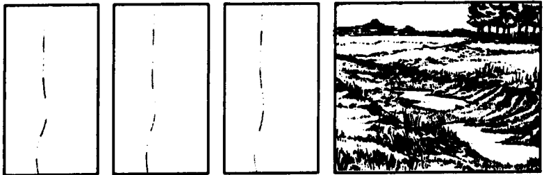
Figure 8. Intermittent Stream.
