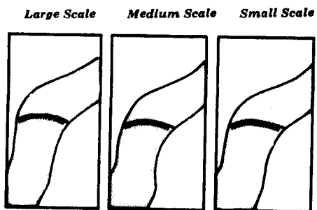
Figure 15. Large Falls.
