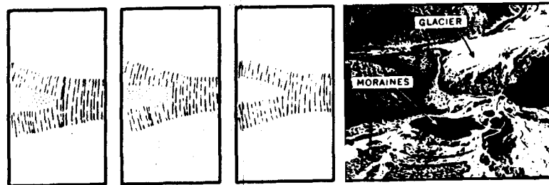
Figure 67. Glacial Moraine.
