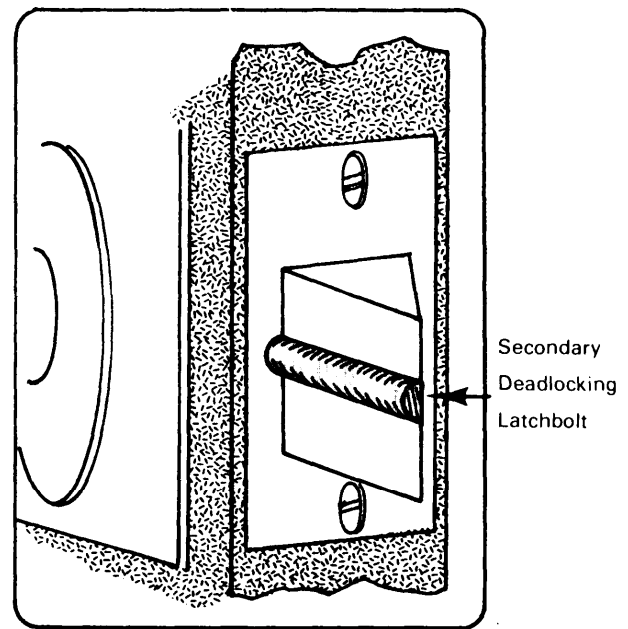
Figure 60—Secondary deadlocking latchbolt.
