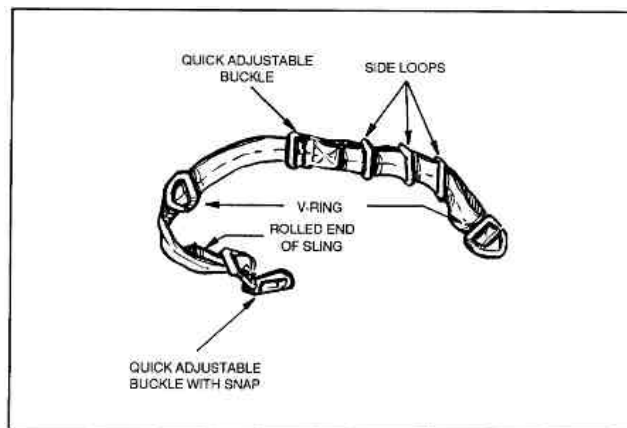
Figure 8-5. Universal load-carrying sling.
