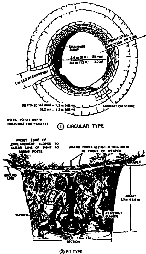
Figure 1-22. Mortar emplacements.
