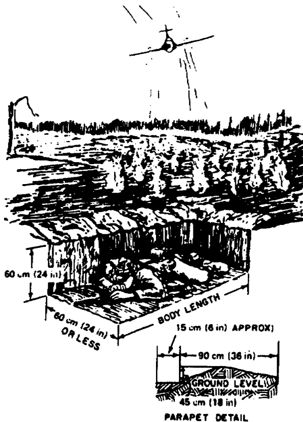
Figure 1-5. Prone emplacement.
