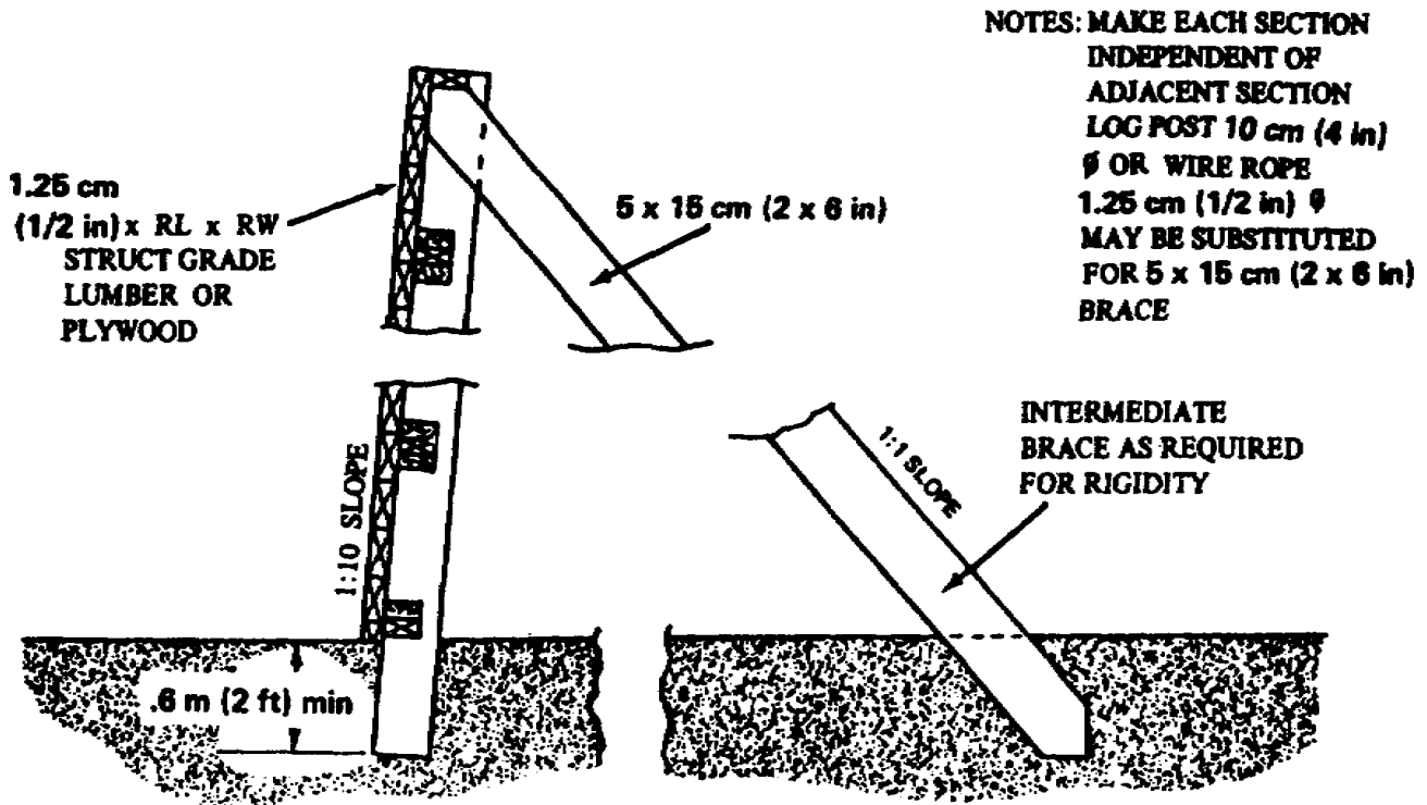
Figure 1-41. Wooden standoff.
