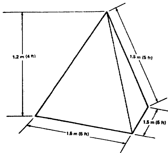
Figure 3-18. Concrete tetrahedron.
