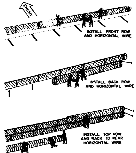
Figure 4-27. Installing concertina.
