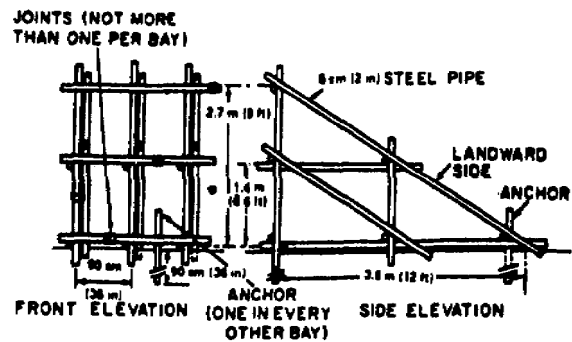
Figure 3-29. Steel scaffolding.
