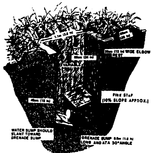
Figure 1-6. One-man foxhole.
