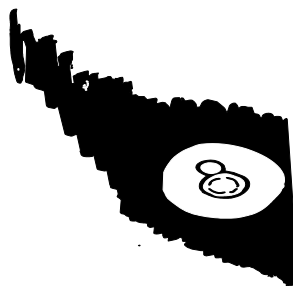
Figure 4-3. Encapsulated cells of Cryptococcus neoformans in India ink.
