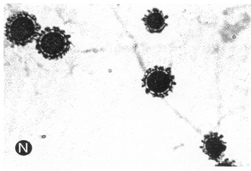
Figure 3-16. Microscopic morphology of Sepedonium species.
