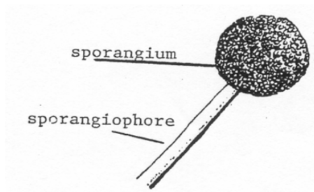
Figure 1-5. Illustration of sporangium and sporangiophore.
