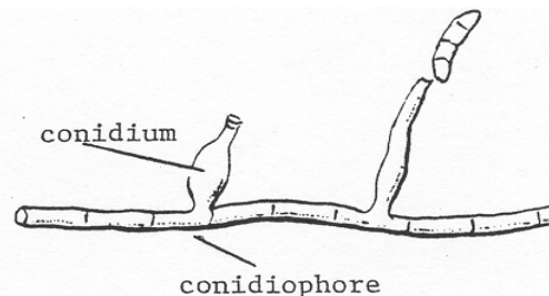
Figure 1-6. Illustration of conidia and Conidiophore.
