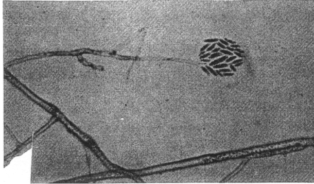
Figure 6-2. Microscopic morphology of Acremonium faliform .
