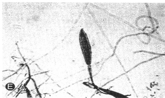
Figure 5-3. Microscopic morphology of Microsporium canis .
