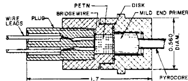
EXPLODING BRIDGEWIRE, WIRE LEAD
