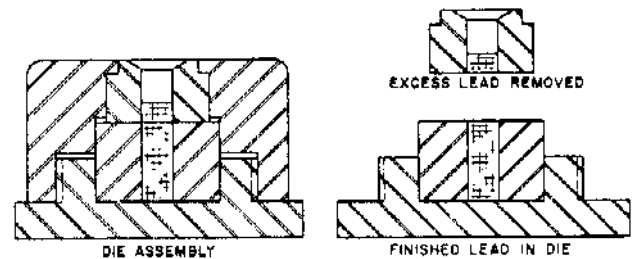
Figure 56. Explosive Loaded by Breaking off Excess
