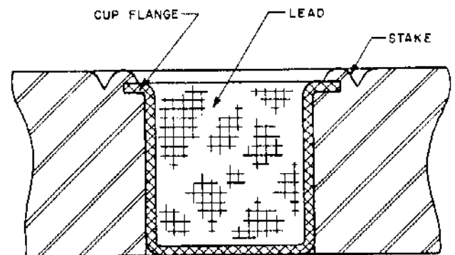
Figure 58. Lead Cup Crimped in Place
