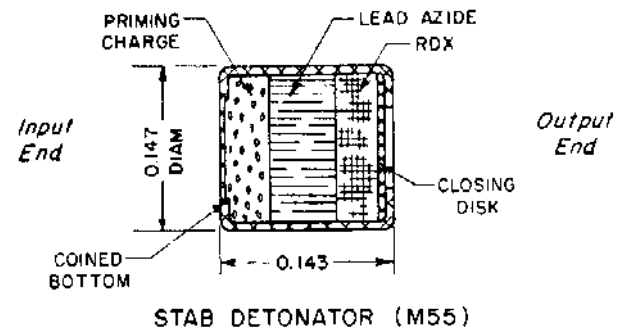
STAB DETONATOR (M55)
