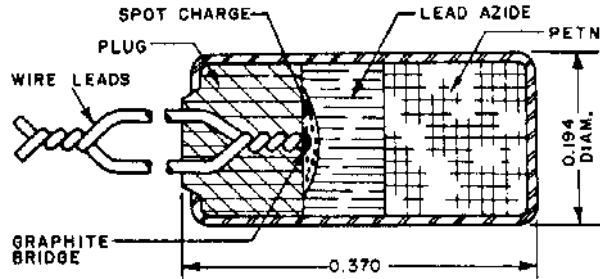
GRAPHITE BRIDGE, WIRE LEAD (M51)
