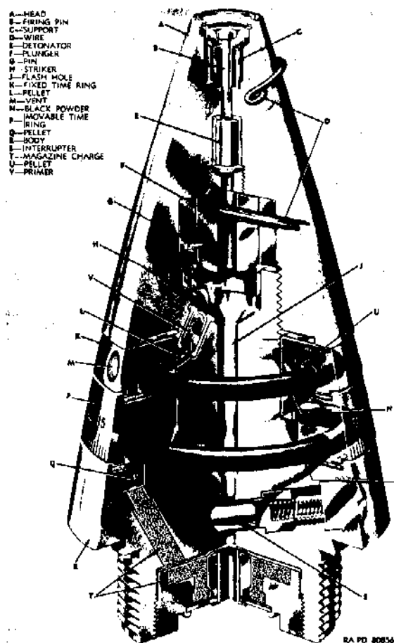
Figure 44. Fuze M54
