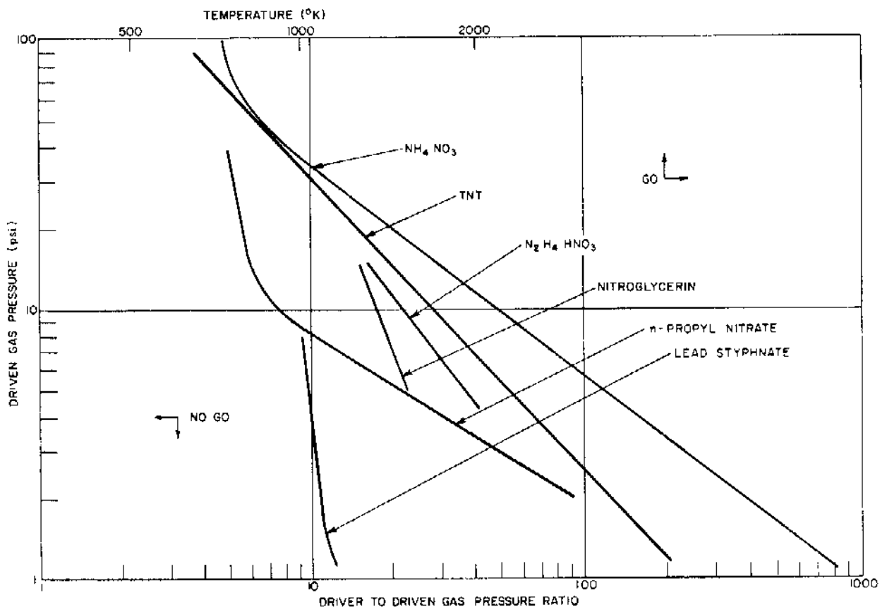
Figure 7. Threshold Conditions for Initiation of Various Explosives in a Shock Tube
