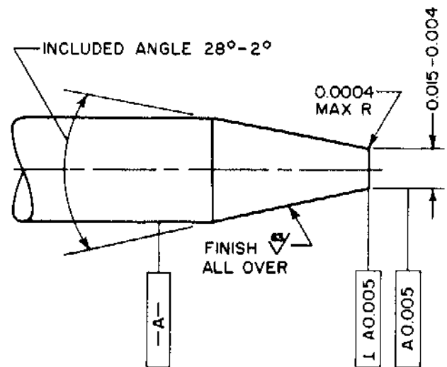
Figure 9. Standard Firing Pin for Stab Initiators
