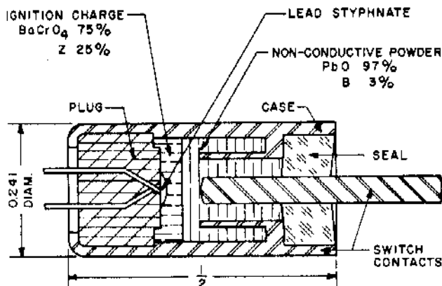
Figure 71. Pyroswitch
