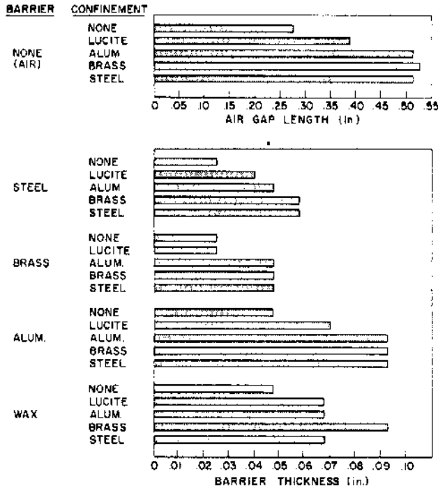
STEEL DENT OUTPUT TEST WITH Tetryl LEADS, 0.169 INCHES O.D. TUBE DETONATORS IN GROUPS OF 30. MINIMUM DENT FOR HIGH ORDER DETONATION IS 0.015 INCHES
