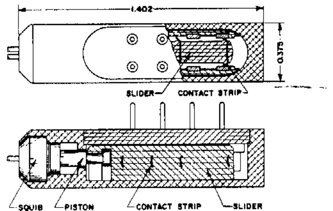
Figure 70. Multiple Contact Switch
