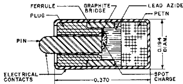
GRAPHITE BRIDGE, BUTTON (T77)
