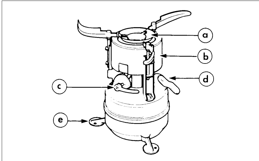
Figure 2-7 Stove M 1950
