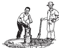
Place reinforcing wire and a mold for the hole.
