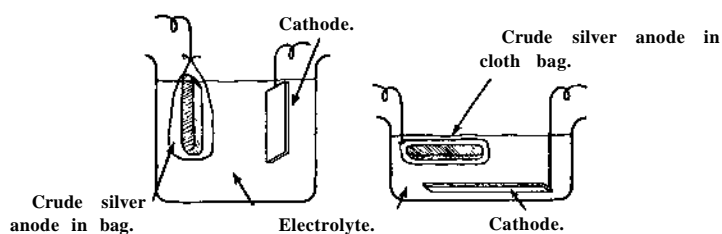
Silver cells at start of electrolytic refining. The Moebius or vertical arrangement is shown on the left, and the horizontal Thum or Balbach-Thum arrangement is shown on the right.
