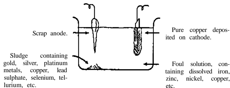
Copper cell at end of electrolytic refining.
