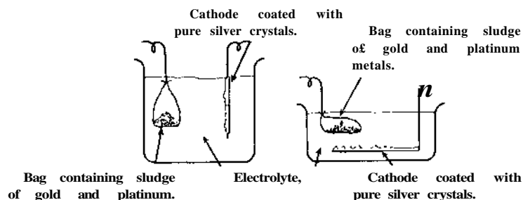
Silver cells at end of electrolytic refining. The Moebius arrangement is to the left, the Thum or Balbach-Thum arrangement is to the right.
