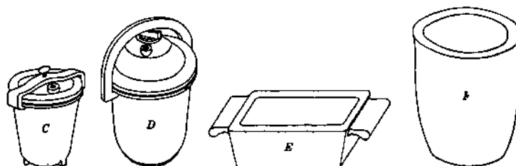
Apparatus for retorting amalgams A, set up of small retort with condenser, B, water sealed vapor trap, C one style of retort, D, Nevada type retort, E, bullion mold, F, graphite crucible
