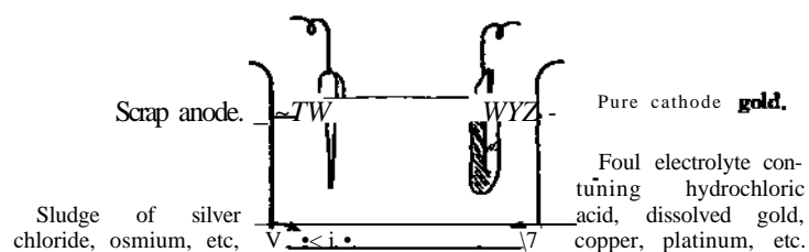
Gold cell at end of Wohlwill electrolytic refining.
