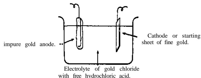
Gold eel! at start of electrolytic refining by the Wohlwill process.
