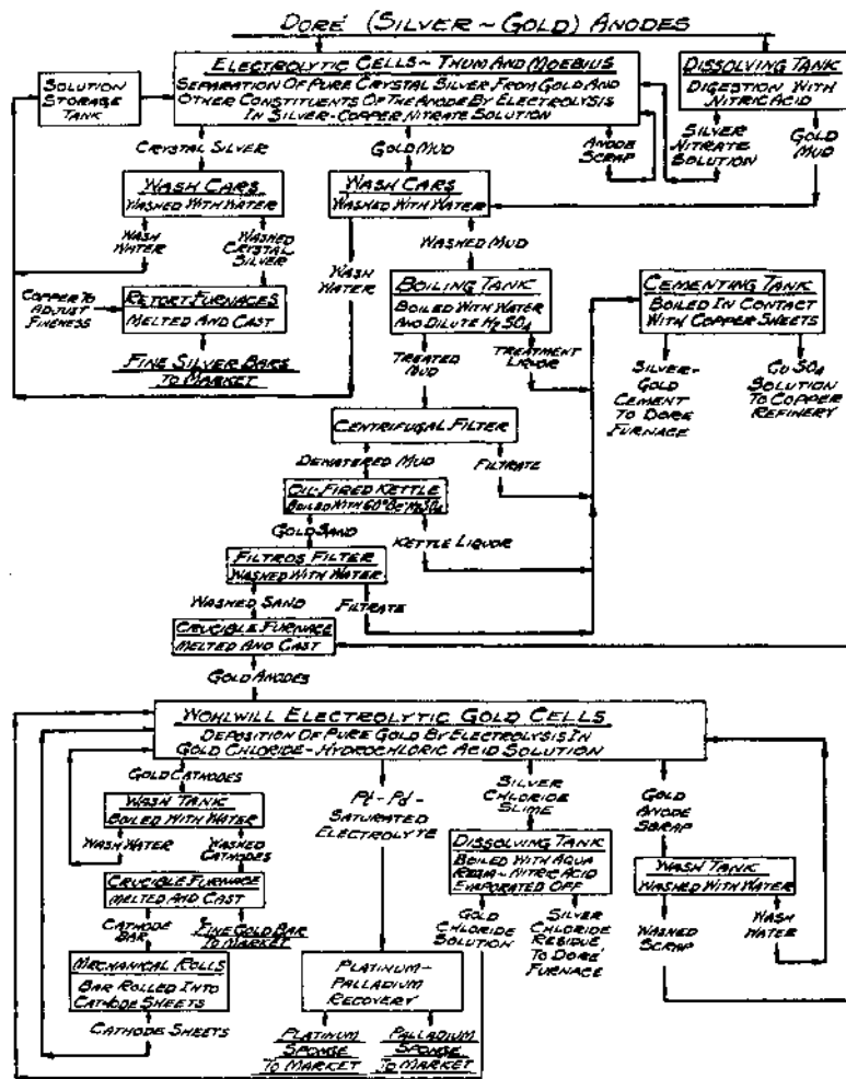
Flow sheet of electrolytic refining of precious metals at the Ranun Copper Works.
