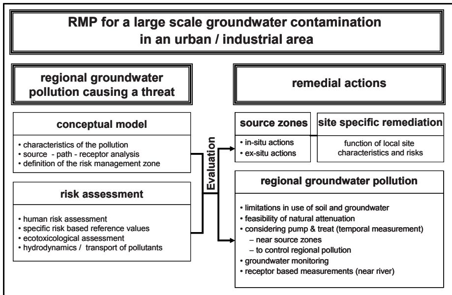
Figure 9. Schematic overview of the RMP proposed for the polluted area at Vilvoorde – Machelen
