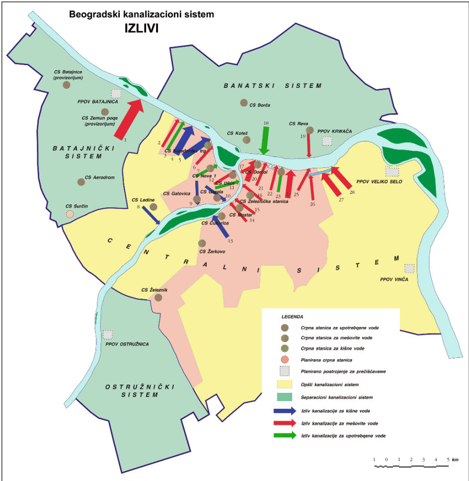
Figure 4. Major sewer system discharges to Sava and Danube
