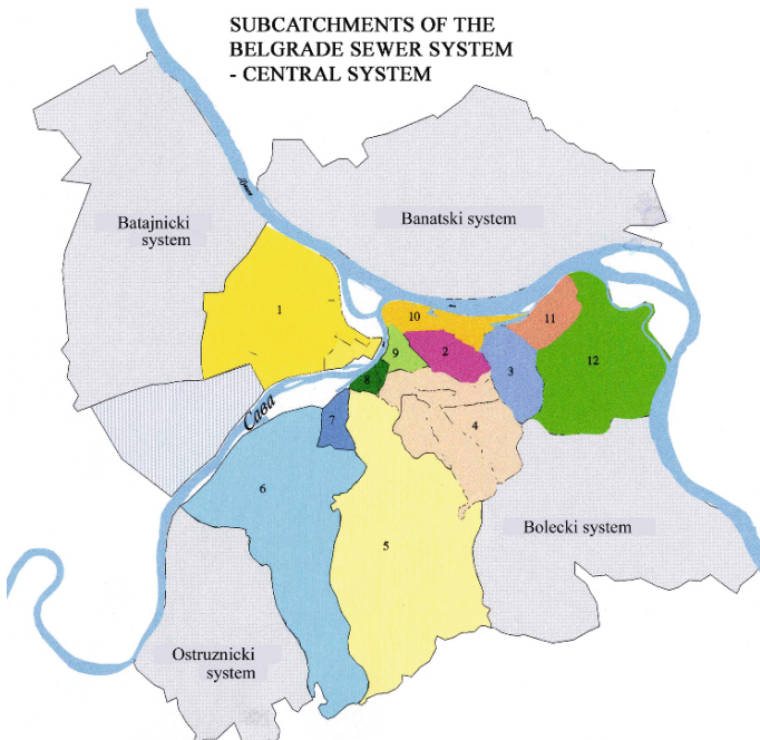
Figure 2. Subsystems of the central sewer system of Belgrade
