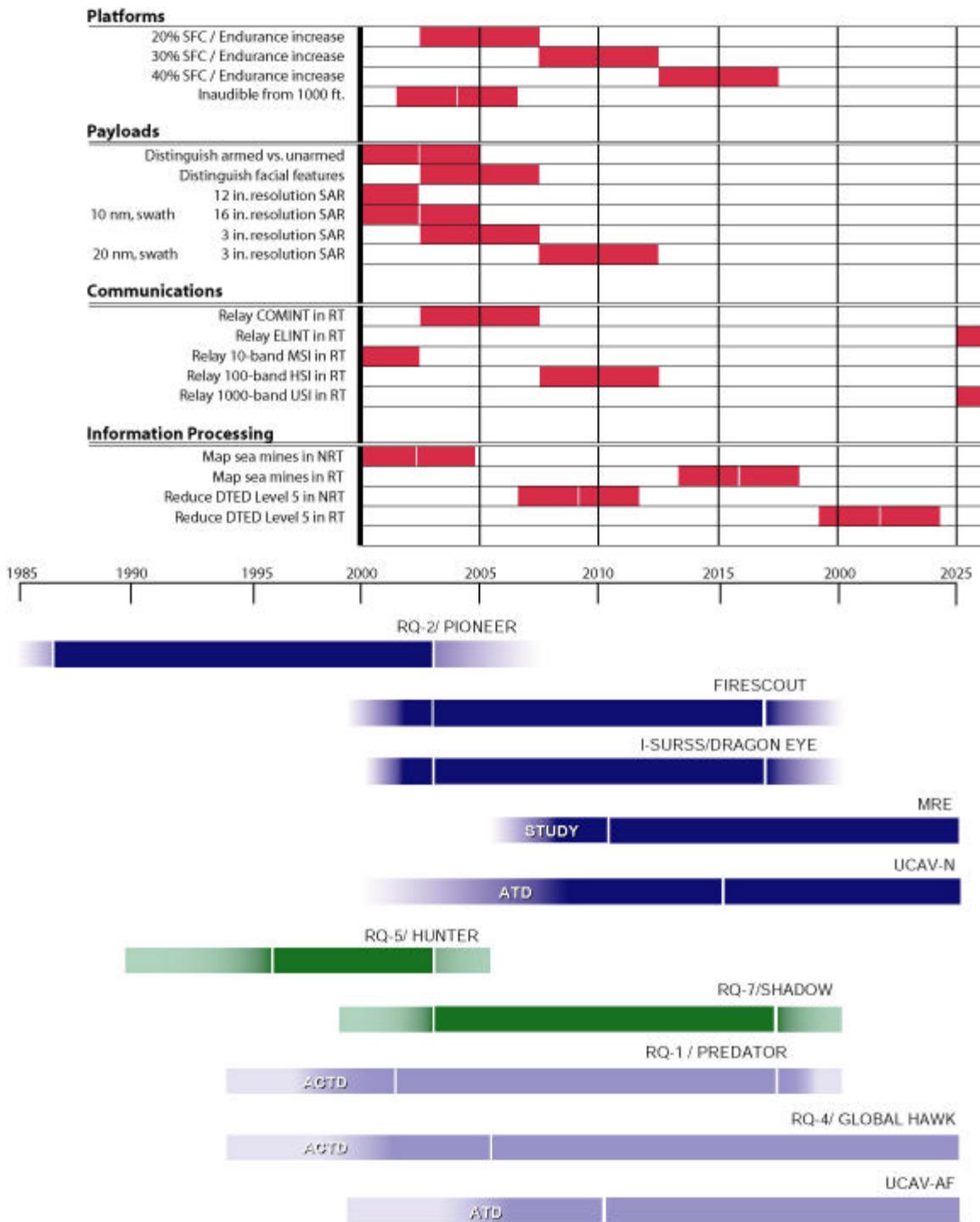
FIGURE 6.2-1: UAV ROADMAP, 2000-2025.
