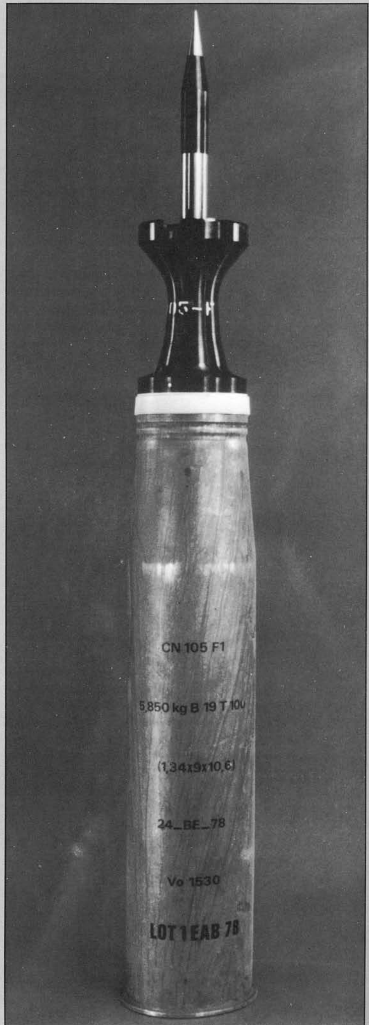
Right: Not small arms by any means, but an example of where the discarding sabot principle is at its best; this is a French fin-stabilized discarding sabot shot for a 105mm tank cannon.
