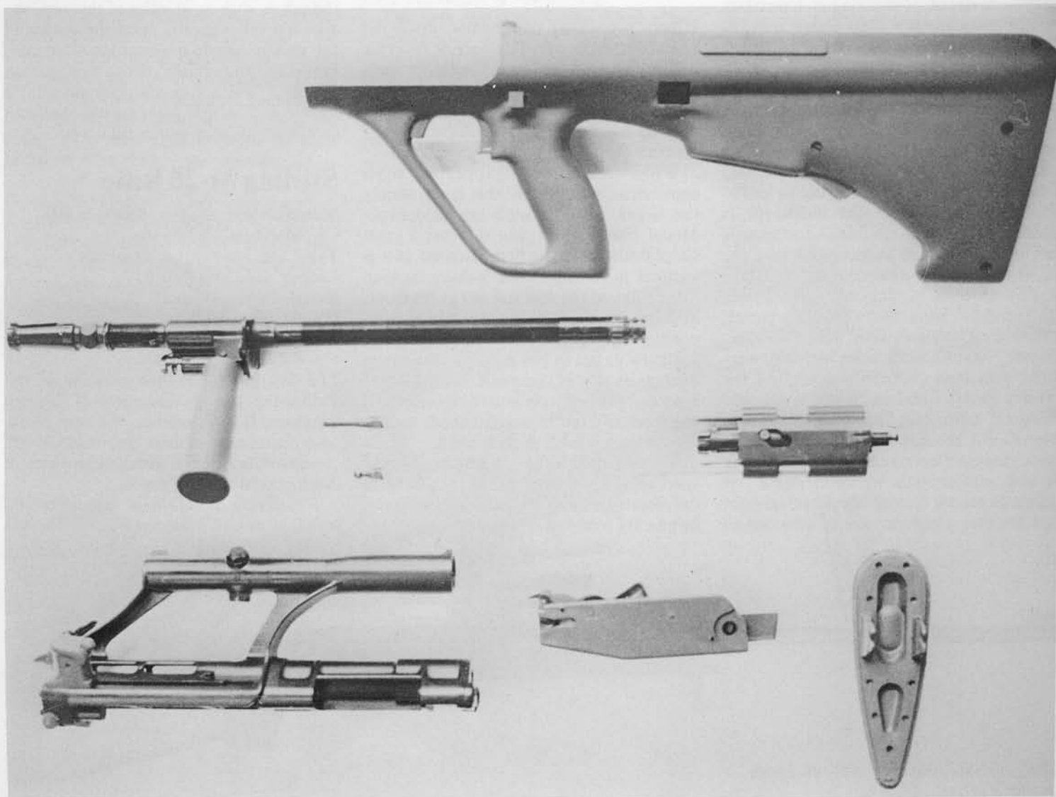
Above: The Steyr AUG with alternative barrels; from top to bottom, the squad machine gun, rifle, carbine and submachine gun barrels. Below: The Steyr AUG field-stripped.
