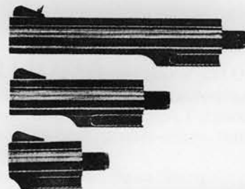
Dan Wesson's 'Pistol Pac', showing the alternative barrels which can be rapidly fitted to the basic frame.
