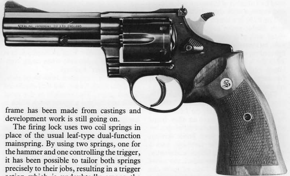
The Sterling .357 Magnum revolver, a new departure for the company and the first new revolver in Britain for almost sixty years.
