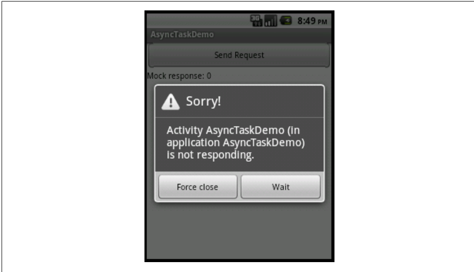
Figure 6-2. Unresponsive application
