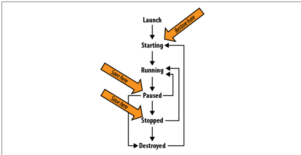
Figure 3-5. Activity life cycle states
