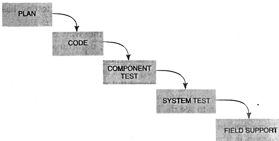
Fig. 19.1 Waterfall model of software construction
