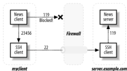
Figure 3-2. Tunneling NNTP with SSH
