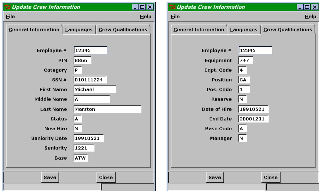
Figure 8.10 Notebooks
