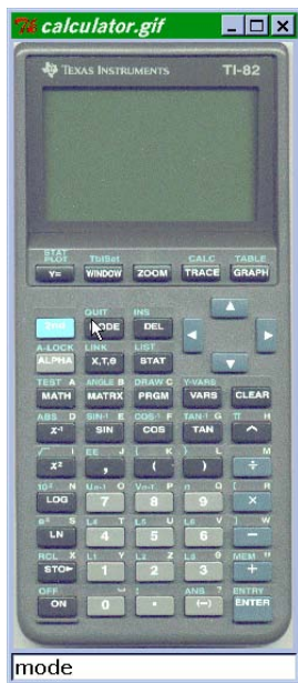
Figure 8.16 Running calculator.py
