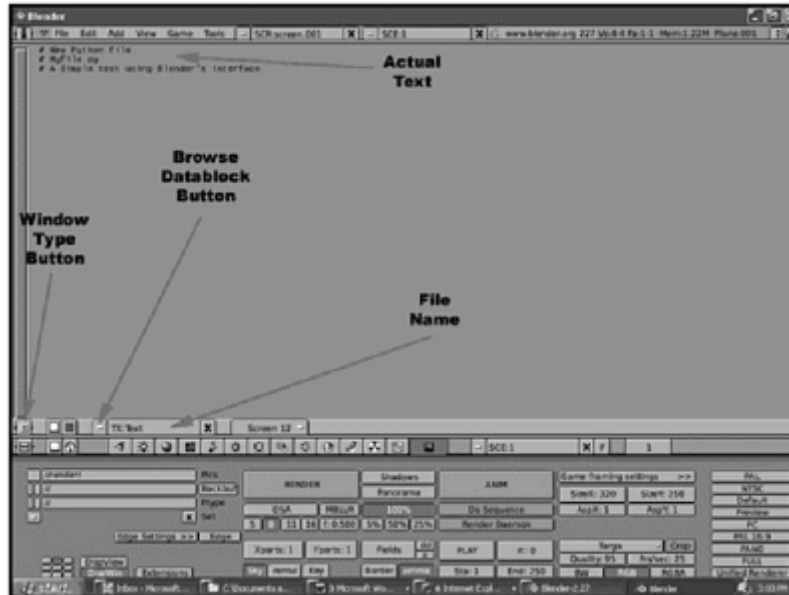
Figure 5.8. Highlighted text controls in Blender
