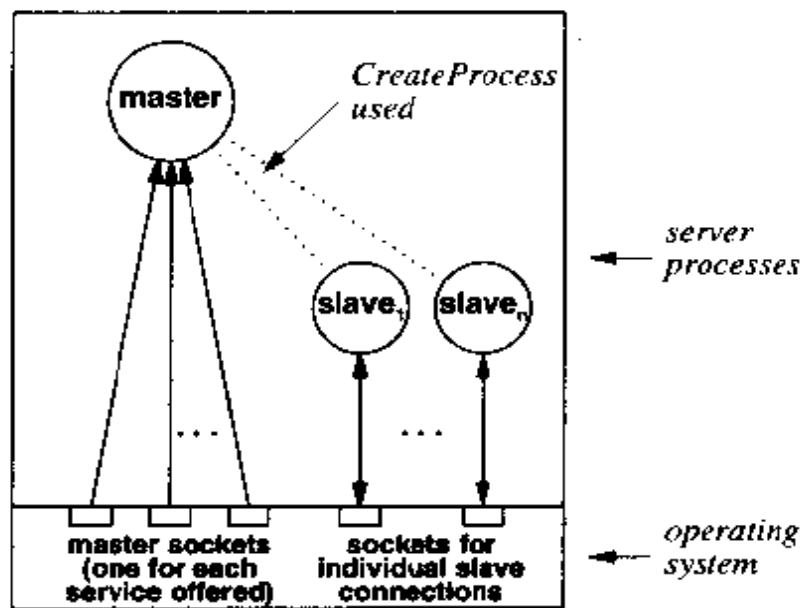
Figure 14.4 The structure of a connection-oriented, multiservice server that uses CreateProcess to execute a separate program to handle each connection.
