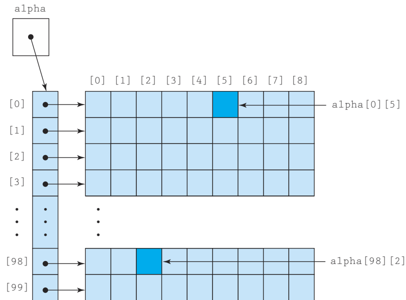
Figure 2.12 Java implementation of the alpha array
