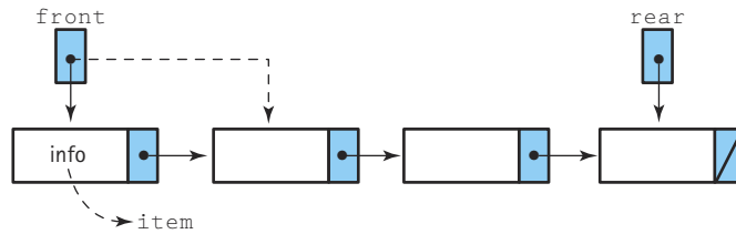
Figure 5.12 The dequeue operation
