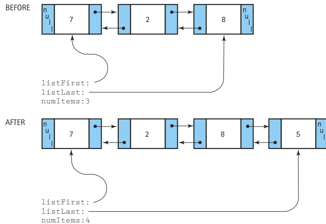
Figure 6.17 Inserting at the front and at the end
