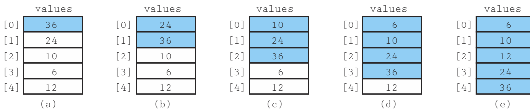
Figure 10.5 Example of the insertion sort algorithm
