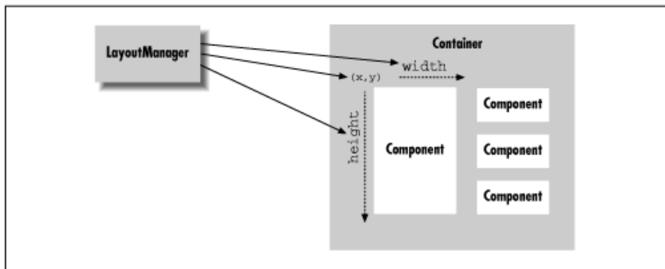
Figure 12.1: LayoutManager at work
