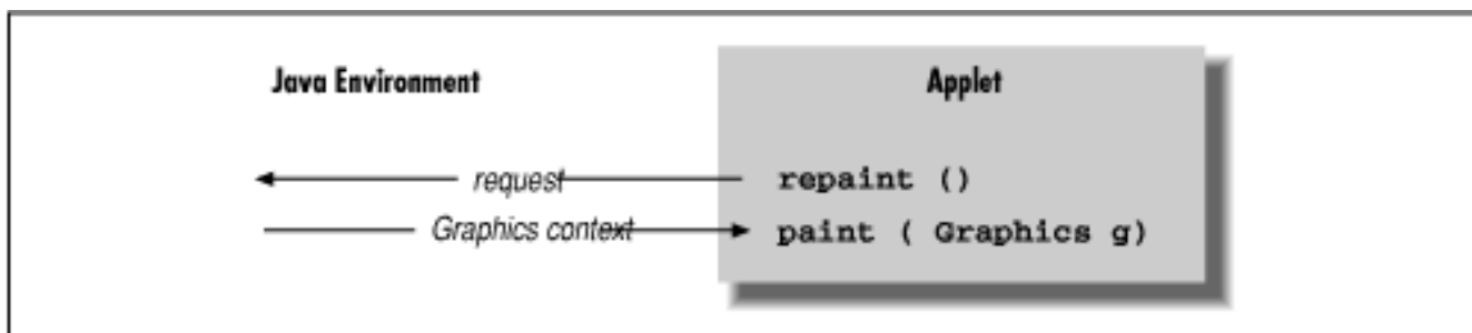
Figure 2.5: Invoking the repaint() method
