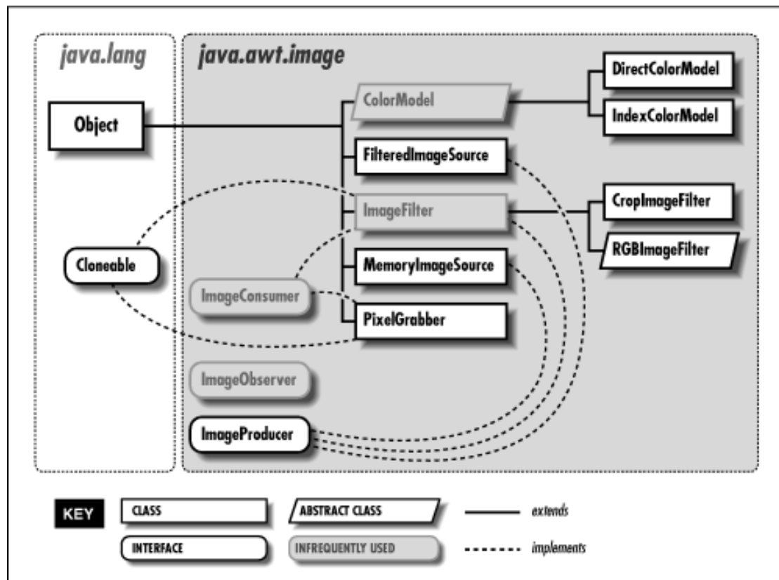
Figure 14.1: The java.awt.image package
