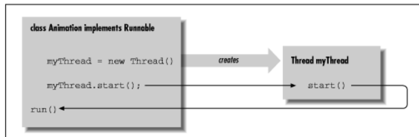
Figure 6.1: Interaction between Animation and its Thread
