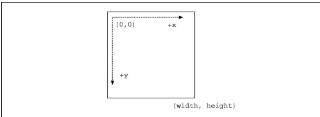
Figure 13.2: Graphics coordinate system
