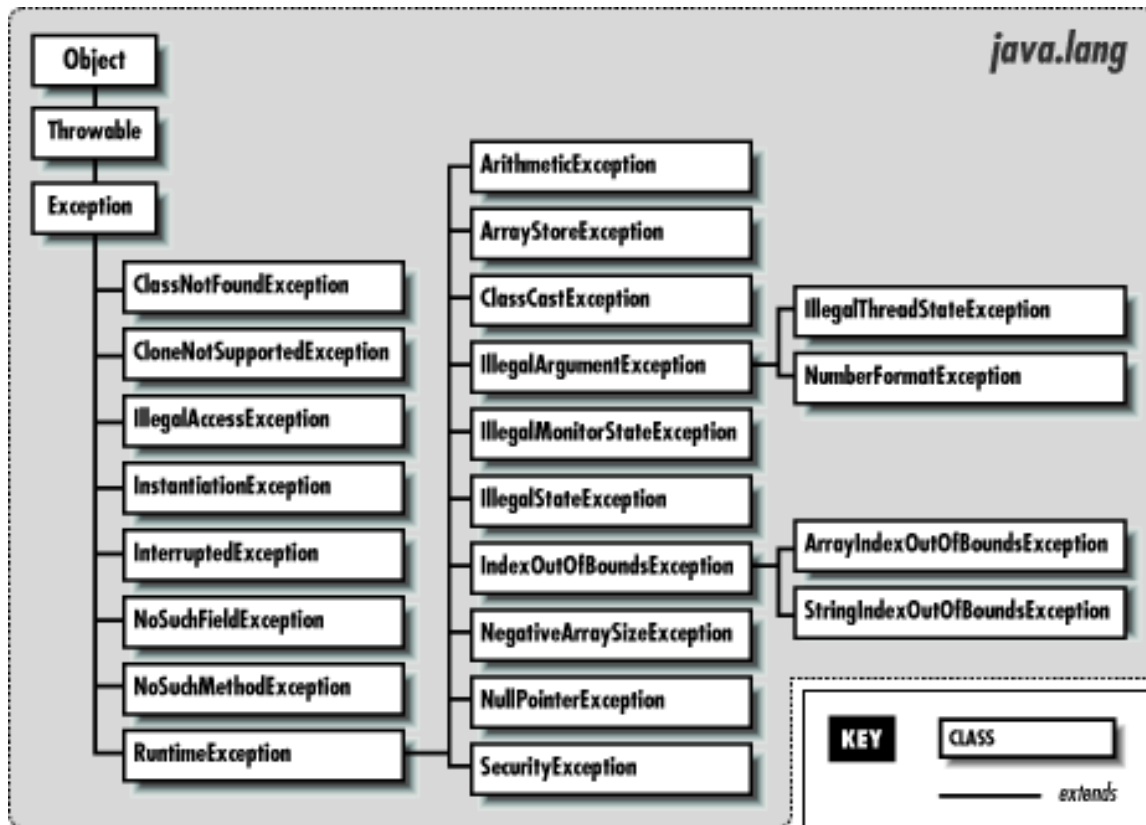
Figure 25.3: The error classes in the java.lang package
