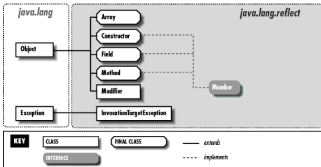
Figure 26.1: The java.lang.reflect package
