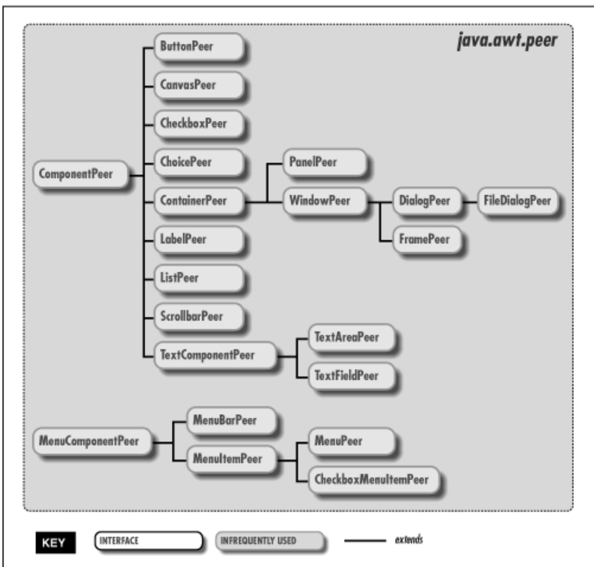
Figure 10.3: The java.awt.peer package
