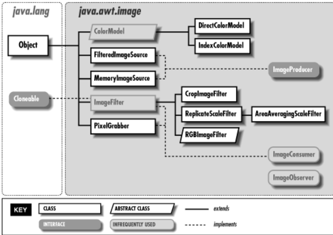
Figure 18.4: The java.awt.datatransfer package
