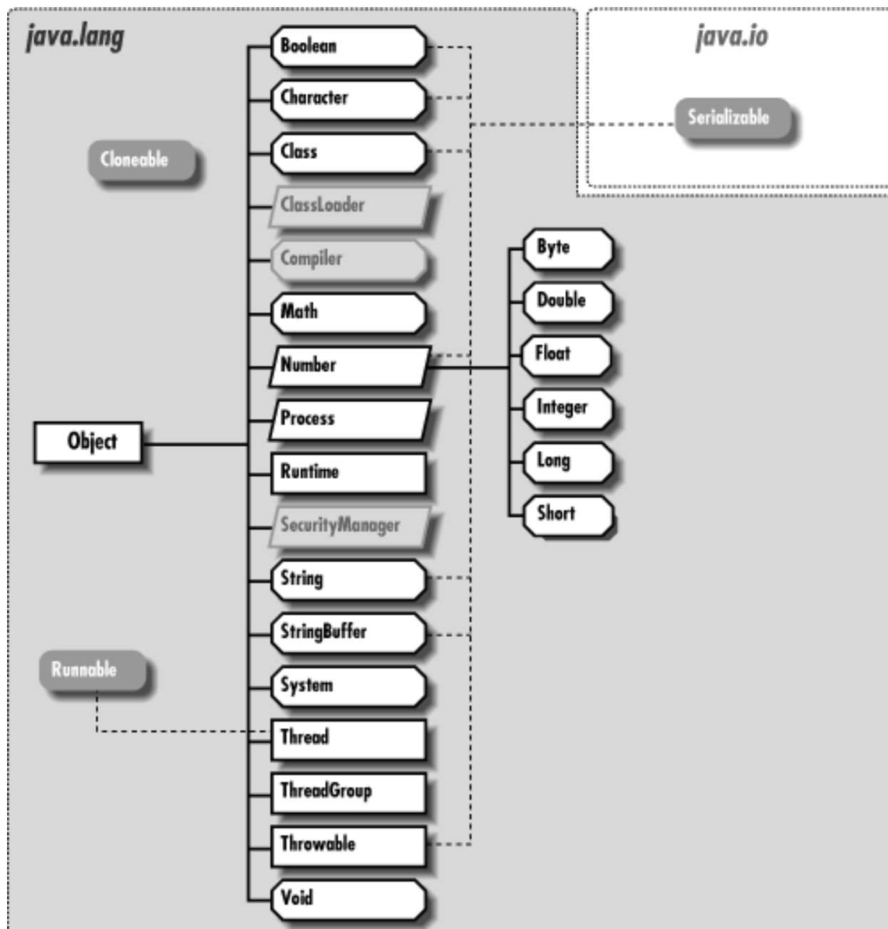
Figure 12.1: The java.lang package
