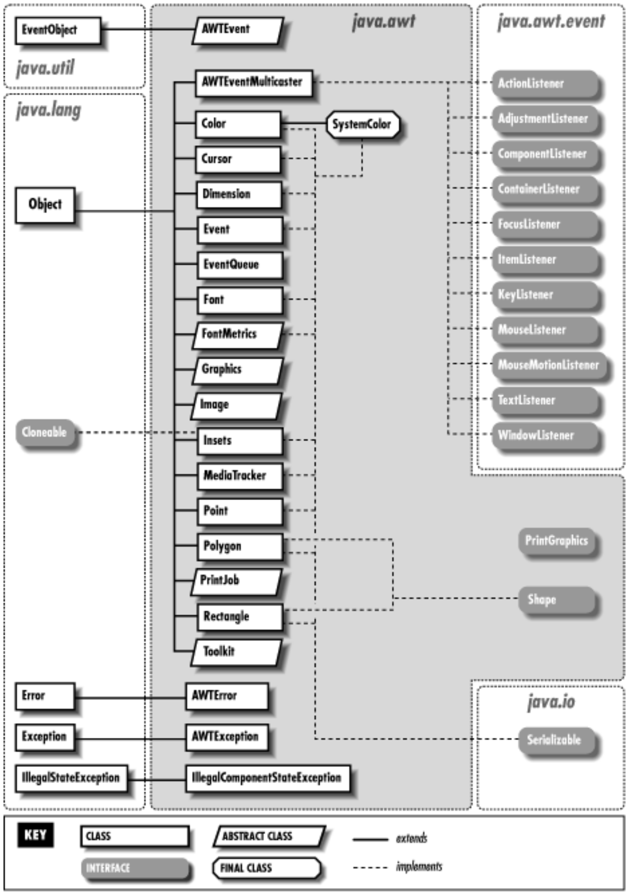
Figure 18.1: Graphics, event, and exception classes of the java.awt package
