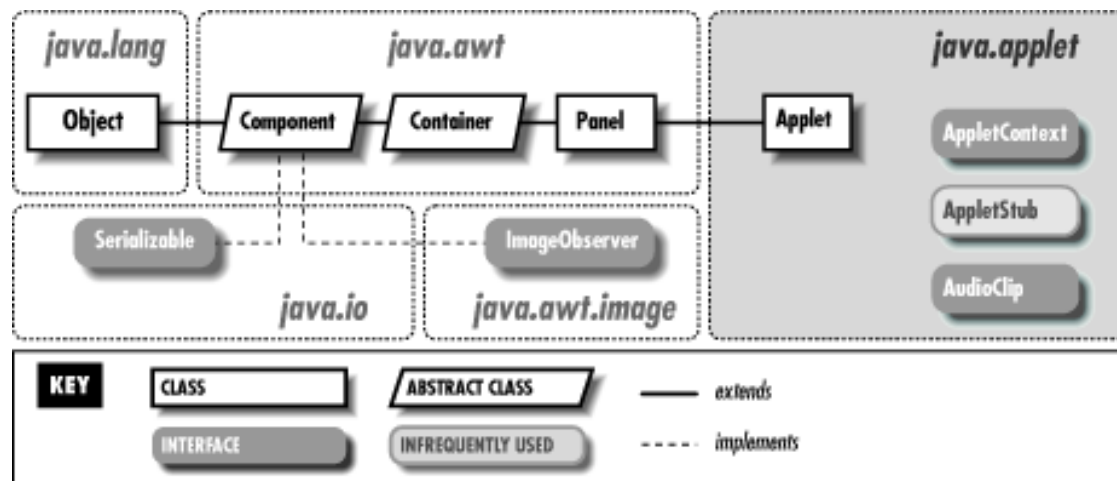
Figure 17.1: The java.applet package
