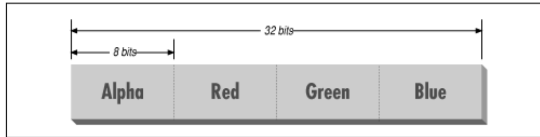
Figure 14.3: ARGB color encoding
