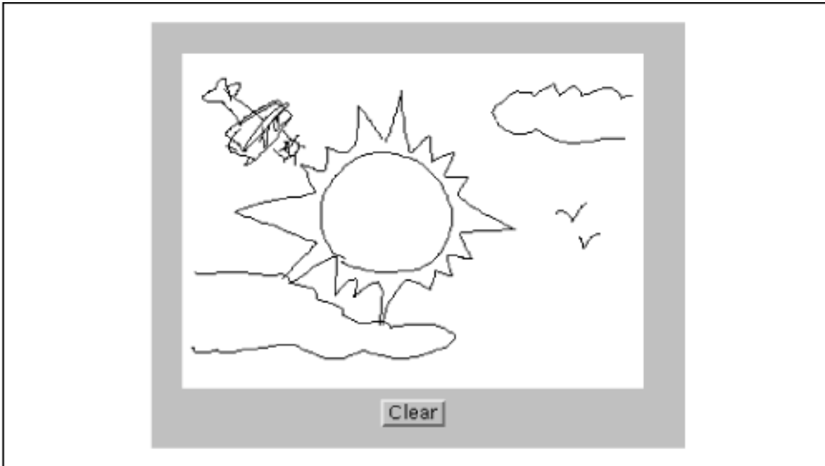
Figure 11.8: The ComponentScrollerApplet
