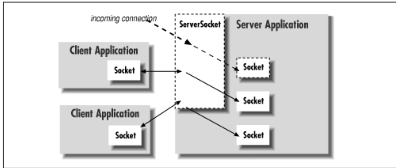
Figure 9.2: Clients and servers, Sockets and ServerSockets
