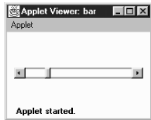
Figure 11.1: Scrollbar elements
