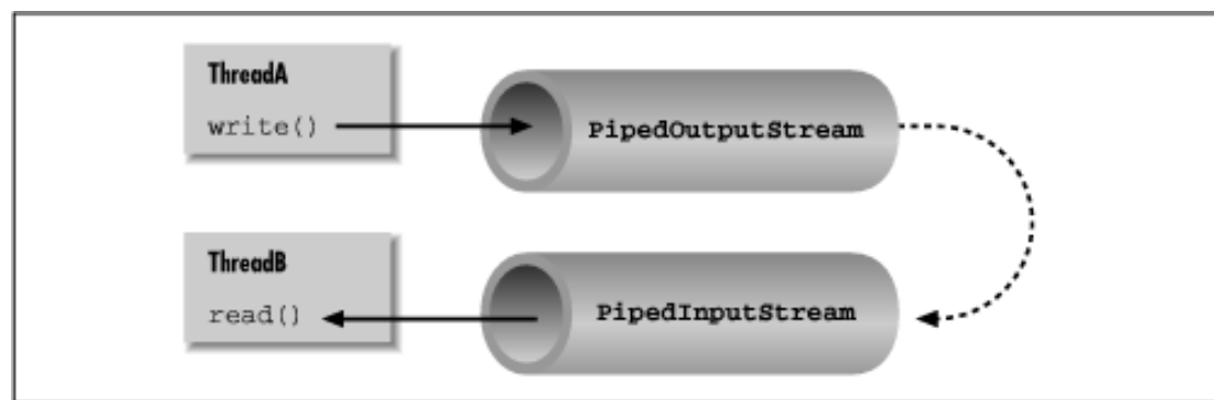
Figure 8.4: Piped streams
