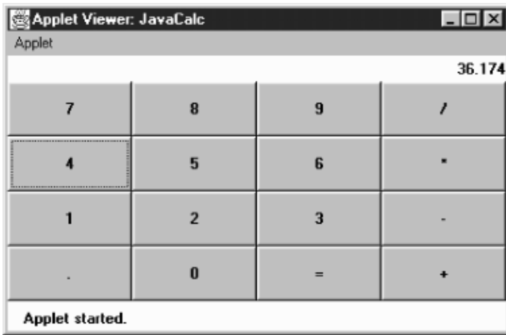
Figure 5.4: Calculator applet
