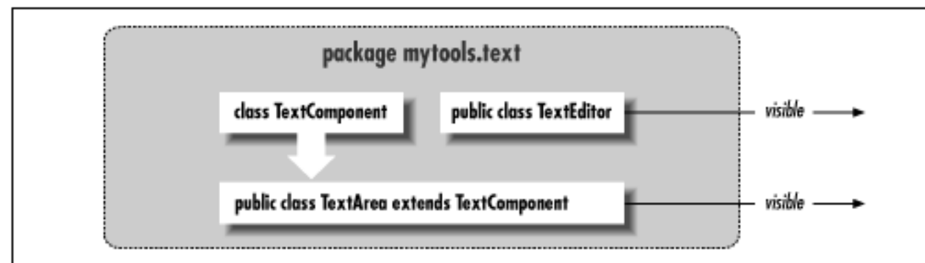
Figure 5.7: Class visibility and packages
