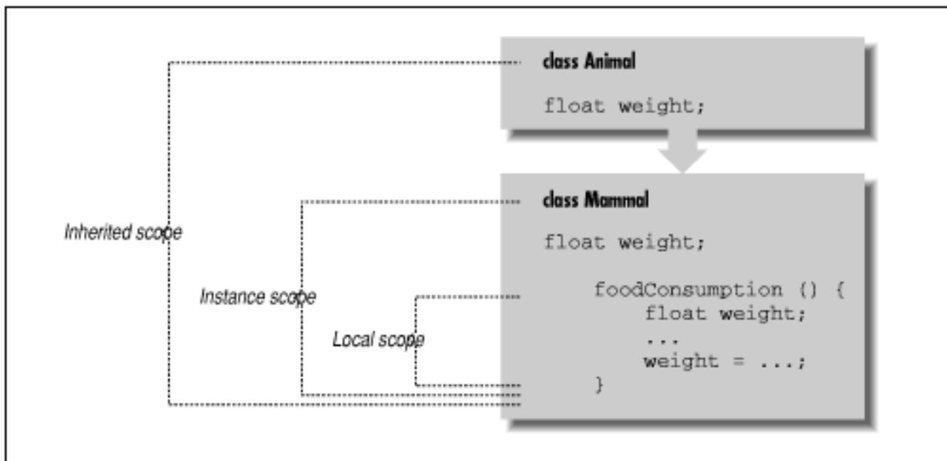
Figure 5.4: The scope of shadowed variables
