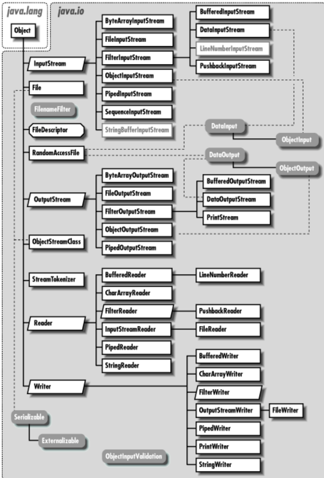
Figure 24.1: The java.io package
