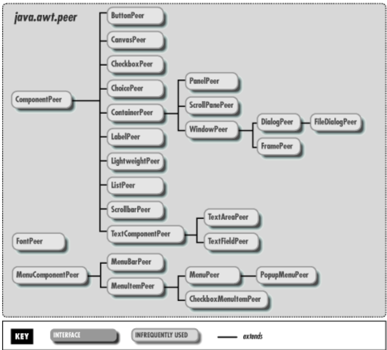
Figure 22.1: The java.awt.peer package
