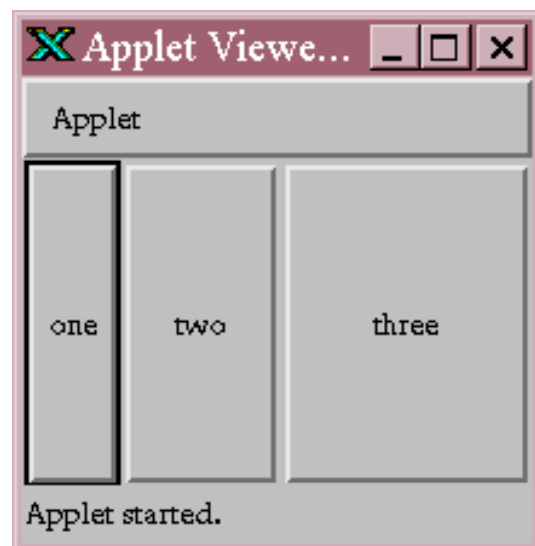
Figure 12.8: Varied weightx
