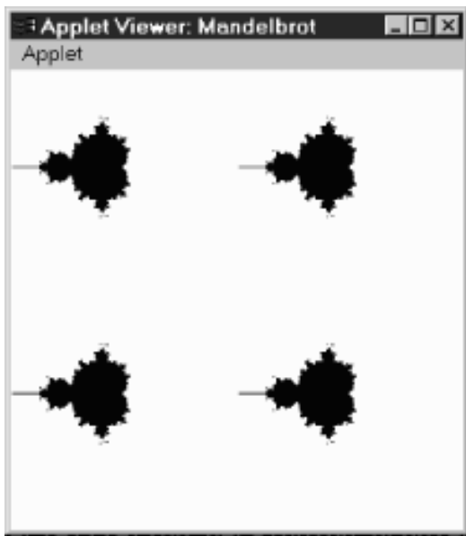
Figure 12.3: Mandelbrot output
