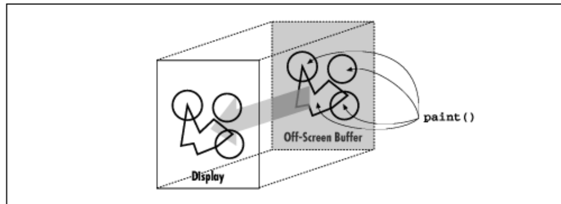
Figure 13.8: Double buffering
