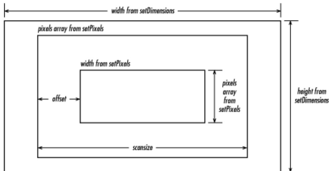
Figure 12.5: Storing pixels in an array
