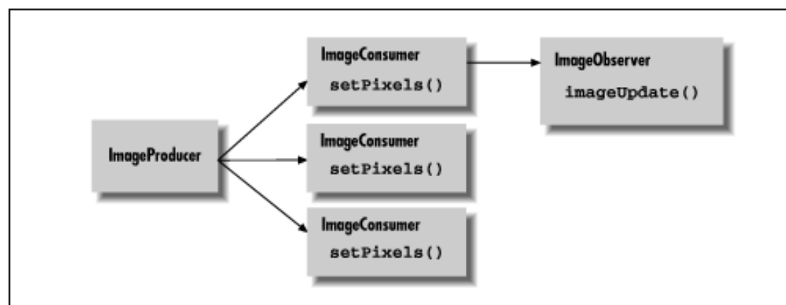
Figure 14.2: Image observers, producers, and consumers
