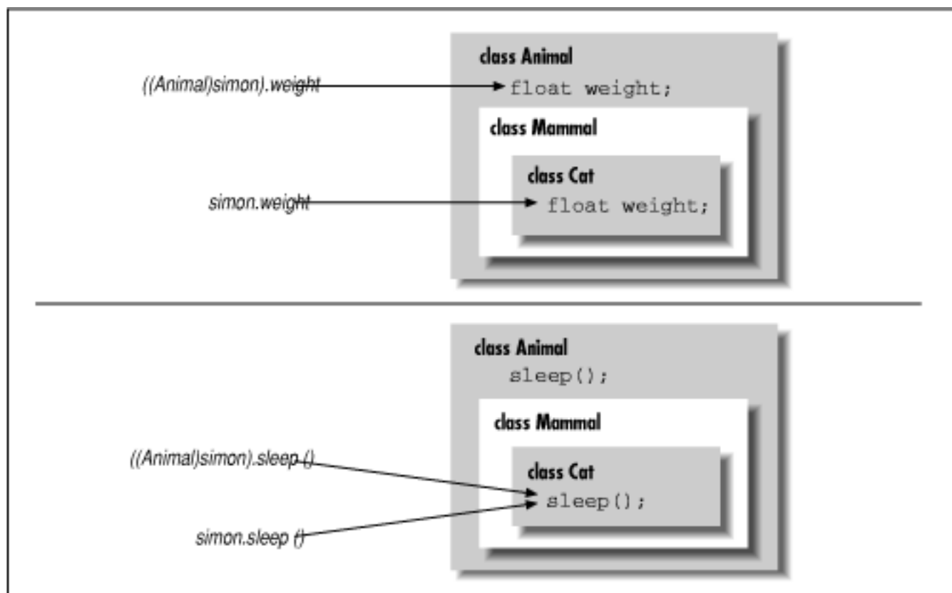
Figure 5.6: Casting and its effect on method and variable selection
