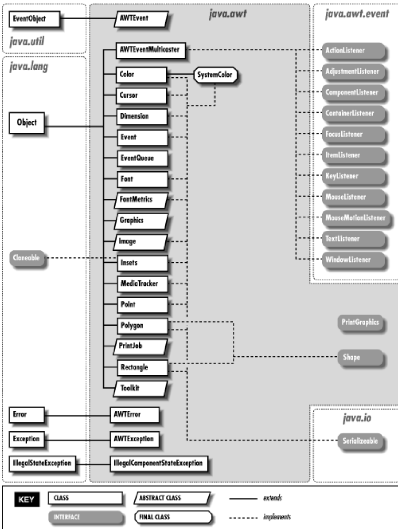
Figure 18.3: The java.awt.image package
