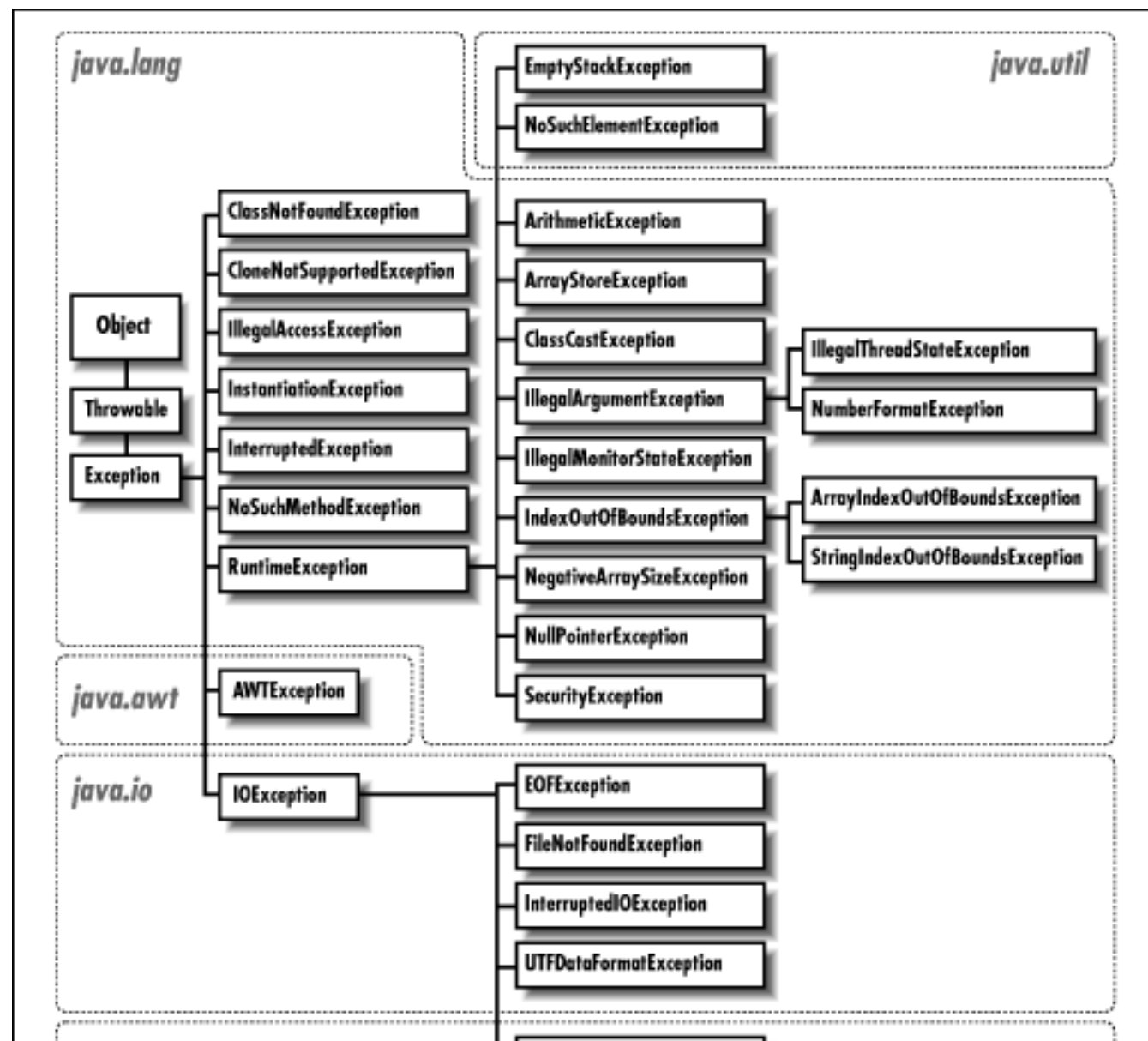
Figure 4.1: Java exception classes
