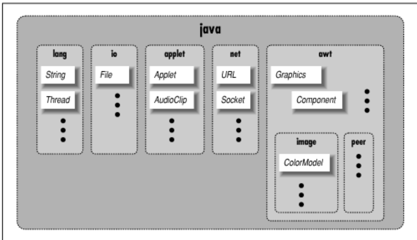
Figure 2.4: The core Java packages
