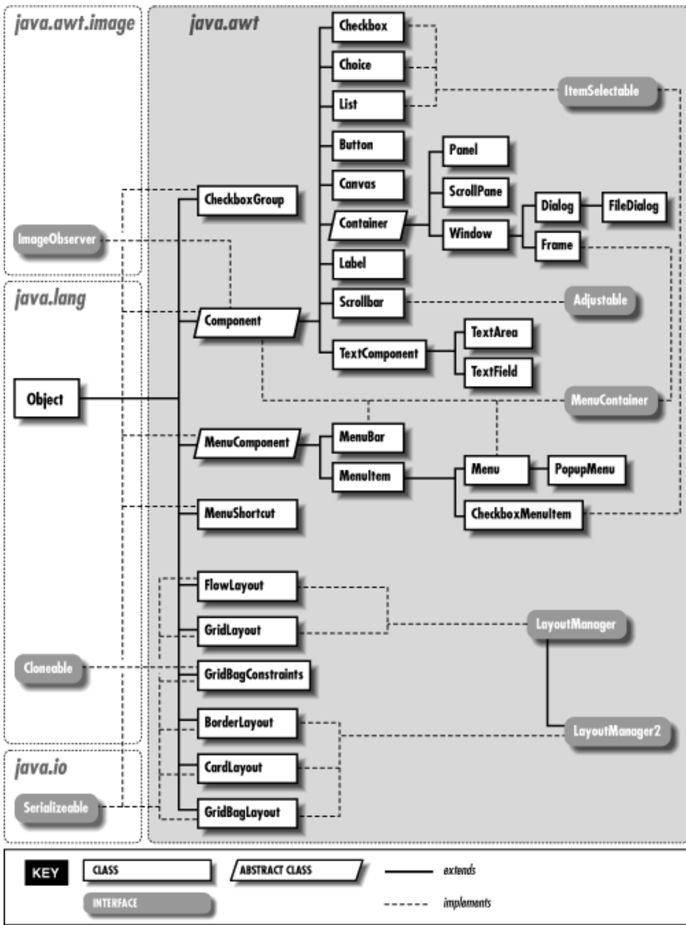
Figure 18.2: Graphics classes of java.awt package
