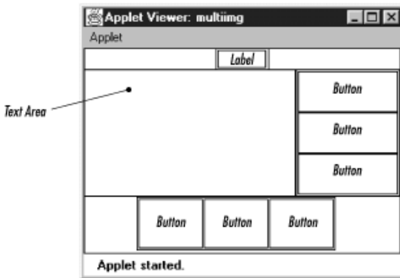
Figure 1.15: Components within containers
