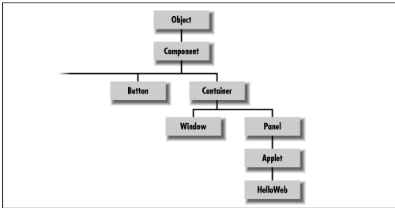
Figure 2.3: Part of the Java class hierarchy
