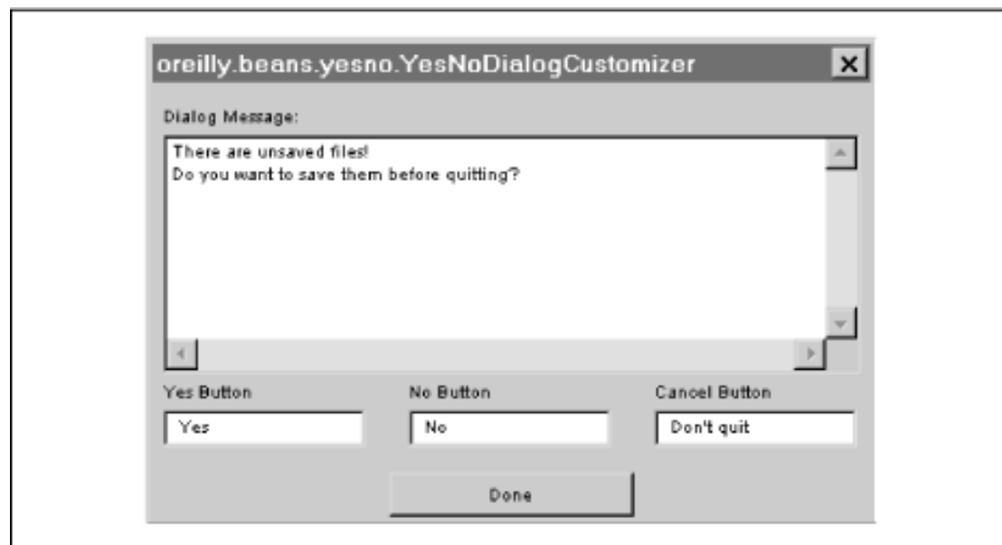
Example 10.8: The YesNoDialogCustomizer Class
