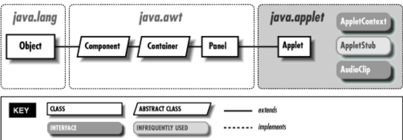
Figure 18.7: The java.applet package
