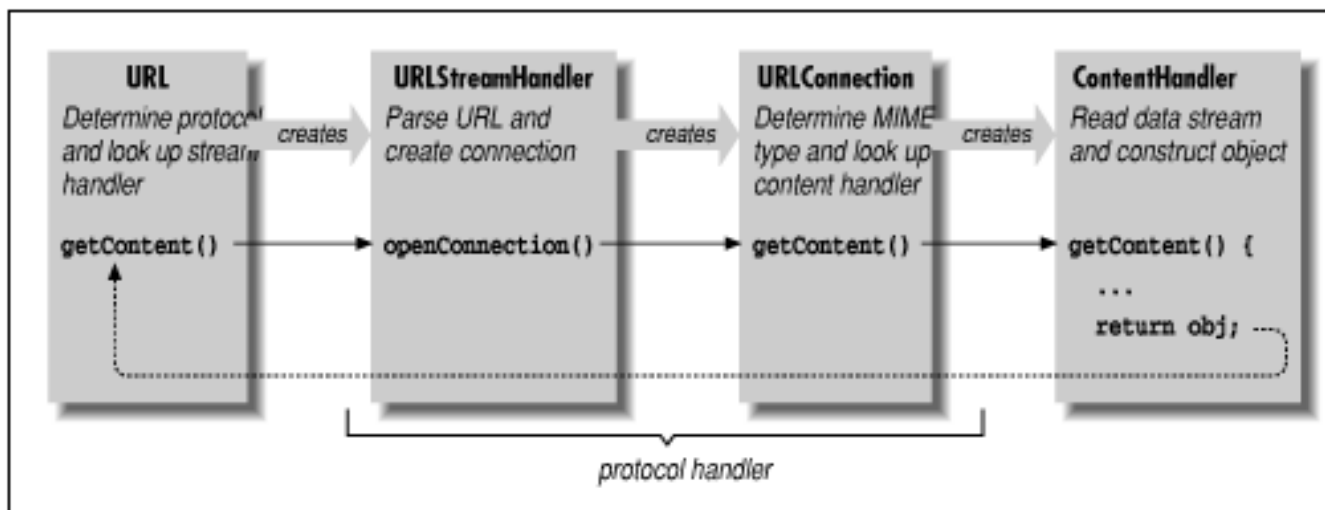
Figure 9.5: The protocol handler machinery
