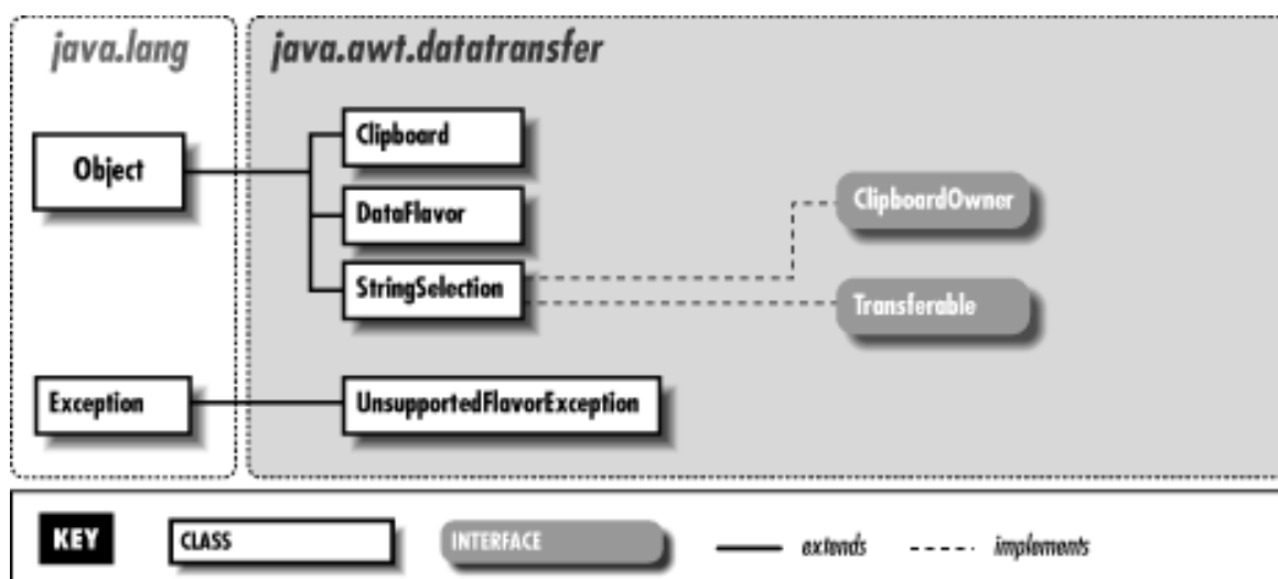
Figure 19.1: The java.awt.datatransfer package
