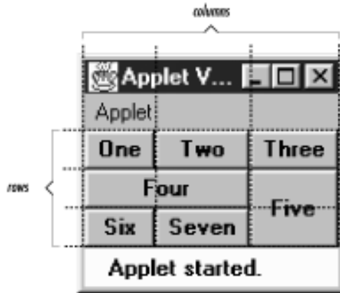
Figure 7.10: How GridBagConstraints counts rows and columns
