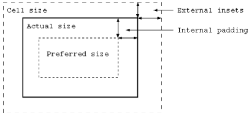
Figure 12.11: Another Layout Using Padding and Insets
