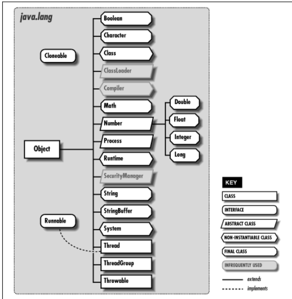
Figure 7.1: The java.lang package
