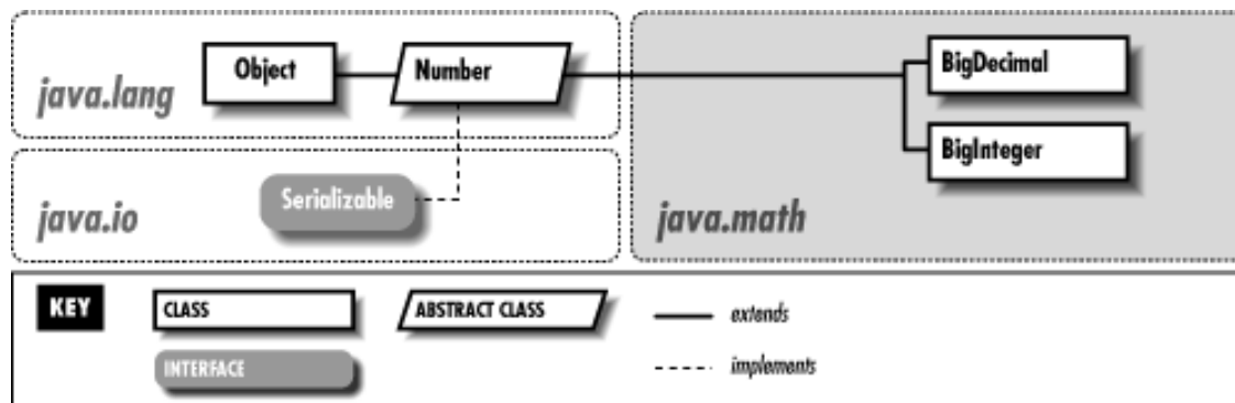
Figure 14.1: The java.math package
