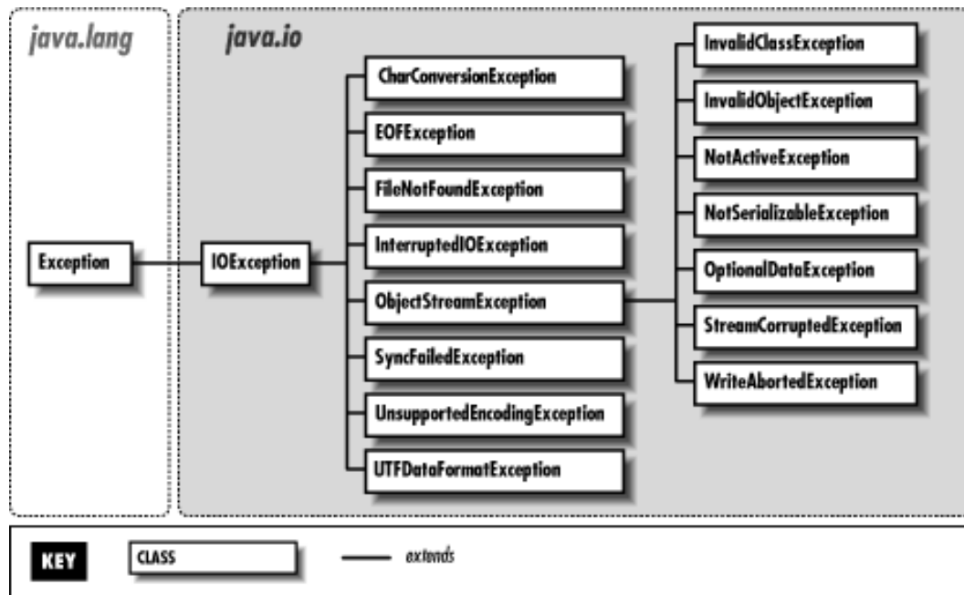
Figure 24.2: The exception classes of the java.io package
