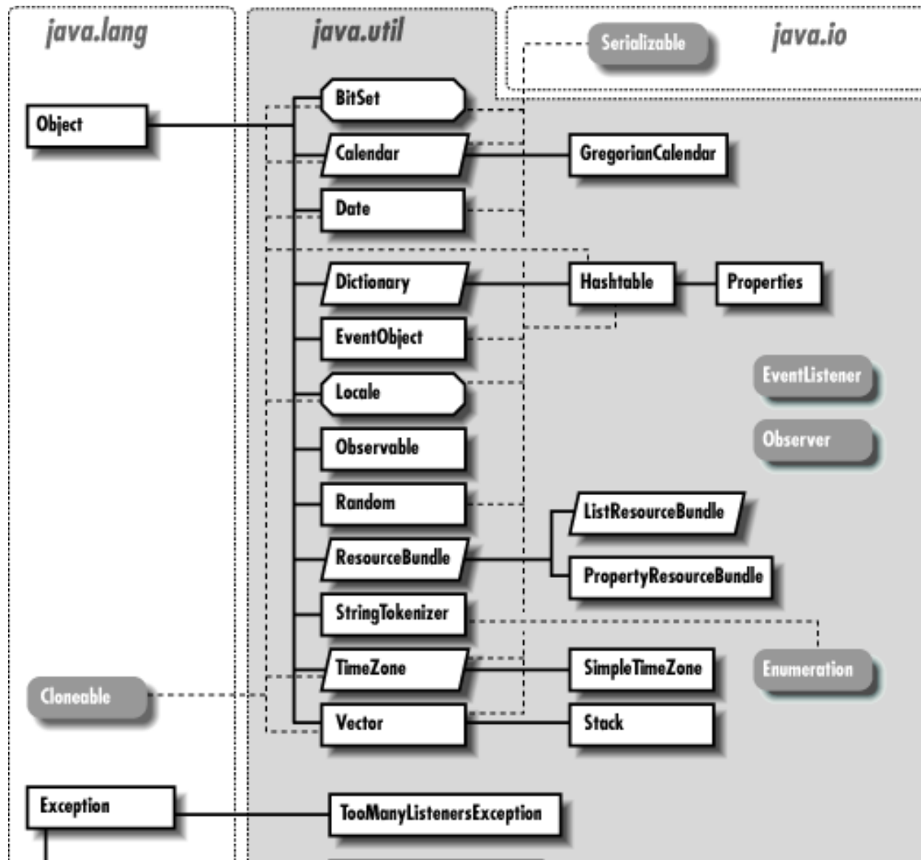
Figure 17.1: The java.util package
