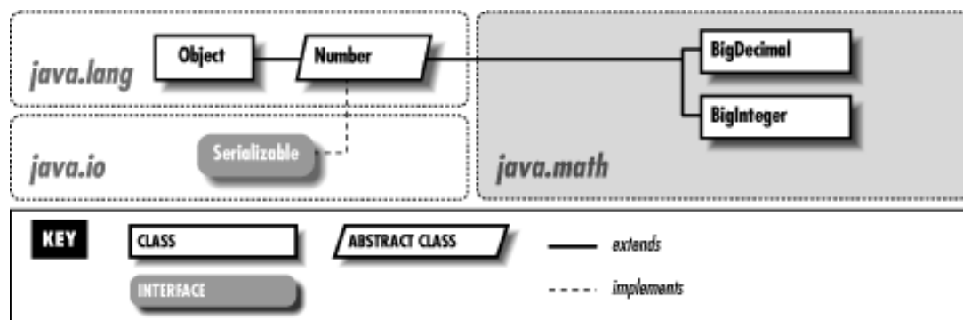
Figure 27.1: The java.math package
