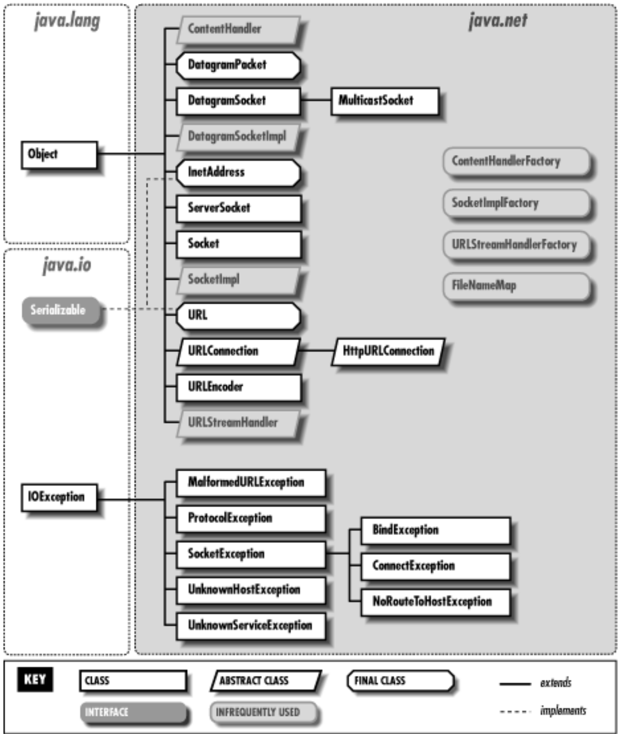
Figure 28.1: The java.net package
