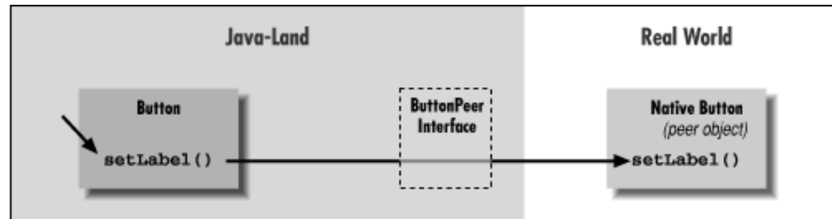
Figure 10.4: Invoking a method in the peer interface
