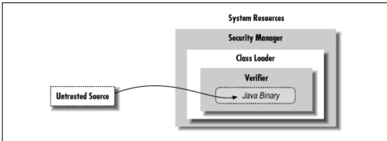
Figure 1.3: The Java security model
