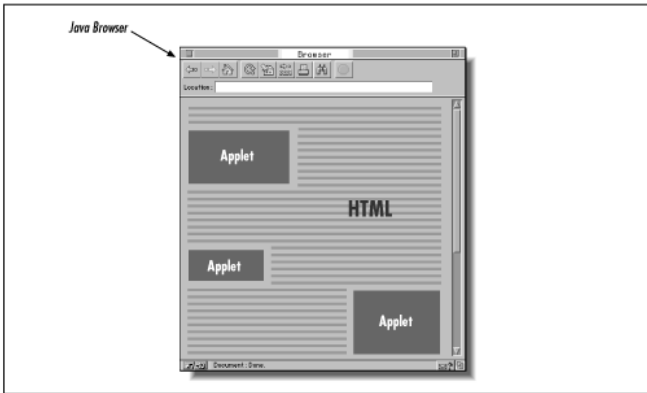
Figure 1.4: Applets in a Web document
