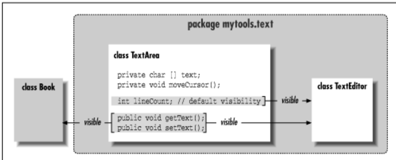
Figure 5.8: Private, default, protected, and public visibility
