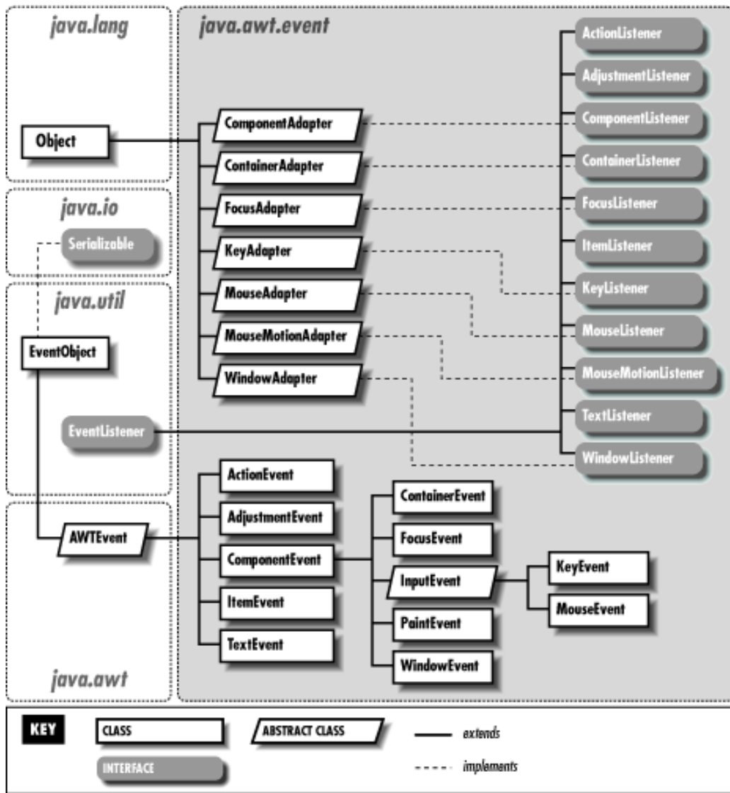
Figure 20.1: The java.awt.event package
