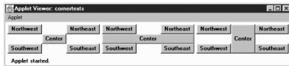
Figure 7.16: HorizBagLayout
