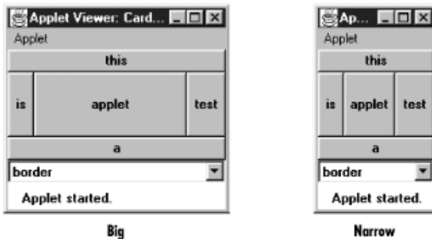
Figure 1.13: A BorderLayout
