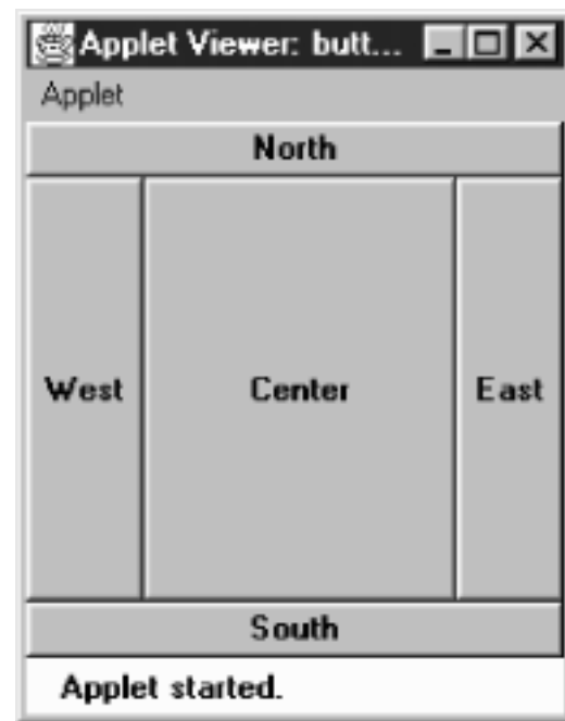
Figure 7.4: BorderLayout
