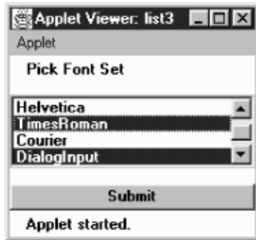
Figure 9.3: Multiselect List
