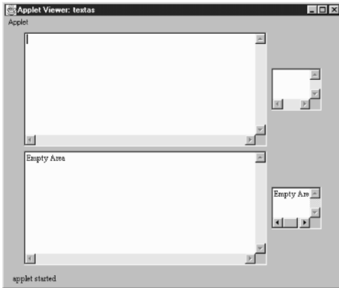
Figure 8.3: TextArea constructor
