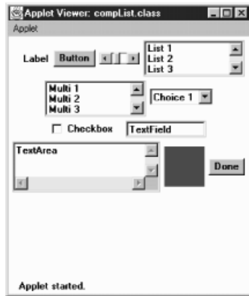
Figure C.1: Test program
