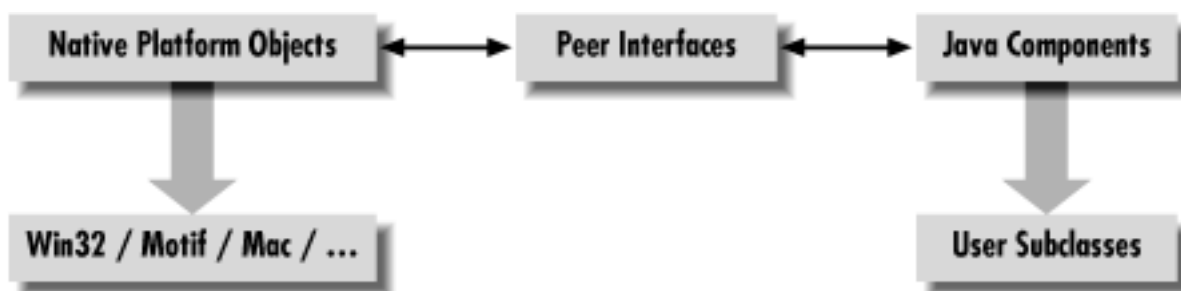
Figure 1.10: Peer architecture
