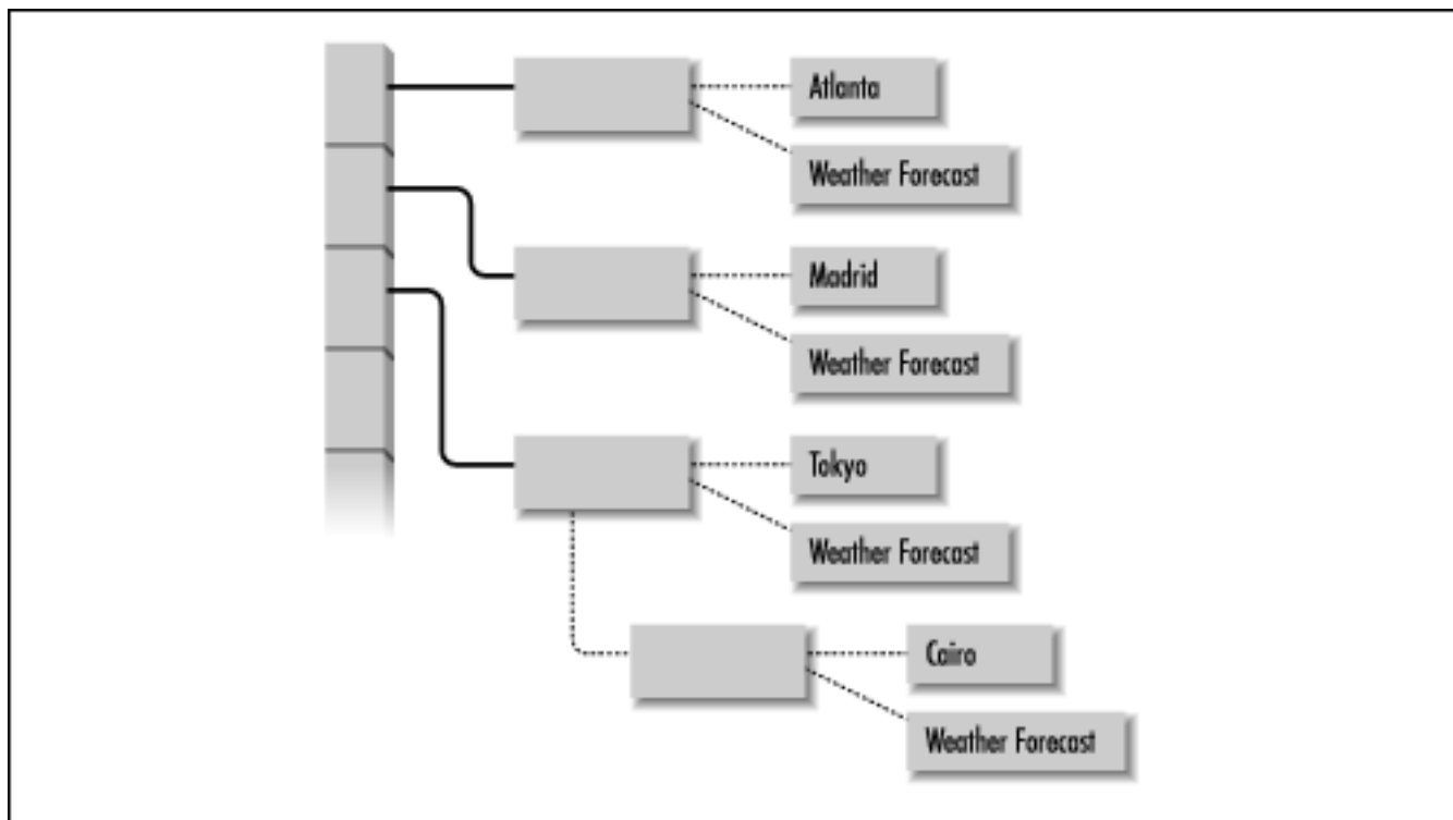
Figure 5.2: An array of key/value pairs that uses chained hashing
