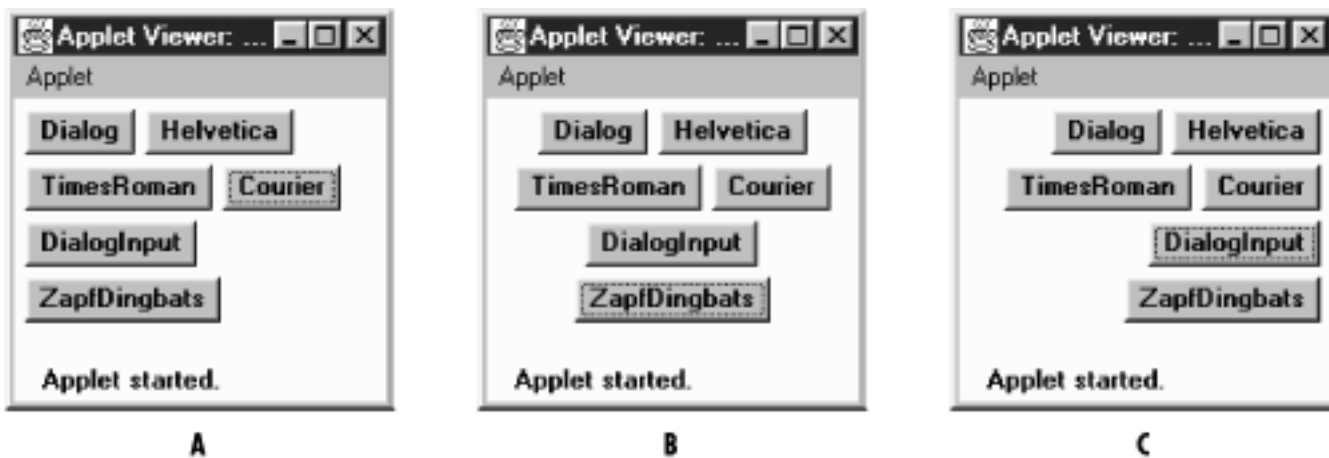
Figure 7.2: FlowLayout with three different alignments
