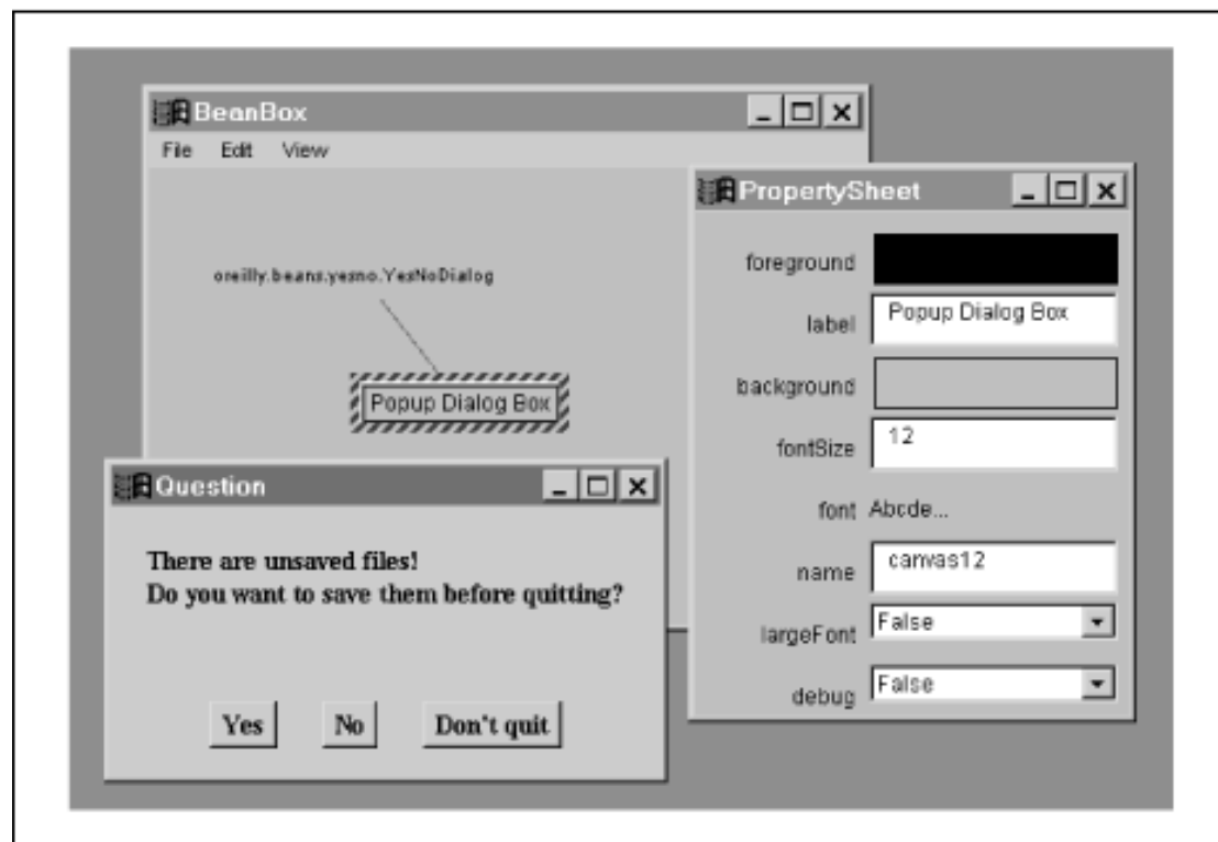
Figure 10.1: The YesNoDialog bean in the beanbox
