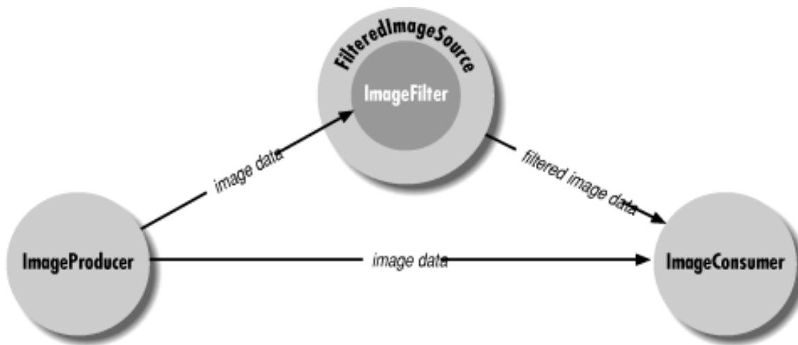
Figure 12.1: Image producers, filters, and consumers
