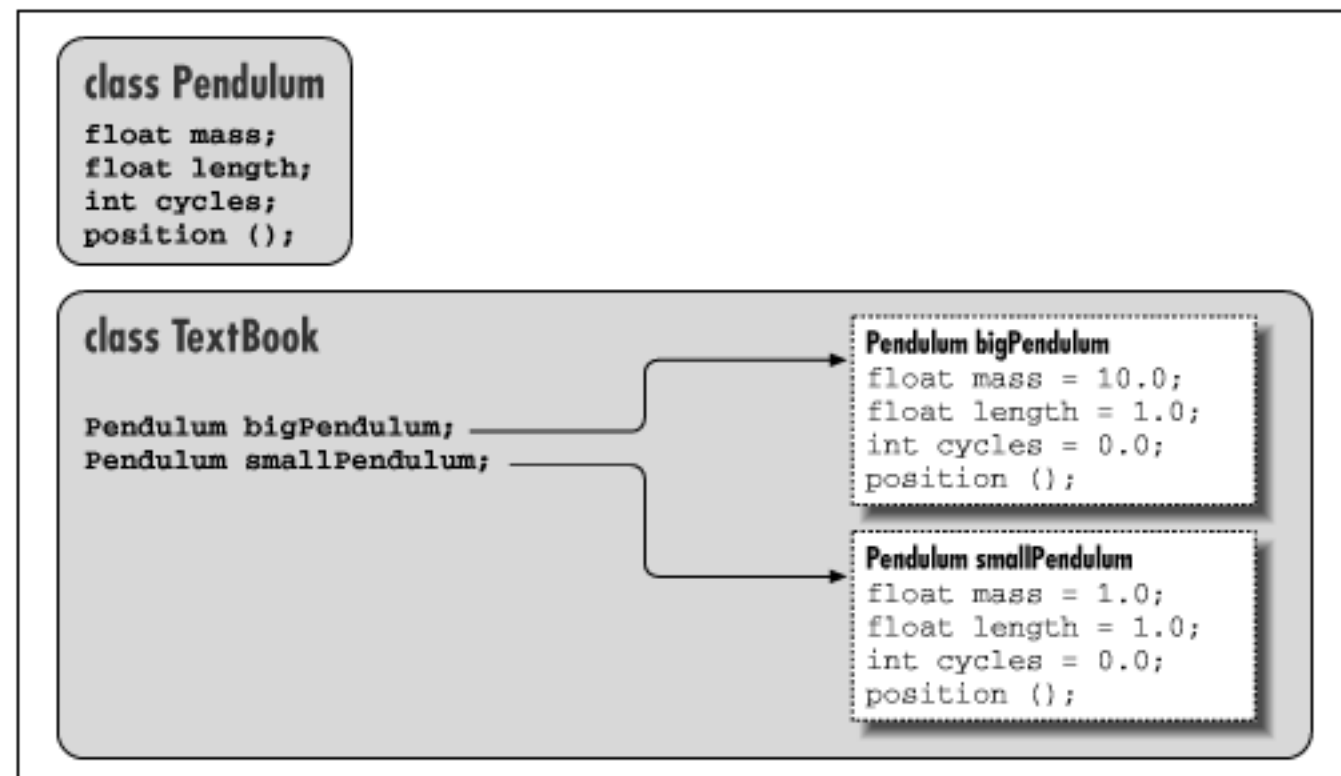
Figure 5.1: Instances of the Pendulum class
