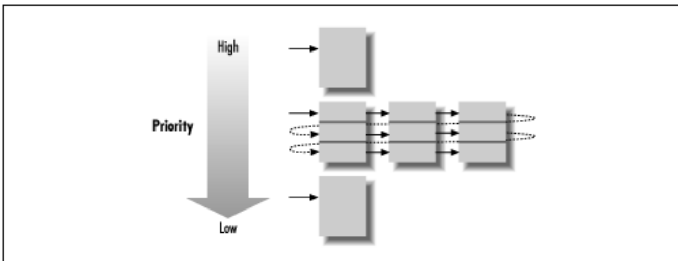
Figure 6.5: Priority preemptive, time-sliced scheduling
