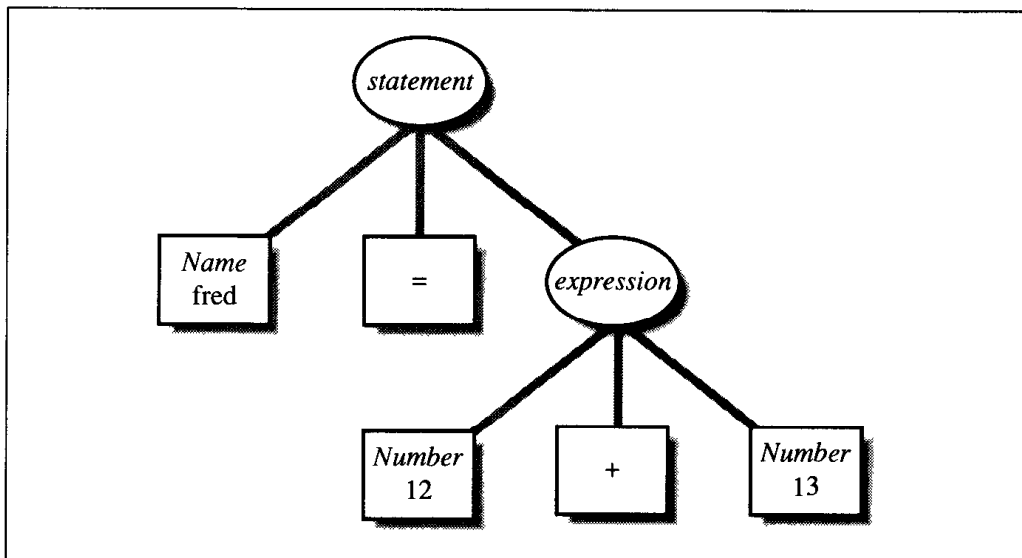
Figure 3-1: A parse tree
