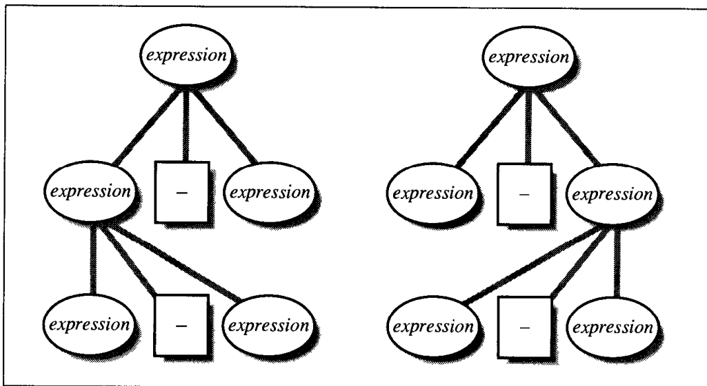
Figure 8-1: Ambiguous input expr - expr - expr
