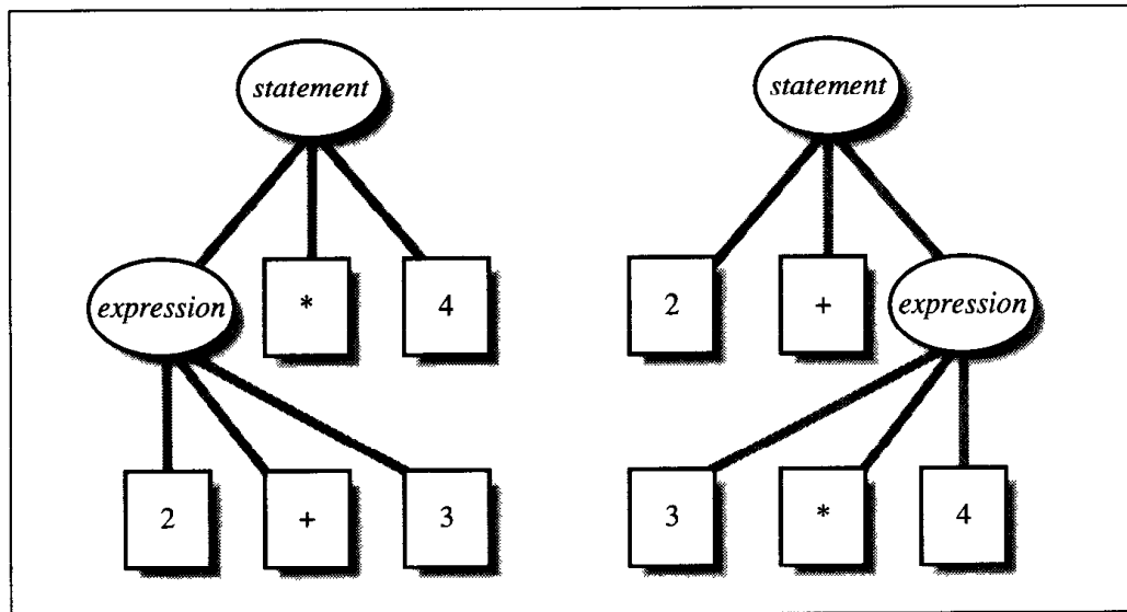
Figure 3-3: Ambiguous input 2+3*4
