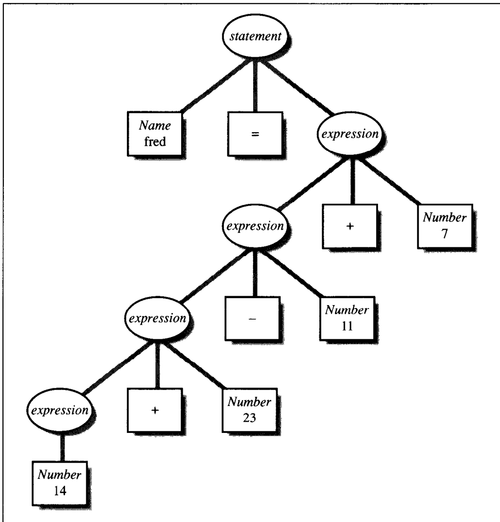
Figure 3-2: A parse using recursive rules
