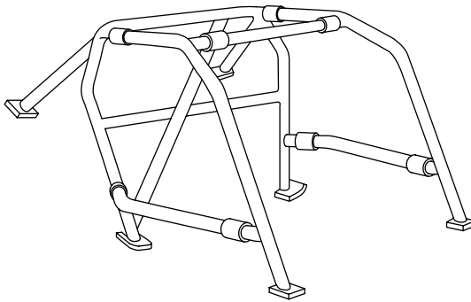
Figure 4-5: A six-point bolt-in roll cage.
