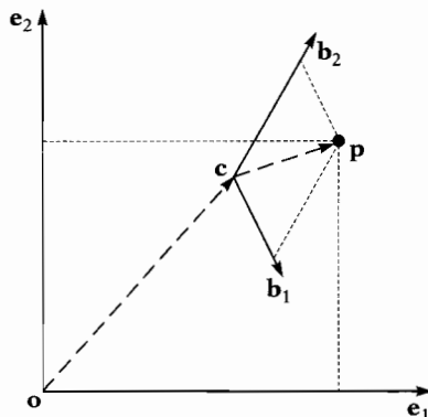
Figure 2.1 An affine transformation in \mathbb{R}^2 . Point \mathbf{p} is given in coordinates relative to the coordinate system (\mathbf{c}, \{\mathbf{b}_1, \mathbf{b}_2\}) . The coordinate vector of \mathbf{p} relative to the world coordinate system (\mathbf{o}, \{\mathbf{e}_1, \mathbf{e}_2\}) is \mathbf{B}\mathbf{p} + \mathbf{c} , where \mathbf{B} = [\mathbf{b}_1, \mathbf{b}_2] .
