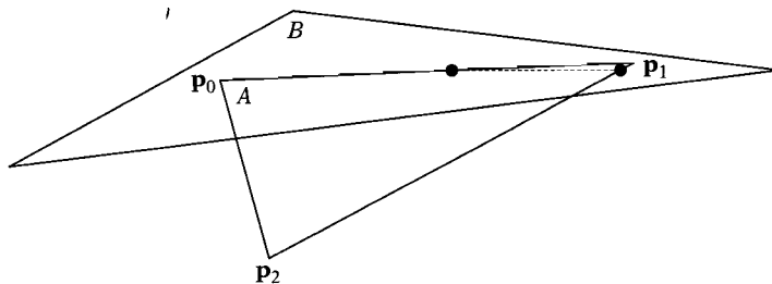
Figure 3.9 The edge \overline{p_0p_1} is almost parallel to triangle B 's plane, and thus is regarded as nonintersecting by the finite-precision ray-triangle test. The only intersecting edge we find is \overline{p_1p_2} .
