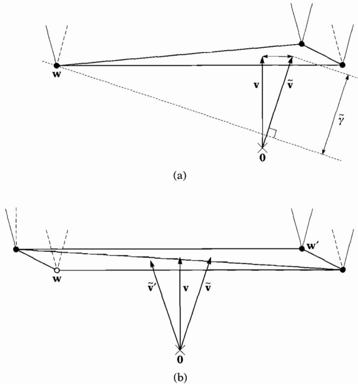
Figure 4.10 Two types of oscillations in GJK when the termination conditions are not met due to an ill-conditioned error bound. (a) A slight error in \tilde{\mathbf{v}} causes a huge error in the error bound \tilde{\gamma} = \|\mathbf{v}\|^2 - \mathbf{v} \cdot \mathbf{w} and prevents GJK from terminating. The same support point \mathbf{w} is found in each following iteration. (b) If \mathbf{v} lies close to the diagonal of a quadrilateral, then failure to meet the termination condition may cause GJK to alternate between two support points.
