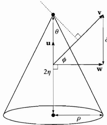
Figure 4.8 Computing a support point for a cone. For the top angle \theta , we have \sin(\theta) = \rho/\sqrt{\rho^2 + (2\eta)^2} . The apex is a support point only if \phi , the angle between \mathbf{v} and \mathbf{w} , is at least \theta . We have \sin(\phi) = \delta/\|\mathbf{v}\| , where \delta = \mathbf{u} \cdot \mathbf{v} .
