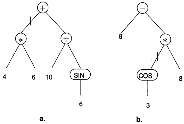
Figure 15.5 Two programs, selected on fitness for crossover. Point l from a and b are randomly selected for crossover.
