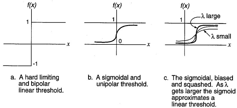
Figure 14.7 Thresholding functions.
