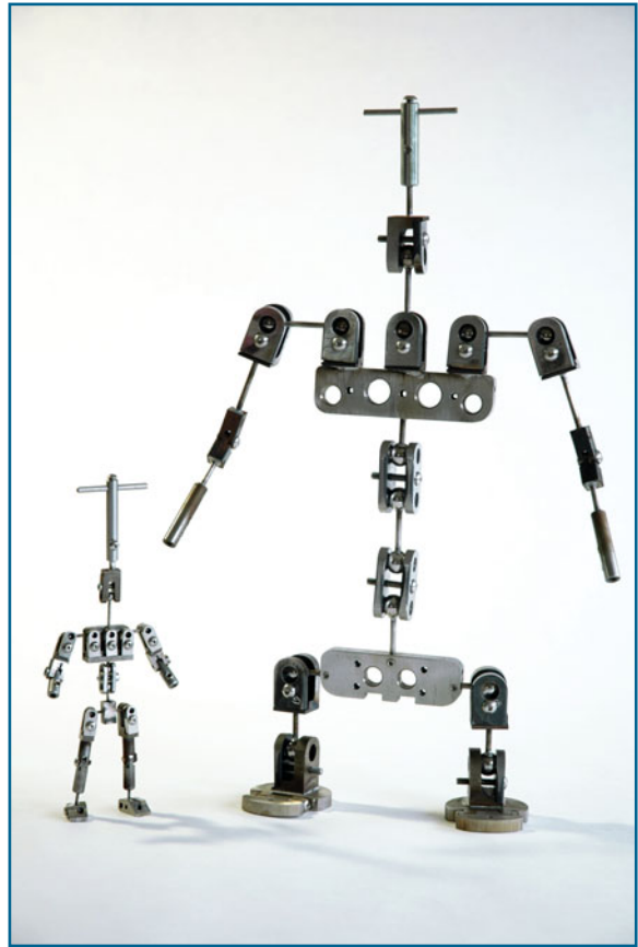
Figure 3.35 Ball-and-socket armatures for Ava and Charlie.
