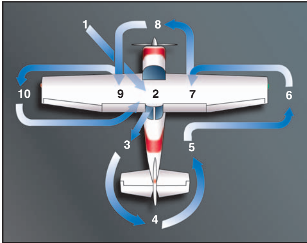
Figure 2-2. Preflight inspection.
