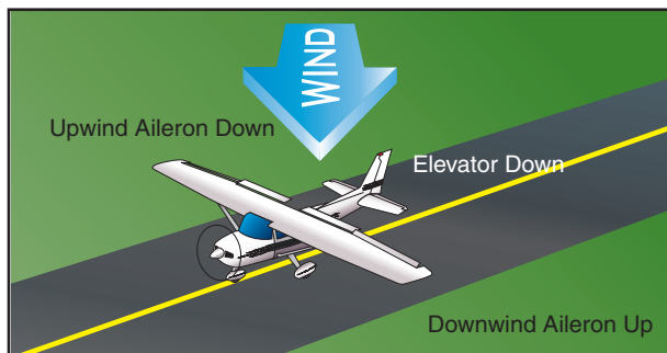
Figure 2-13. Quartering tailwind.
