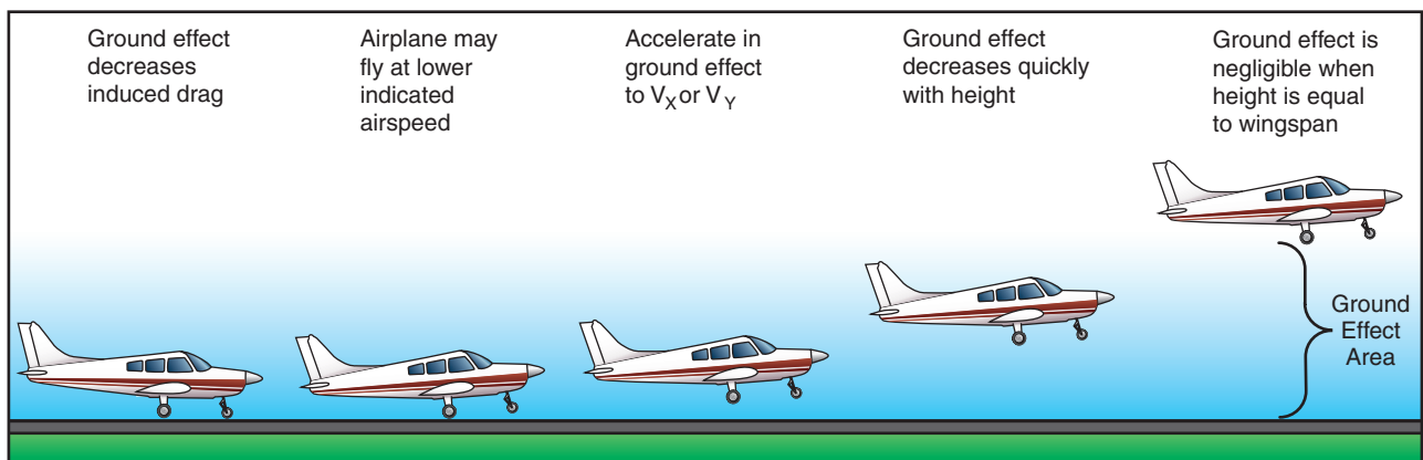
Figure 5-6. Takeoff in ground effect area.
