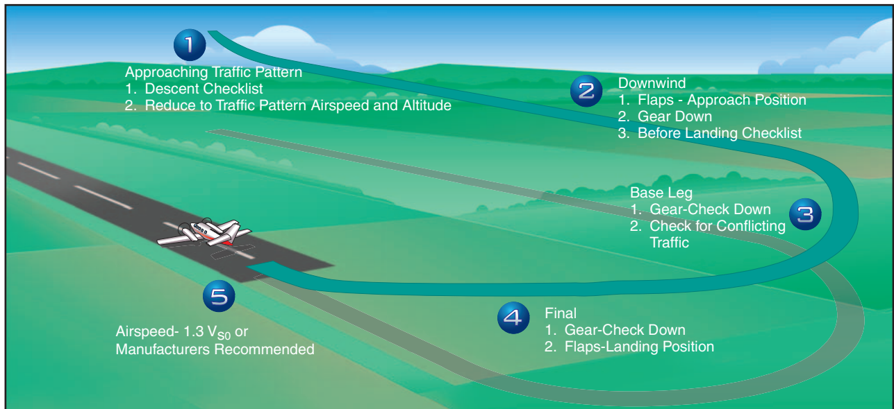
Figure 12-8. Normal two-engine approach and landing.
