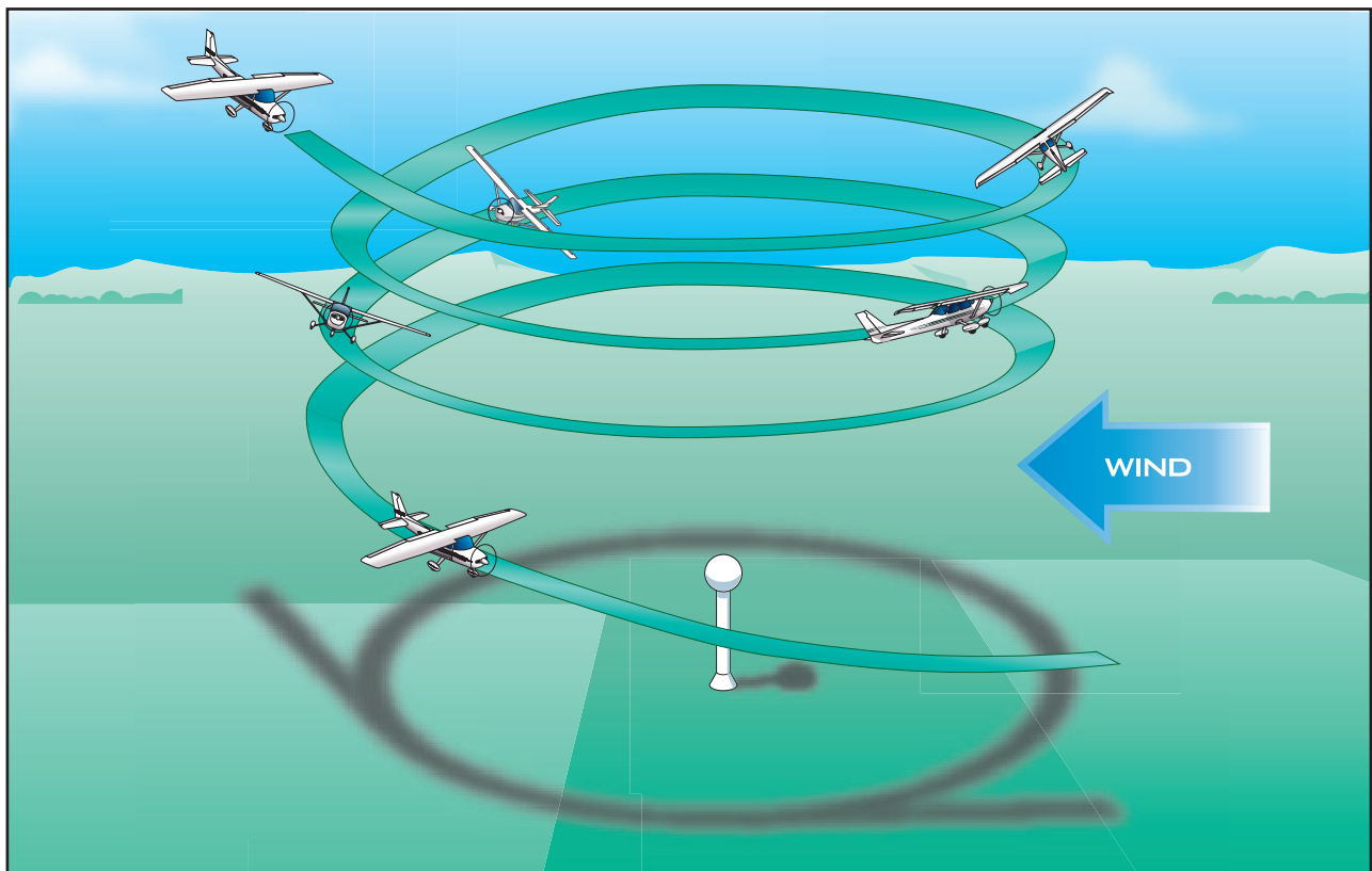
Figure 9-2. Steep spiral.
