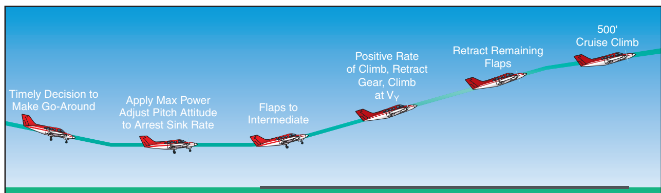
Figure 12-10. Go-around procedure.
