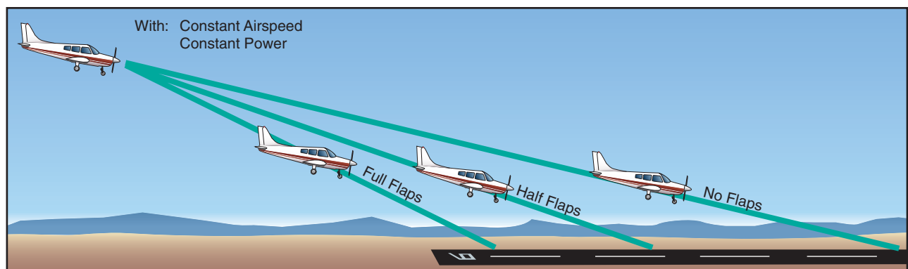
Figure 8-3. Effect of flaps on the landing point.
