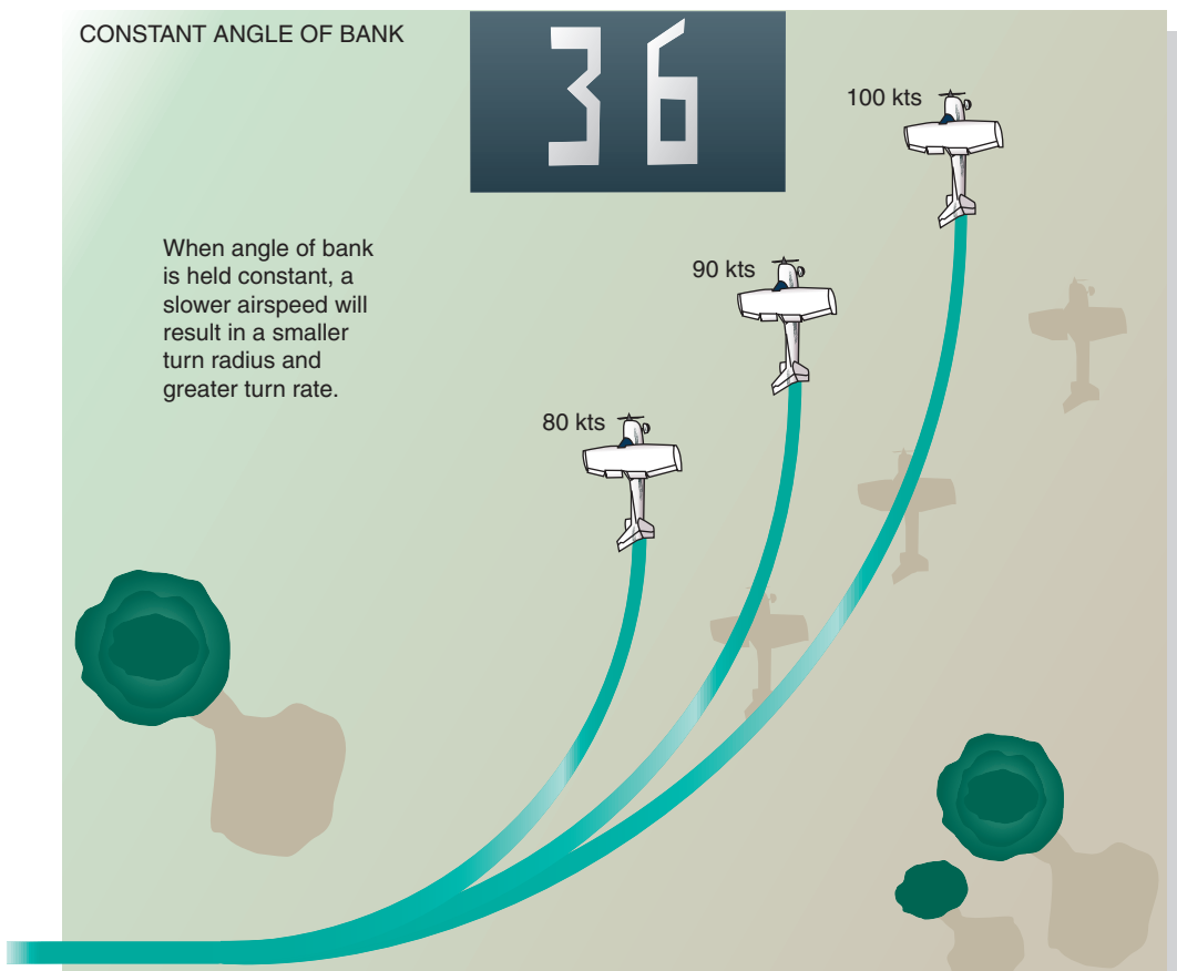
Figure 3-9. Angle of bank and airspeed regulate rate and radius of turn.
