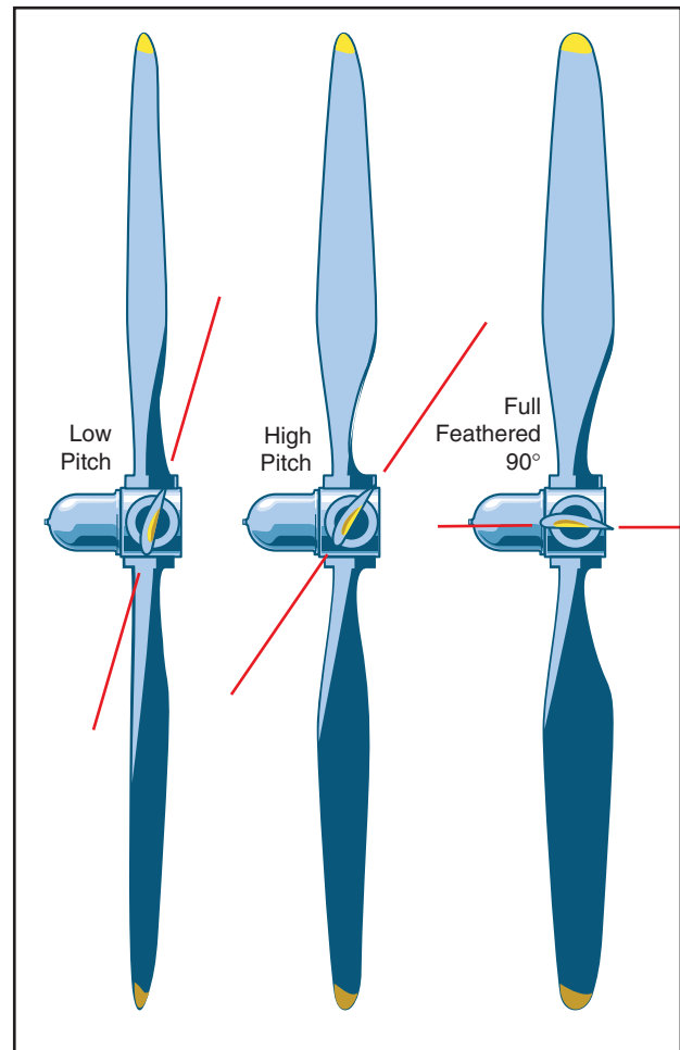
Figure 12-2. Feathered propeller.
