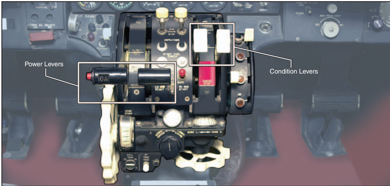
Figure 14-3. Powerplant controls—fixed shaft turboprop engine.
