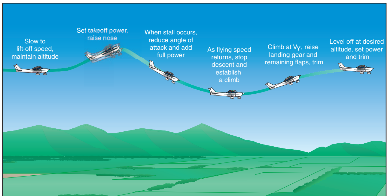
Figure 4-6. Power-on stall.
