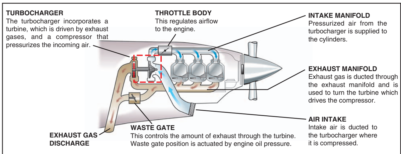
Figure 11-5. Turbocharging system.
