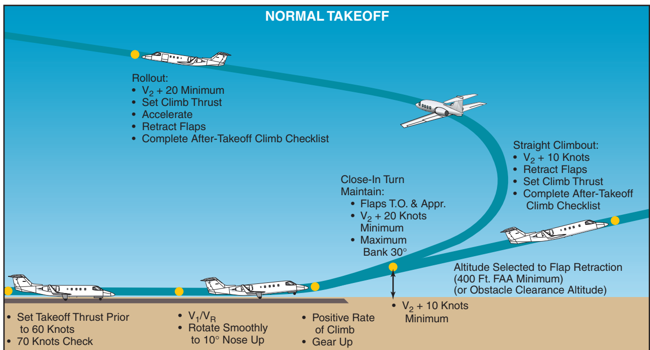
Figure 15-21. Takeoff and departure profile.
