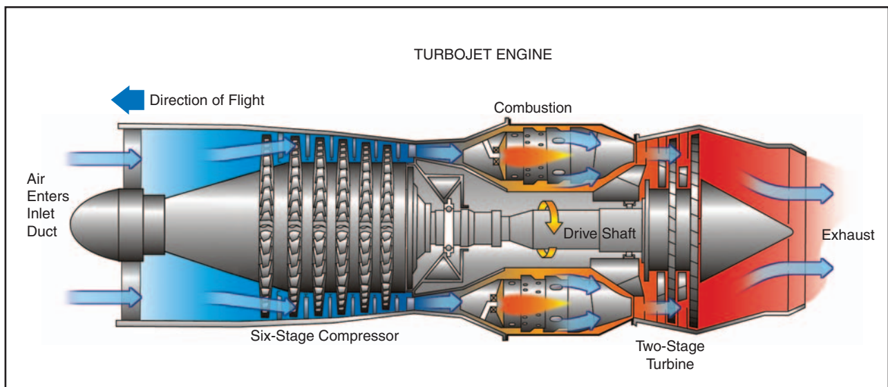
Figure 15-1. Basic turbojet engine.
