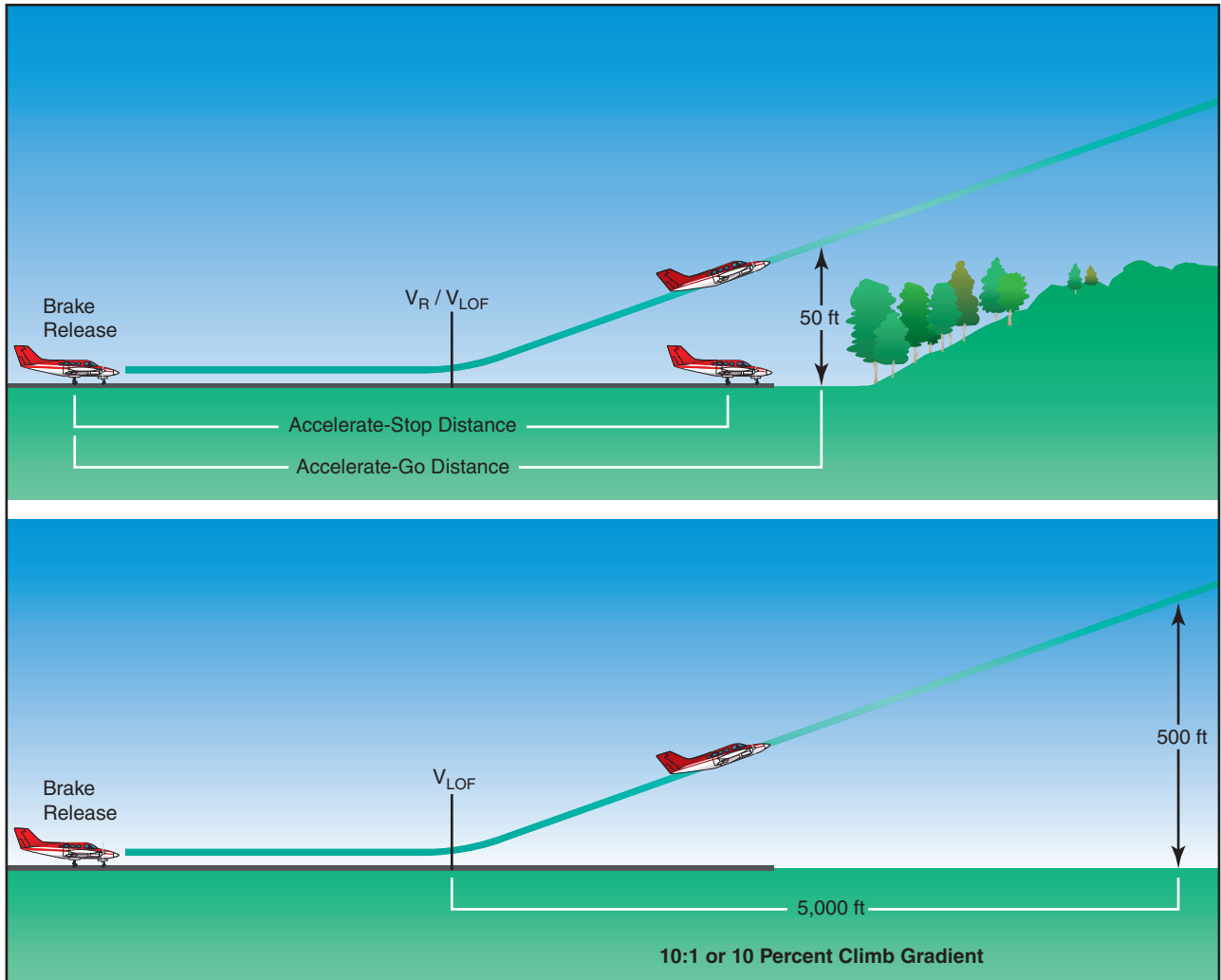
Figure 12-5. Accelerate-stop distance, accelerate-go distance, and climb gradient.
