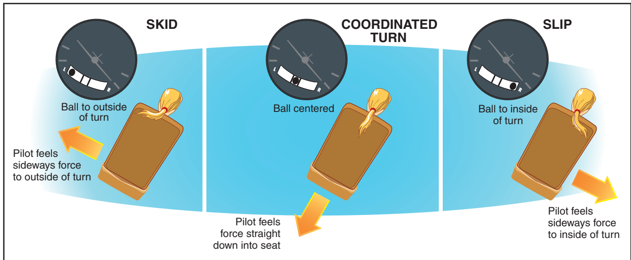
Figure 3-8. Indications of a slip and skid.
