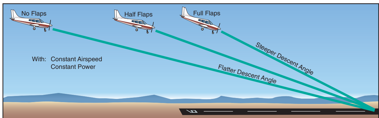
Figure 8-4. Effect of flaps on the approach angle.
