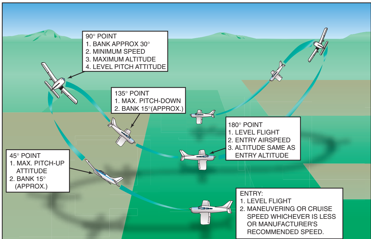
Figure 9-5. Lazy eight.
