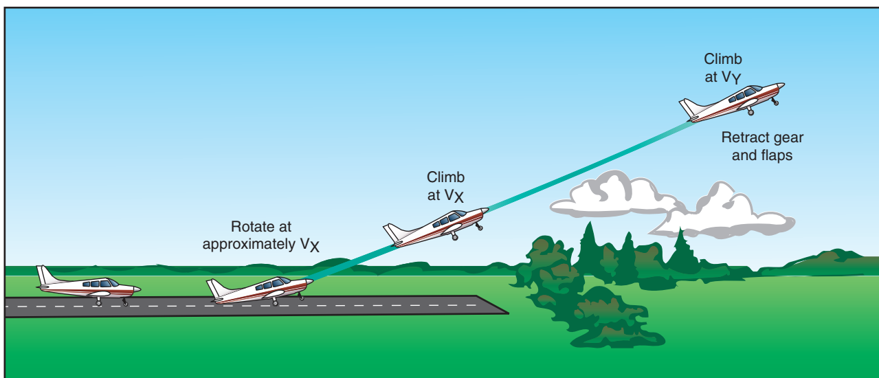
Figure 5-7. Short-field takeoff.
