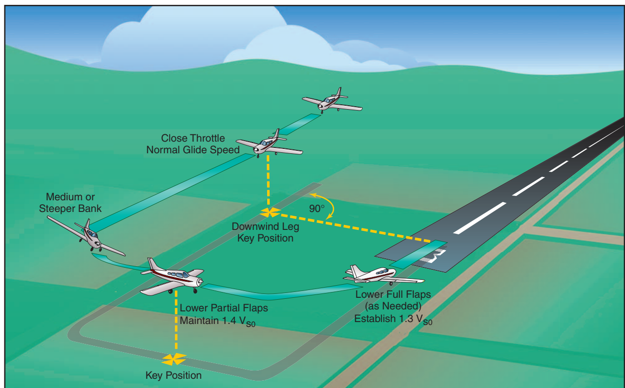
Figure 8-27. 180° power-off approach.
