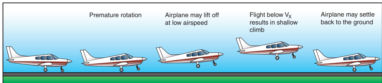
Figure 5-8. Effect of premature lift-off.
