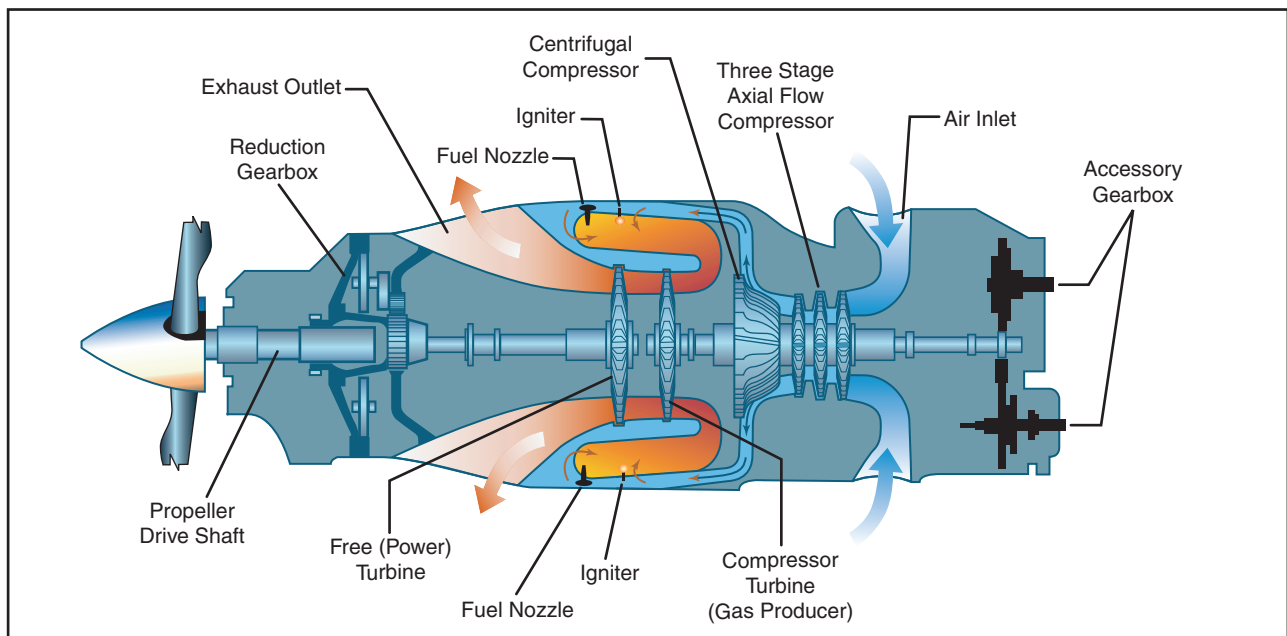
Figure 14-5. Split shaft/free turbine engine.
