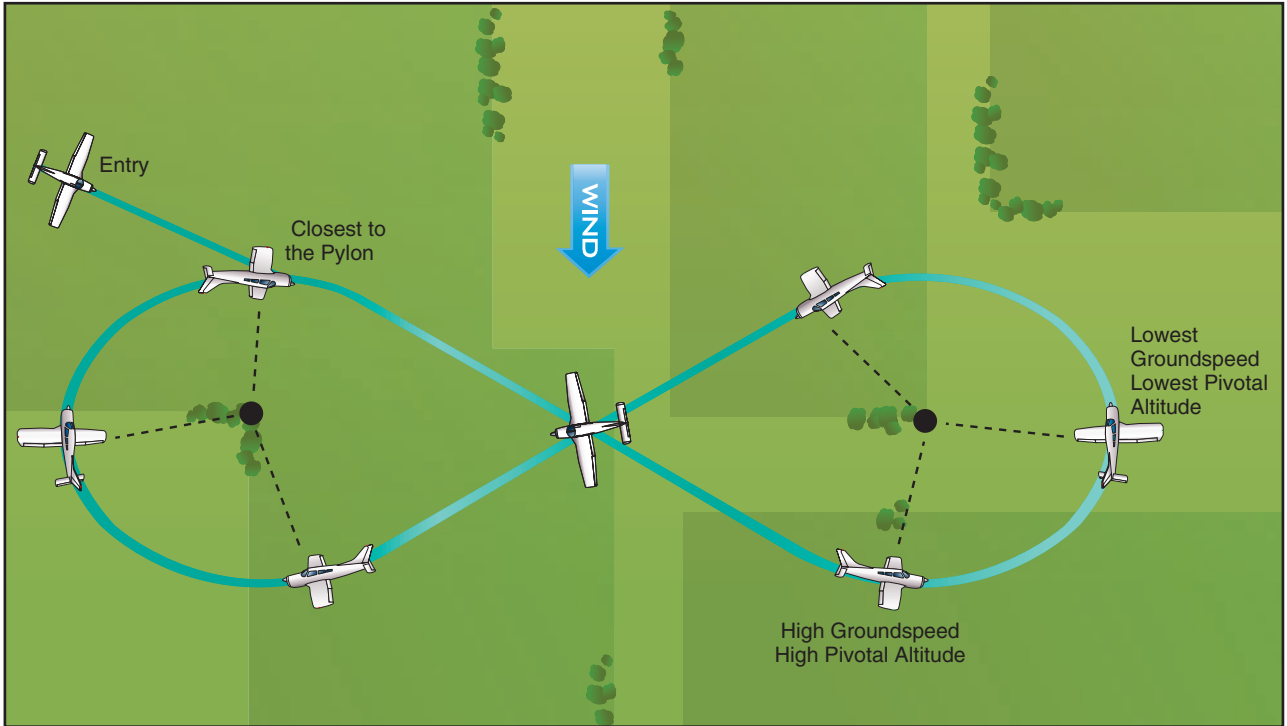
Figure 6-10. Eights-on-pylons.
