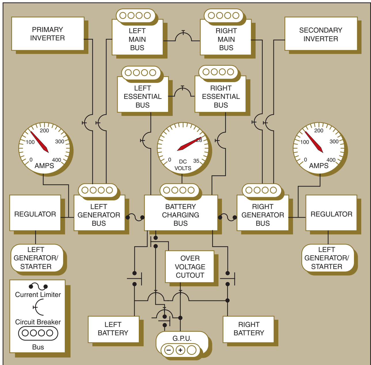
Figure 14-10. Simplified schematic of turboprop airplane electrical system.
