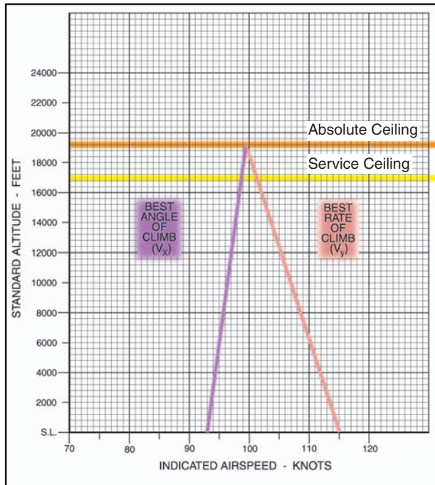
Figure 3-15. Absolute ceiling.
