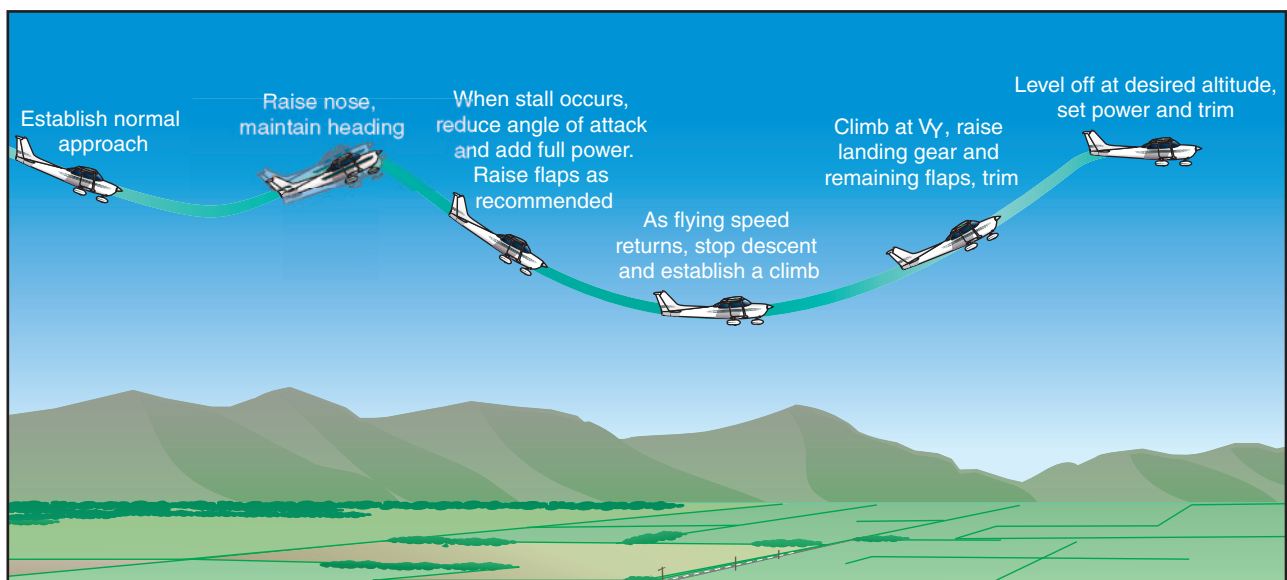
Figure 4-5. Power-off stall and recovery.
