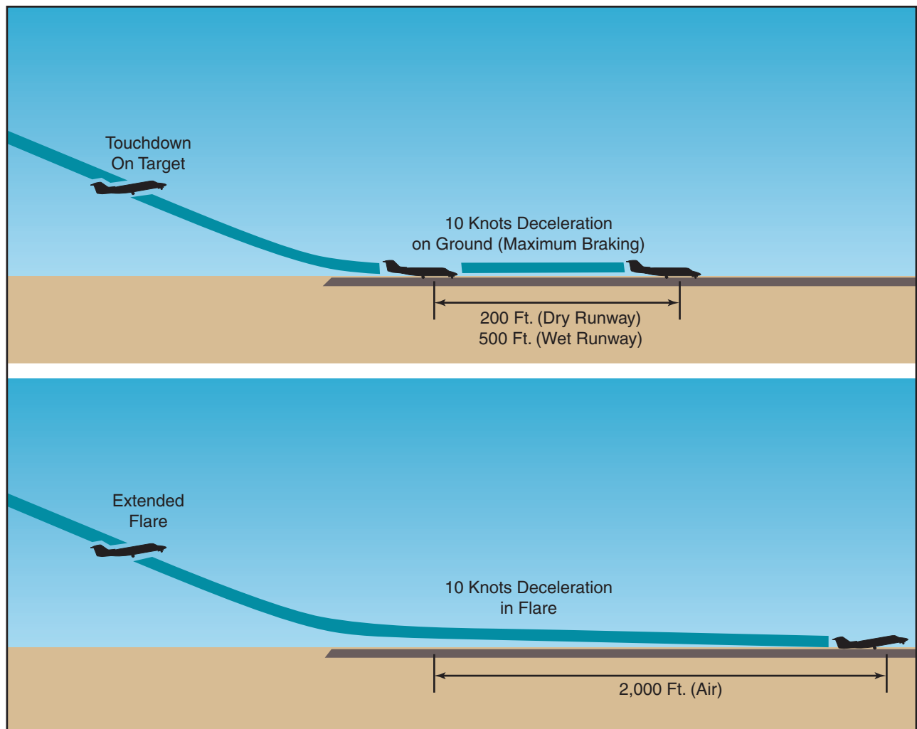
Figure 15-25. Extended flare.
