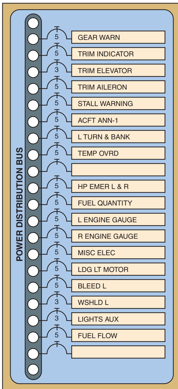
Figure 14-9. Typical individual power distribution bus.
