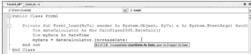
Figure 13-4: Overload- ing and IntelliSense.
