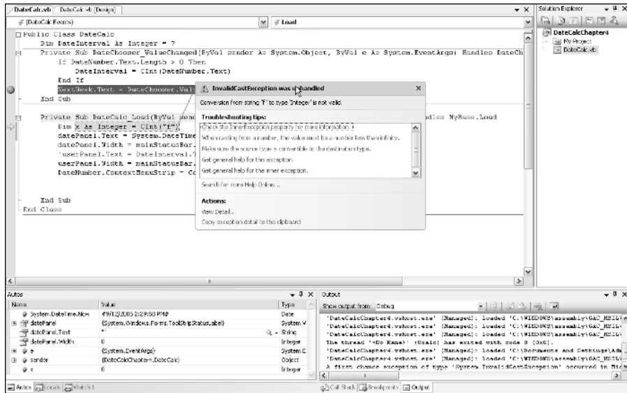
Figure 9-2: You can't enter text in a text box cast as an integer!
