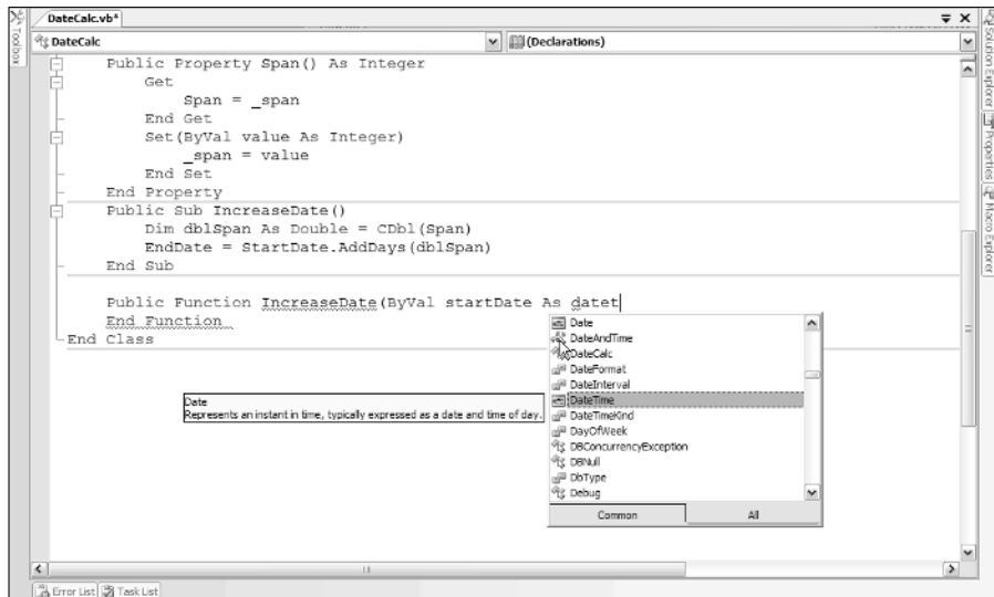
Figure 6-5: Declaring a function.
