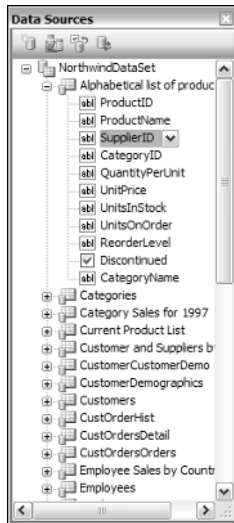
Figure 2-9: The Data Sources window.
