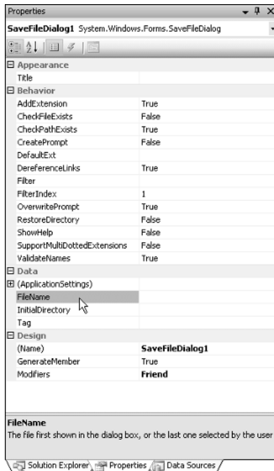
Figure 16-3: Options for the SaveFile Dialog control .
