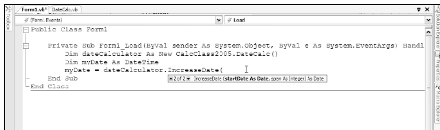
Figure 6-6: Overloading in the IDE — IntelliSense shows two overloads.
