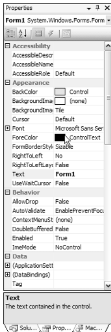
Figure 2-4: The Properties window.
