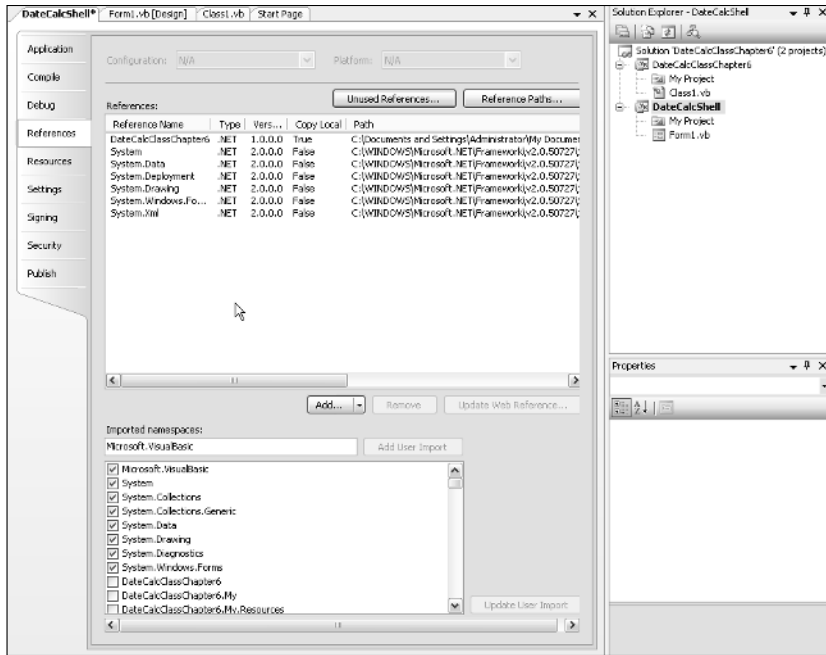
Figure 6-4: The References tab of the My Project file.
