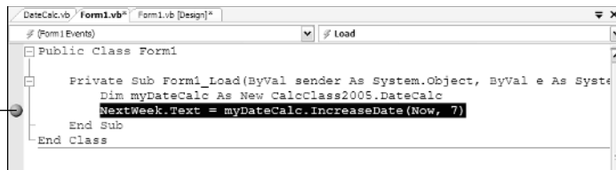
Figure 8-1: Making a breakpoint.
