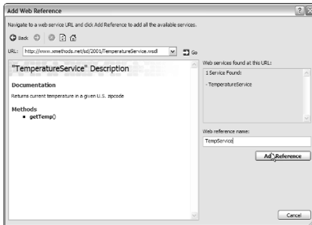
Figure 20-1: Adding a reference to the Temp- Service.
