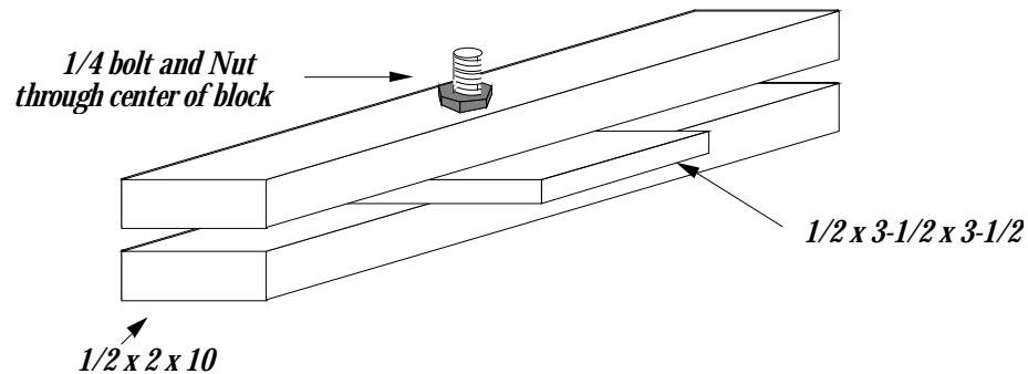
Figure 8 Spacer Block - make 2
