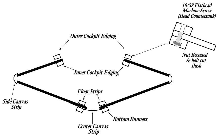
Cross Section-Midship
