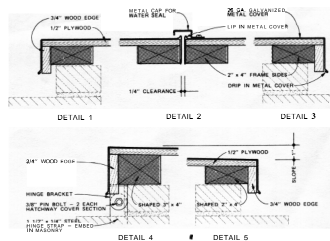
HATCHWAY COVER DETAILS
