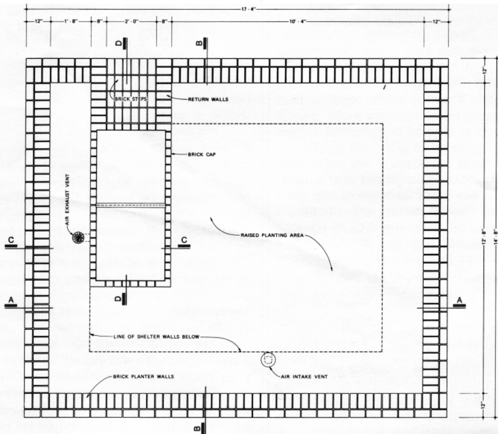
PLAN OF PLANTER AND HATCHWAY AT YARD LEVEL
