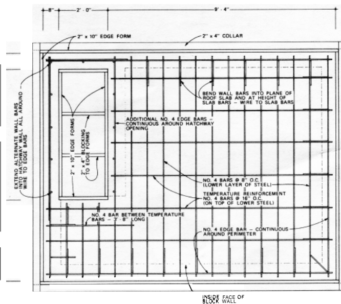
ROOF SLAB REINFORCEMENT PLAN
