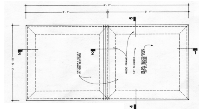
PLAN OF HATCHWAY COVER
