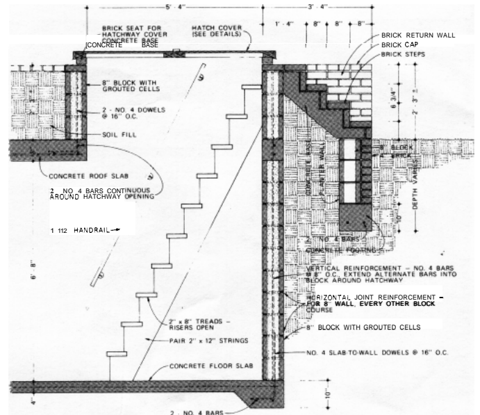
SECTION D - D AT HATCHWAY
