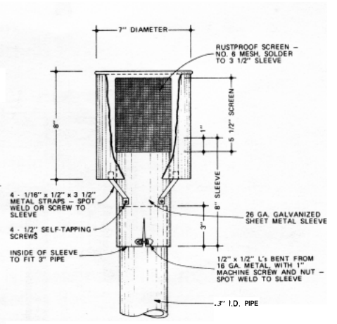
AIR INTAKE HOOD DETAIL
