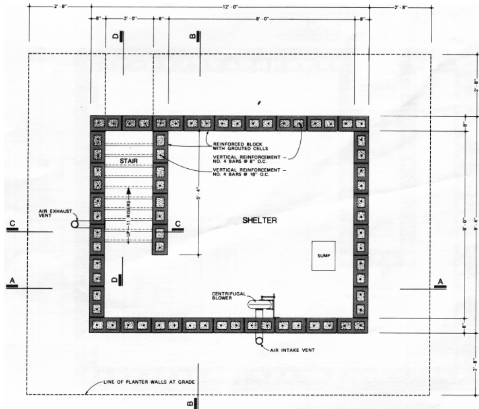
FLOOR PLAN OF THE SHELTER
