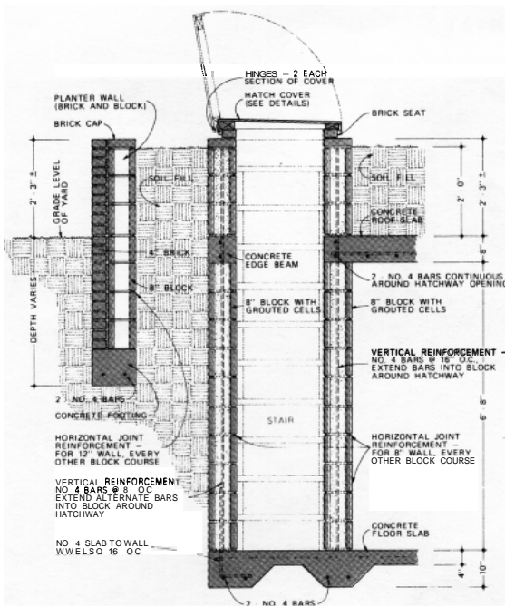
SECTION C - C AT HATCHWAY
