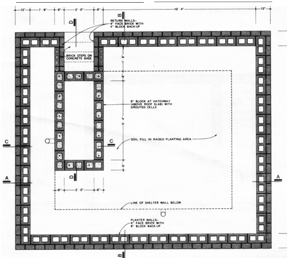
PLAN SHOWING PLANTER WALLS AND HATCHWAY WALLS
