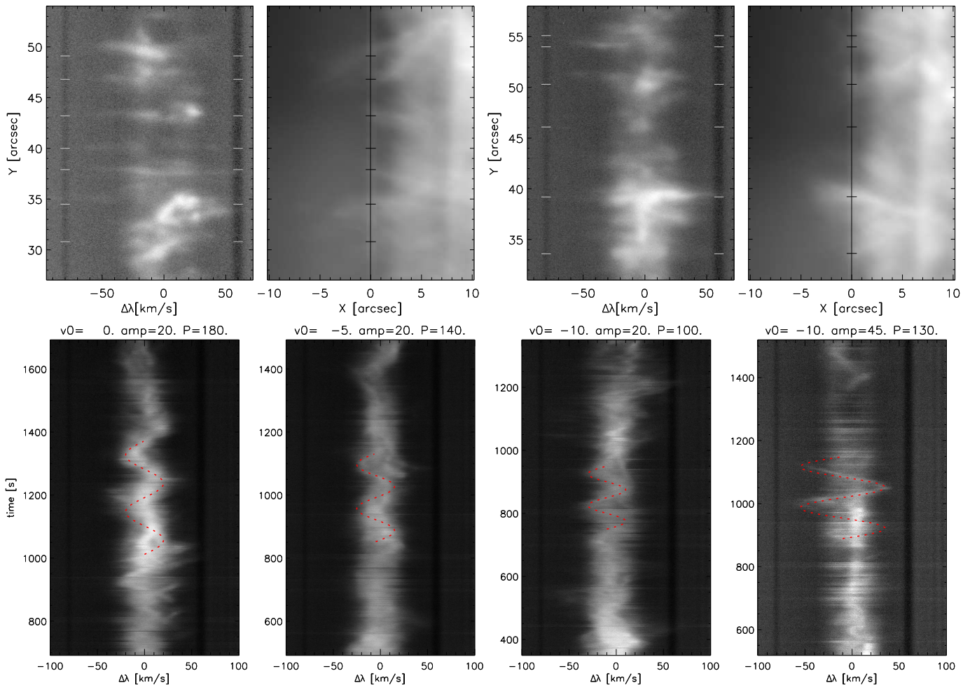
Figure 1. Examples of large torsional motion in off-limb spicules in Ca II H. Top row shows the spatial variation of the Ca II H profile, with the righthand panel of each pair a slit-jaw image with the off-limb intensities enhanced with a radial filter. These show spicules protruding upwards from the limb which is to the right. The lefthand panels are corresponding Ca II H spectrograms. The black line in the slit-jaw images shows the slit location. The spectrograms are dominated by linear features that are often tilted from the horizontal dispersion direction, a clear signature of torsional motions, typically over 20\text{--}40\text{ km s}^{-1} . Selected spicules are marked by black ticks in the slit-jaw images and white ticks in the spectrograms. Bottom row shows examples of large swaying motion in off-limb spicules in Ca II H. Each panel shows the temporal evolution of the Ca II H profile. Despite significant superposition of multiple oscillatory signals there are often episodes of quasi-sinusoidal oscillation. For guidance we have overlotted sinus curves with the amplitude (“amp” in \text{km s}^{-1} ) and period ( P in s) specified in each legend.
