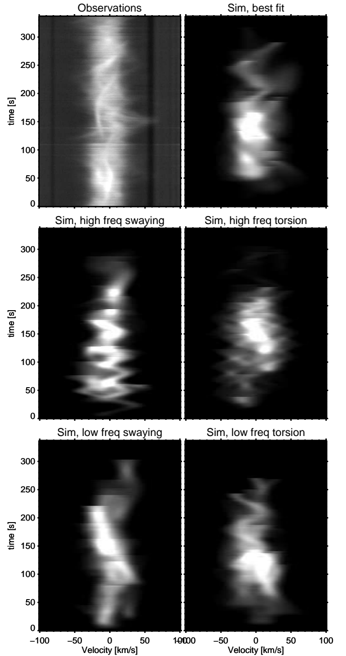
Figure 3. Comparison between observations and Monte Carlo simulations in \lambda - t displays. The best-fit solution has field-aligned velocities of 60 \text{ km s}^{-1} , torsional velocities of 30 \text{ km s}^{-1} and swaying motions of 15 \text{ km s}^{-1} with periods of 100-300 s. Significant discrepancies occur for wave periods that are much higher or lower than these values.
