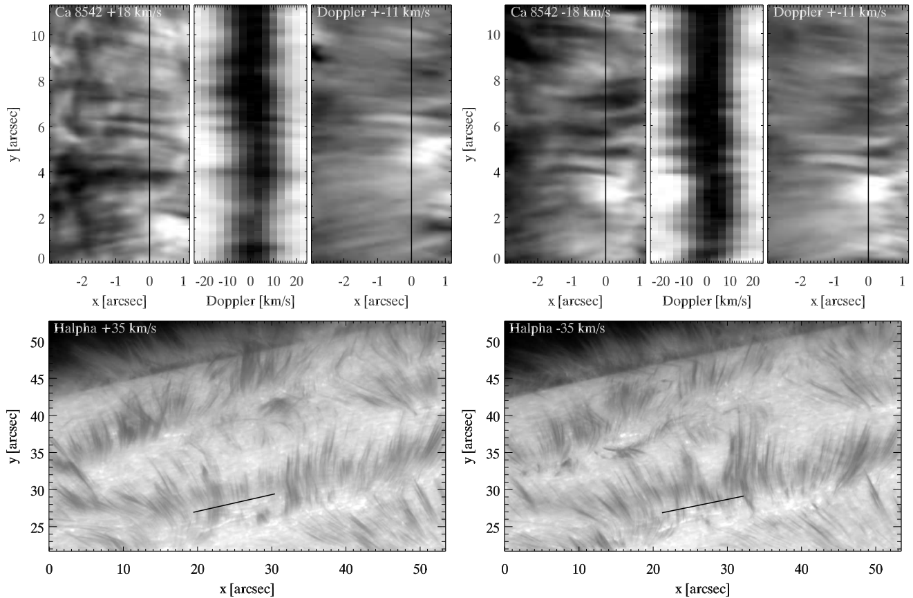
Figure 5. Two examples of CRISP Ca II 854.2 nm spectral behavior close to the limb which is to the left (in top row). The slit-like sampling crossed a bush of near-limb spicules as shown by the black line in the H \alpha context images in the lower row. In the top row, each Ca II \lambda - y diagram is accompanied by two Ca II slit-jaw images that have the location of the slit marked by a black line, at left a wing image, at right a Doppler image. The Ca II spectrograms and images were taken 17 s apart, the righthand trio first. The H \alpha images were taken within a few seconds of each other 34 s later.
