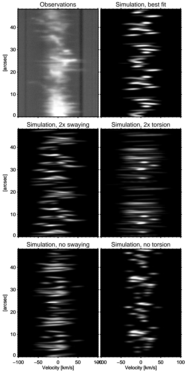
Figure 2. Comparison between observations and Monte Carlo simulations in \lambda - y displays. The best-fit solution has field-aligned velocities of 60 \text{ km s}^{-1} , torsional velocities of 30 \text{ km s}^{-1} and swaying motions of 15 \text{ km s}^{-1} with periods of 100-300 s. Significant discrepancies occur for larger swaying, more torsion, no swaying, and no torsion.
