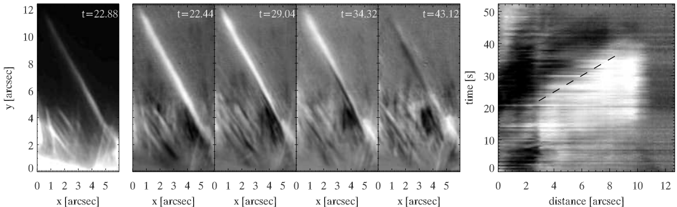
Figure 4. Example of sign change in spicule Doppler tilt in the ultra-high cadence ( 0.44 \text{ s} ) \pm 55 \text{ km s}^{-1} CRISP \text{H}\alpha data. Lefthand panel shows an \text{H}\alpha wing image at maximum spicule length. Center panels contain sequences of four Doppler images at different sampling times (in seconds, blueshift bright). The righthand panel show space-time diagrams measured along the spicule axis. Dashed guidelines illustrate a propagation speed of 285 \text{ km s}^{-1} .
