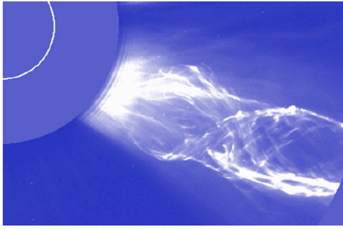
Fig. 4 Coronal mass ejection (CME) with a helical structure observed by LascoC2 on SOHO. Through spectro-polarimetric observations SolmeX will allow us to measure the magnetic field in these structures for the first time. (The thin white line outlines the solar limb).
