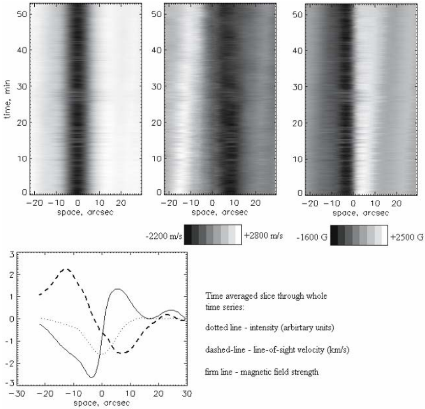
Figure 2. Example of the time series in AR NOAA 50 at August 3, 2002 (09:10 UT). Top left — continuum near 6569 \text{ \AA} , center — photospheric line-of-sight velocity, right — longitudinal magnetic field strength. Positive and negative velocities correspond to the direction to and from the observer, respectively.
