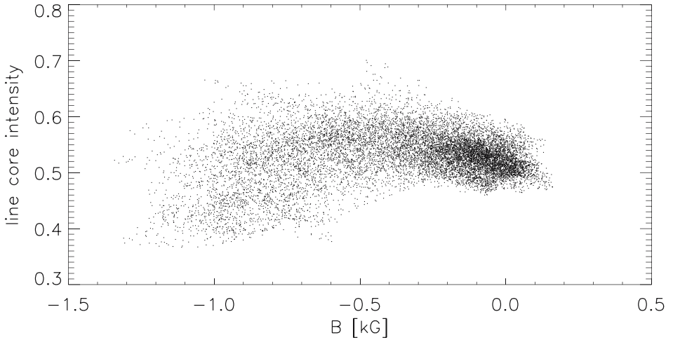
Figure 3. Relation of the line core intensity to the line-of-sight magnetic field strength. The distribution is the more scattered the stronger the field.
