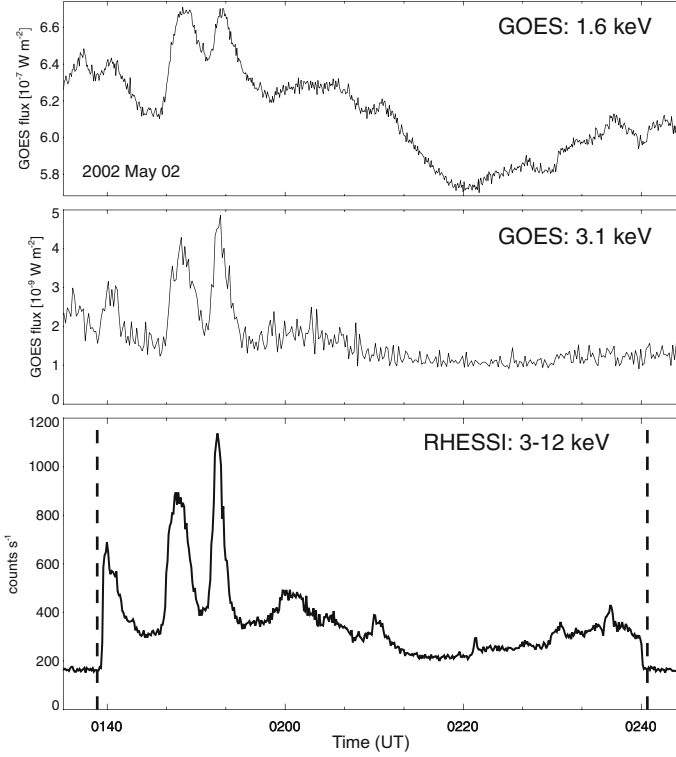
Figure 5. Results from Krucker et al. (2002) showing recurring microbursts of nonthermal HXRrs around 10 keV from active regions. (Dashed lines indicate the end/beginning of RHESSI night time.)
