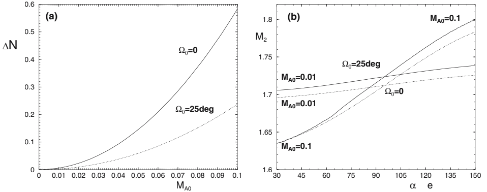
Figure 2. For \beta_0 = 0.01 , we present the dependence of: (a) the relative difference \Delta N_{\%} of the compression N and the Soward approximation value N_S ; (b) the outflow Mach number M_2 on the incidence angle \alpha for the inflow Mach Alfvén numbers M_{A0} = 0.01 and 0.1, combined with \Omega_0 = 25^\circ and 0^\circ (2-D case).
