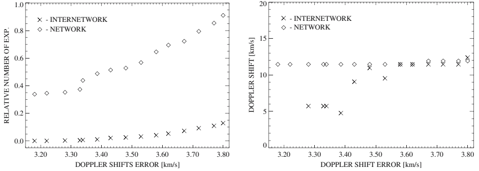
Figure 3. Left panel: Relative cumulative number of exposures from the internetnetwork and network as a function of the Doppler shift errors of O v line. Right panel: Doppler shifts of the O v spectral line in the internetnetwork and in the network as a function of the Doppler shifts errors.
