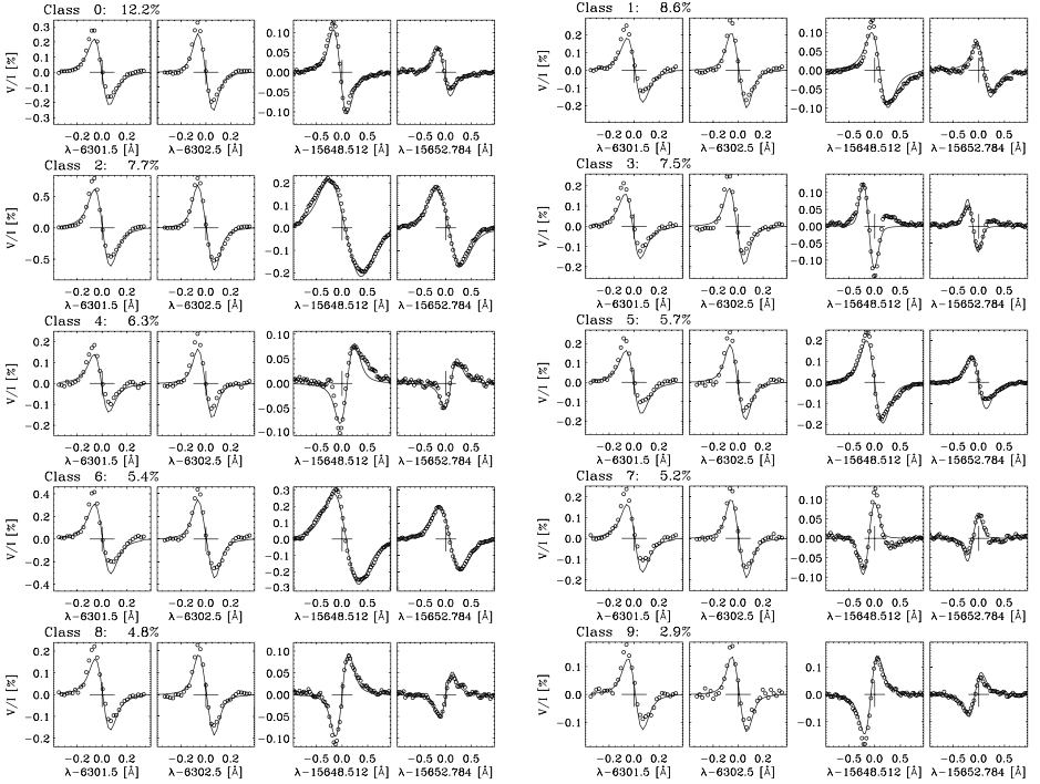
Figure 1. First 10 classes of Stokes V profiles from the PCA classification, with abundance in percentage. Circles represent observations (mean profile among those in each class), and solid lines are the ME fits.
