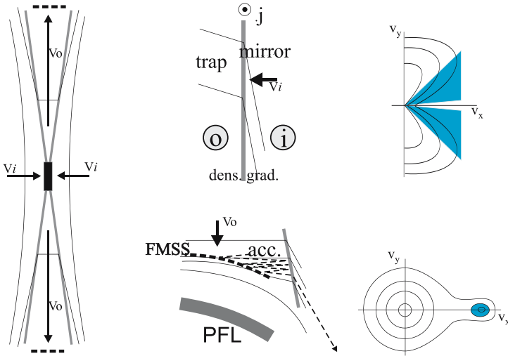
Figure 9. Left : Petschek’s model of fast reconnection in a current sheet. Middle : Properties of the model – magnetic mirrors at the SMSSs form magnetic bottle between the SMSSs (top); collapsing trap configuration between the SMSS and the FMSS providing particle acceleration above postflare loops (bottom). Right : Unstable velocity distribution functions f(v_x, v_y) – loss-cone (top); bump on tail (bottom). The velocity component in the direction of the magnetic field (“parallel velocity”) is denoted as v_x , and v_y represents the perpendicular one. The unstable regions ( \partial f/\partial v_{in} > 0 ) are shaded.
