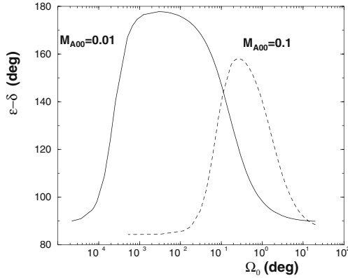
Figure 3. Illustrative results of dramatic changes in transition from 2\frac{1}{2} -D to 2-D. The difference of the angles ( \epsilon - \delta ) in region 1 in dependence on \Omega_0 is presented for the perpendicular inflow, at two reconnection rates M_{A00} and \beta_0 = 0.01 .
