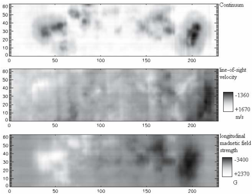
Figure 3. Example of the scan through AR NOAA 50 at July 31 2002 (09:49 UT): continuum near 6569 \text{ \AA} , photospheric line-of-sight velocity, longitudinal magnetic field strength. Positive and negative velocities correspond to the direction to and from the observer, respectively.
