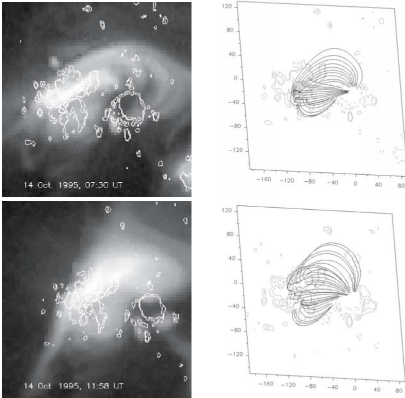
Figure 1. SXT images with longitudinal magnetograms overlaid (left) and coronal linear force-free model (right) of AR 7912. Iso-contours ( \pm 70 , \pm 140 G) have been drawn with cont./dashed lines for positive/negative magnetic field values (left).
