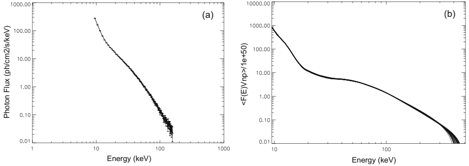
Figure 7. a) RHESSI photon spectrum of the February 26 ( \sim 10:26 UT), 2002 flare accumulated near the peak over 20 s interval with error bars. b) The resulting electron spectrum obtained inverting the photon spectrum using first order regularization algorithm (Kontar et al. , 2004). The multiple lines present various realizations of the regularized solution within the errors of the photon spectrum.
