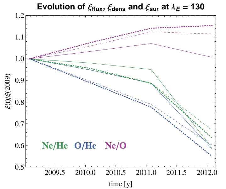
Fig. 15. Relative change of the \xi quotients for the season-integrated flux (solid lines), densities at the ecliptic longitude where the NIS gas flow intersects the Earth’s orbit (broken lines) and time-dependent survival probabilities of the NIS atoms reaching IBEX at this location (dotted lines). All quantities are shown as ratios to the respective values in 2009. The color code for species pairs is indicated in the panel.
