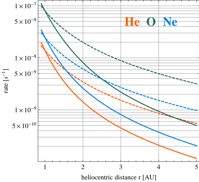
Fig. 2. Comparison of the radial dependence of electron impact ionization adopted in this paper with the 1/r^2 -dependence for He, Ne, and O. Solid lines indicate the radial profiles calculated using \beta_{\text{el}}^{\text{slow}}(r) from Eq. (A.9), broken lines are for electron ionization calculated from \beta_{\text{el}}^{\text{slow}}(r = 1\text{AU})/r^2 , both for solar wind proton density at 1 AU n_{\text{sw}}(r = 1\text{AU}) = 6.14 \text{ cm}^{-3} , assuming the decrease of proton density like 1/r^2 .
