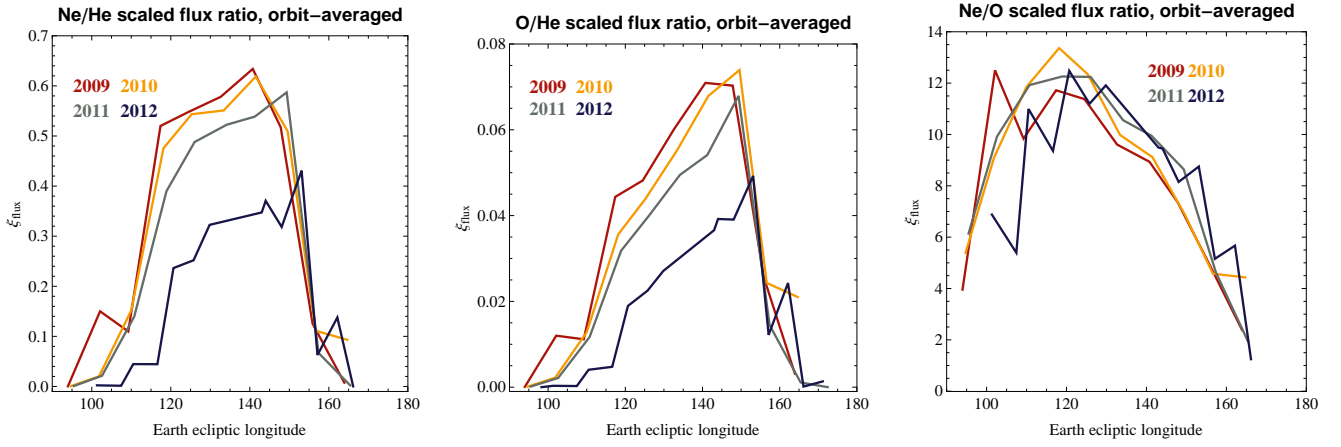
Fig. 14. Flux abundance quotients \xi_{\text{flux},X/Y} for the Ne/He, O/He, and Ne/O pairs calculated from the scaled fluxes integrated over IBEX spin phase and averaged over the orbits for the first four years of IBEX observations.
