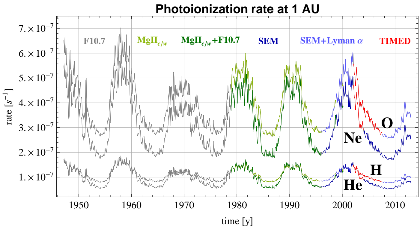
Fig. A.1. Time series of Carrington period-averaged photoionization rates of H, He, Ne, and O at 1 AU from the Sun. The color code denotes the various sources of data and proxies used, as discussed in the text.
