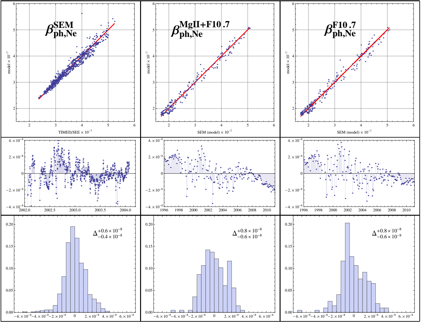
Fig. A.4. Scatter plot of model vs data for photoionization models for Ne defined in Eq. (A.2) (left column), Eq. (A.3) (middle column) and Eq. (A.4) (right column), fit residuals (middle row), and histograms of the residuals (lower row). The red y = x lines are eye guides. The statistical uncertainties of the models are indicated in the insets in the histogram panels.
