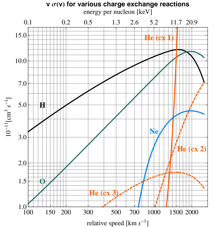
Fig. A.7. Products of relative speeds of reaction components and charge exchange cross sections for these speeds for the charge exchange reactions listed in the text (see Section 2.2). To obtain the actual charge-exchange rate, one has to multiply a quantity read off from the figure for a given speed by the local density of the ionized reaction component (solar wind proton, alpha particle). The lower horizontal axis is scaled in \text{km s}^{-1} , the upper axis in energy per nucleon in keV.
