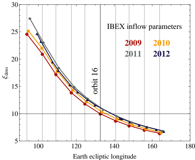
Article number, page 14 of 25 Fig. 11. Heliospheric abundance quotients calculated from the relative densities shown in Fig. 9 using Eq. (32) for the times and locations as for Fig. 9.
