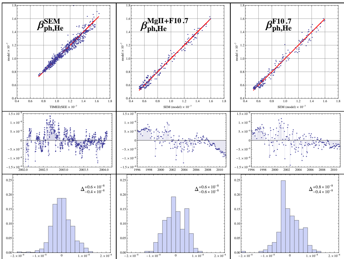
Fig. A.3. Scatter plot of model vs data for photoionization models for He defined in Eq. (A.2) (left column), Eq. (A.3) (middle column) and Eq. (A.4) (right column), fit residuals (middle row), and histograms of the residuals (lower row). The red y = x lines are eye guides. The statistical uncertainties of the models are indicated in insets in the histogram panels.
