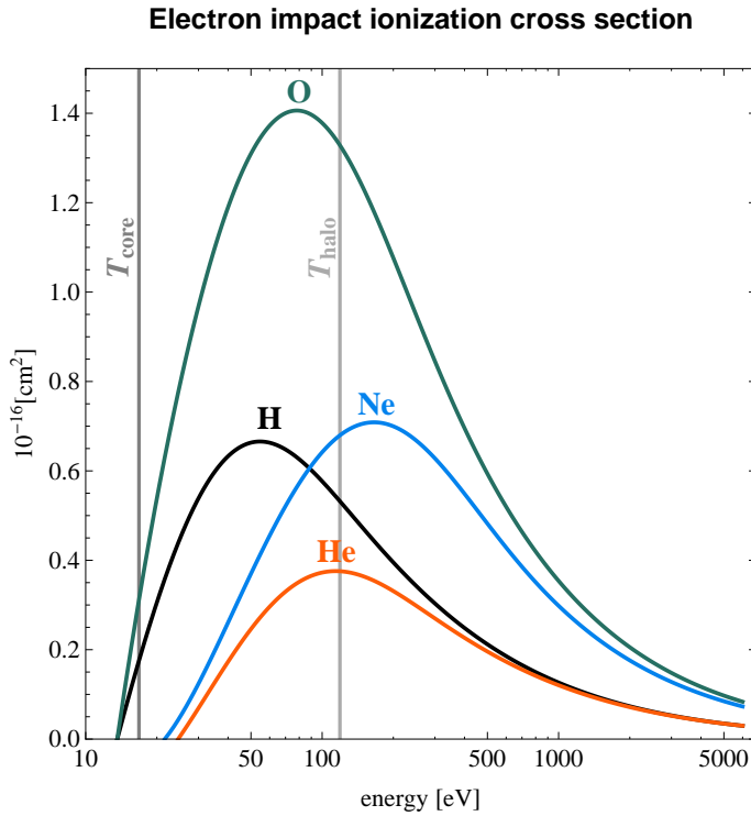
Fig. A.6. Cross sections of electron impact ionization for H, He, Ne, and O (Lotz 1967). The accuracies for H, He, and O are 10%, for Ne 15%. The vertical bars mark the energies corresponding to the temperatures of the core and halo solar wind electron populations in the slow solar wind at 1 AU from the Sun. Note that the noble gases can only be ionized by a high-energy wing of the core population and mostly by the halo population.
