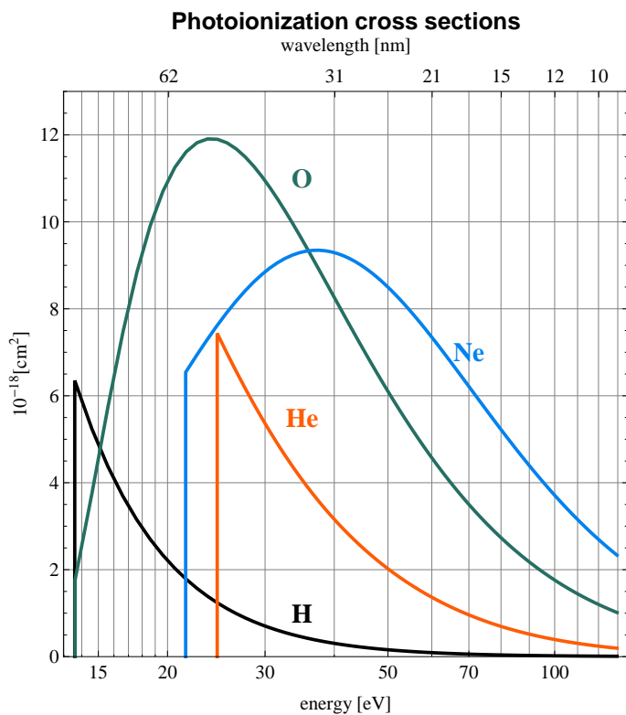
Fig. A.2. Cross sections for photoionization of neutral H, He, Ne, and O used in the calculations (Verner et al. 1996). The accuracy is at a \sim 5\% level. Note that even though the ionization threshold energy for O and H are very similar, the cross section values for the low energy portion, where the solar spectral flux is greatest, are substantially different.
