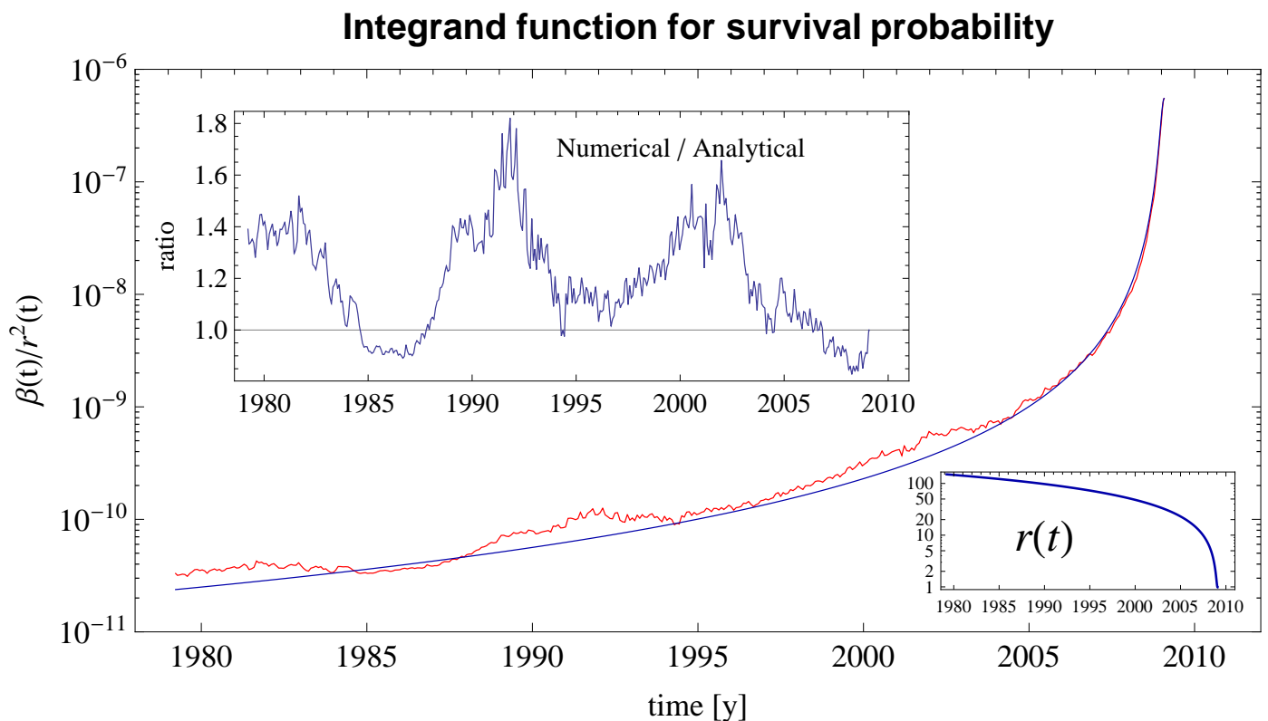
Fig. 3. Integrand function in Eq. (3) for an O atom on the orbit whose perihelion is at the Earth location on IBEX Orbit 16 in 2009 ( \lambda_E = 130^\circ ). The red line is the \beta(\mathbf{r}(t), \mathbf{v}, t) from Eq. (1) taken along the orbit of the atom. The model used in \beta(\mathbf{r}(t), t) is time dependent and has a component of electron impact rate, which does not follow the 1/r^2 dependence. The dark-blue line is the integrand function calculated for \beta(r_E, t_0) \left(\frac{r_0}{r(t)}\right)^2 , i.e. assuming that the ionization rate is equal to the ionization rate from our model calculated for the instant of detection t_0 . The history of the radial distance of the atom from the Sun is shown in the lower-right inset and it is identical for the red and dark-blue lines. The upper-left inset presents the ratio of the actual ionization rate for atoms following the aforementioned trajectory and the rate used in the analytical model \beta_0(t_0) (r_0/r)^2 . To obtain the survival probability one must calculate the exponent of the time integral of the function drawn in red, see Eqs. (2) and (3). The analytic approximation is equivalent to taking exponent of the integral of the function drawn with the blue line, i.e. to evaluating the exponent of the expression from Eqs. (2) and (4).
