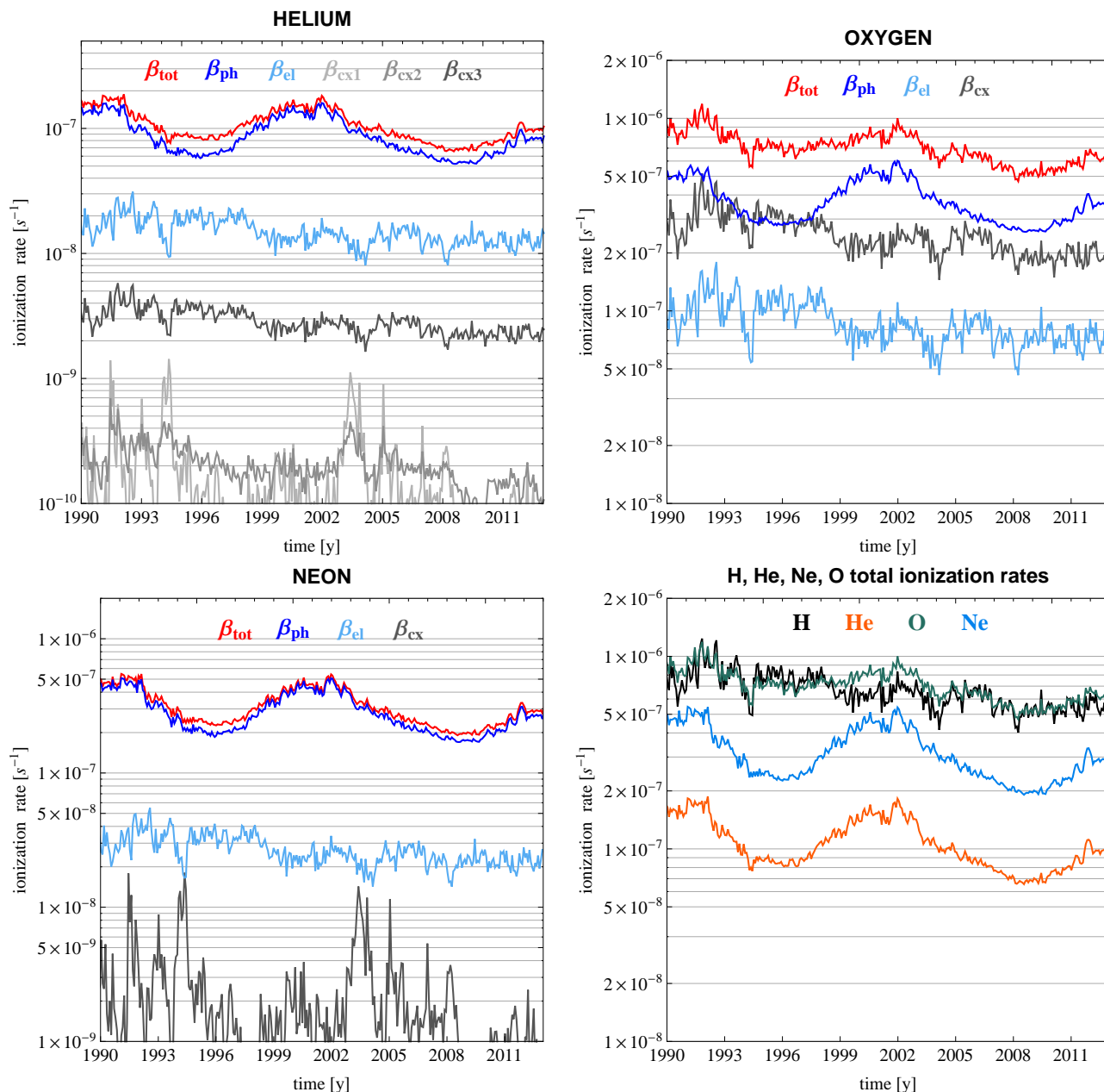
Fig. 1. Time series of ionization rates of neutral He, Ne, and O used in this study. Shown are total ionization rates at 1 AU from the Sun as well as photoionization, electron-impact, and charge exchange rates for all relevant reactions. The lower-right panels show the total ionization rates of He, Ne, and O in a common scale. For comparison, the ionization rate of H (Bzowski et al. 2013) is added.
