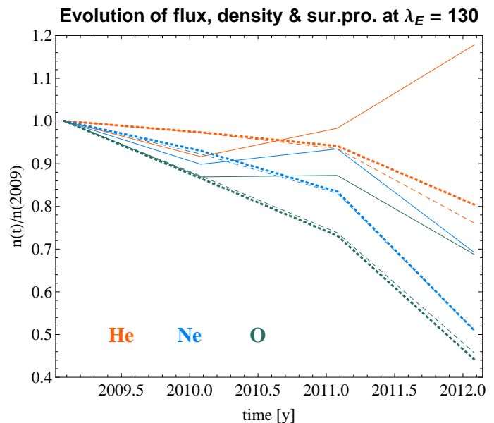
Fig. 10. Relative change of the season-integrated flux (solid lines), density at the ecliptic longitude where the NIS gas flow intersects the Earth's orbit (broken lines) and time-dependent survival probabilities of the NIS atoms reaching IBEX at this location (dotted lines). All quantities are shown as ratios to the respective values in 2009. The relative change of the flux is equivalent to the change of total counts per orbit. The color code for species is indicated in the panel.
