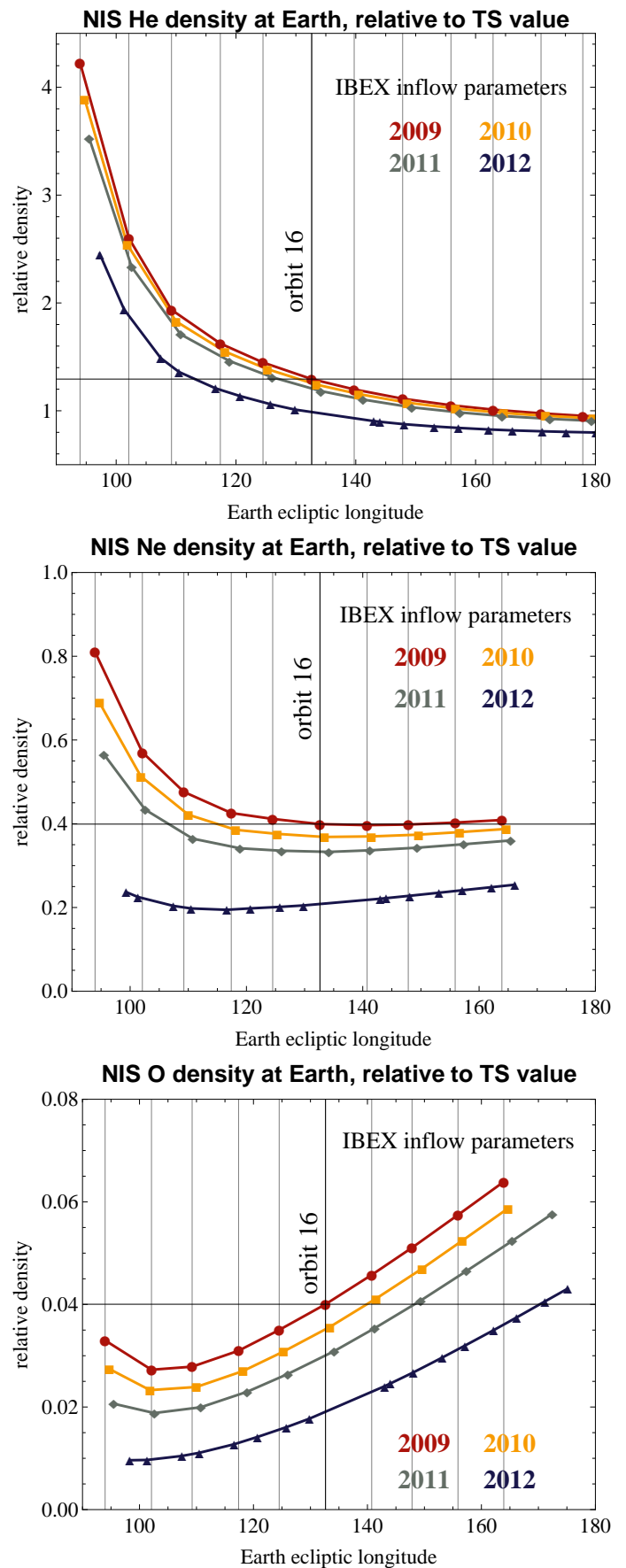
Fig. 9. Relative densities (scaled to the values at TS, Eq. (32)) for NIS He, Ne, and O for the four IBEX sampling seasons, calculated for the apogee times of IBEX orbits for the inflow parameters obtained by Bzowski et al. (2012) from IBEX NIS He observations. The vertical bars mark the longitudes of IBEX apogees in 2009, the horizontal bars marks the relative density levels for this time and location in space.
