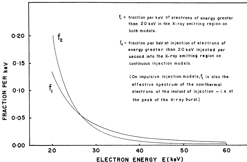
Fig. 1. Effective differential energy spectra of energetic electrons ( > 20 keV) required to produce a hard X-ray burst with power law X-ray spectrum \sim \varepsilon^{-4} (at photon energies \varepsilon > 20 keV) at the burst peak.
