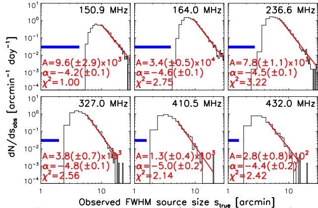
Fig. 2.— Histogram of the radio sources' rms FWHM s = s_{rms,obs} , at different frequencies. The red curves are fittings \frac{dN}{ds} = A s^\alpha to the histograms, from the bin to the immediate right of the peak in the histogram and above. The blue bar delimits the minimum NRH point spread function (which can vary by almost a factor 2, depending on the season and time of day).
