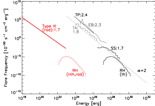
Fig. 16.— Black/gray : Approximate flare heating input to the solar corona as derived from various EUV/X-ray nanoflare and microflare studies: RH : RHESSI , Hannah et al. (2008); SS : Yohkoh SXT, Shimizu (1995); TA : TRACE , Aschwanden et al. (2000); TP : TRACE , Parnell & Jupp (2000); EB : SOHO EIT , Benz & Krucker (2002) (after Hannah et al. 2008). Red lines : Radiated energies. The dotted red line corresponds to the radiated energy in non-thermal HXR that roughly accompanied the RHESSI -derived flare input, using an approximated nonthermal bremsstrahlung efficiency of 10^{-5} . The solid red line is the radiated energy derived from this Type III study.
