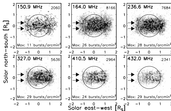
Fig. 5.— Occurrence density distributions for the radio bursts in Section 2, on a 1' pixel grid. The number in upper right corner is the total number of events with reliable positions. The intensity scale is linear from white to black, with black representing the maximum pixel value as specified in each plot. The arrows indicate the \pm 15 degrees heliographic latitudes.
