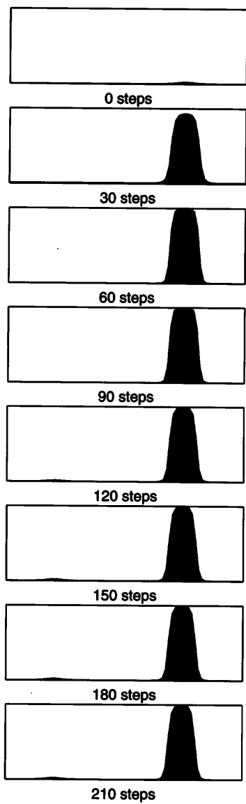
Figure A.3 Simulation of an attractor network unaffected by offset input. A small excitation is input far from the center of the bump. (Compare figure A.4.) Similar simulations have been reported by Redish (1997).
